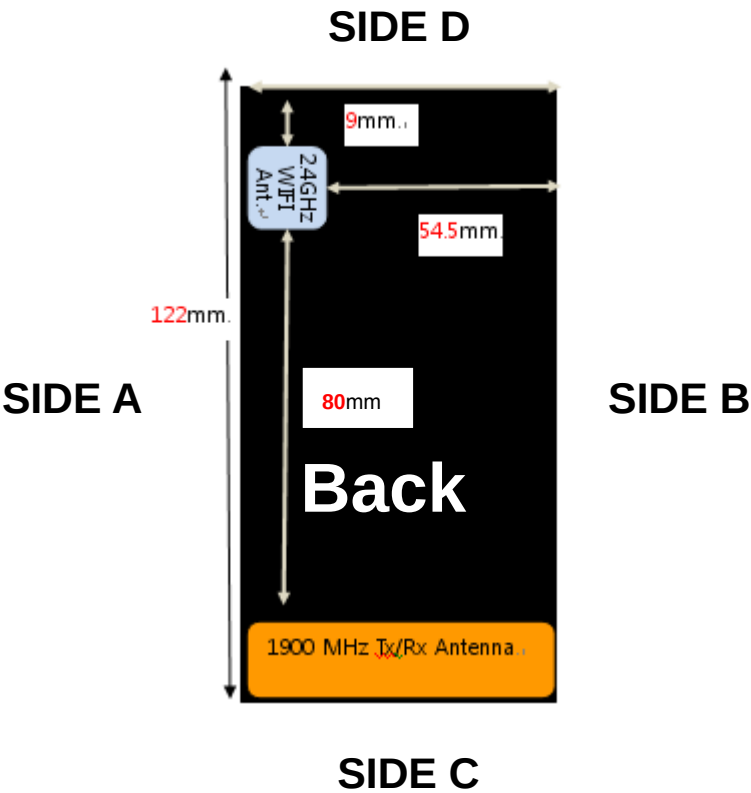
Figure 5.7 Antenna Locations, as viewed from back of device
