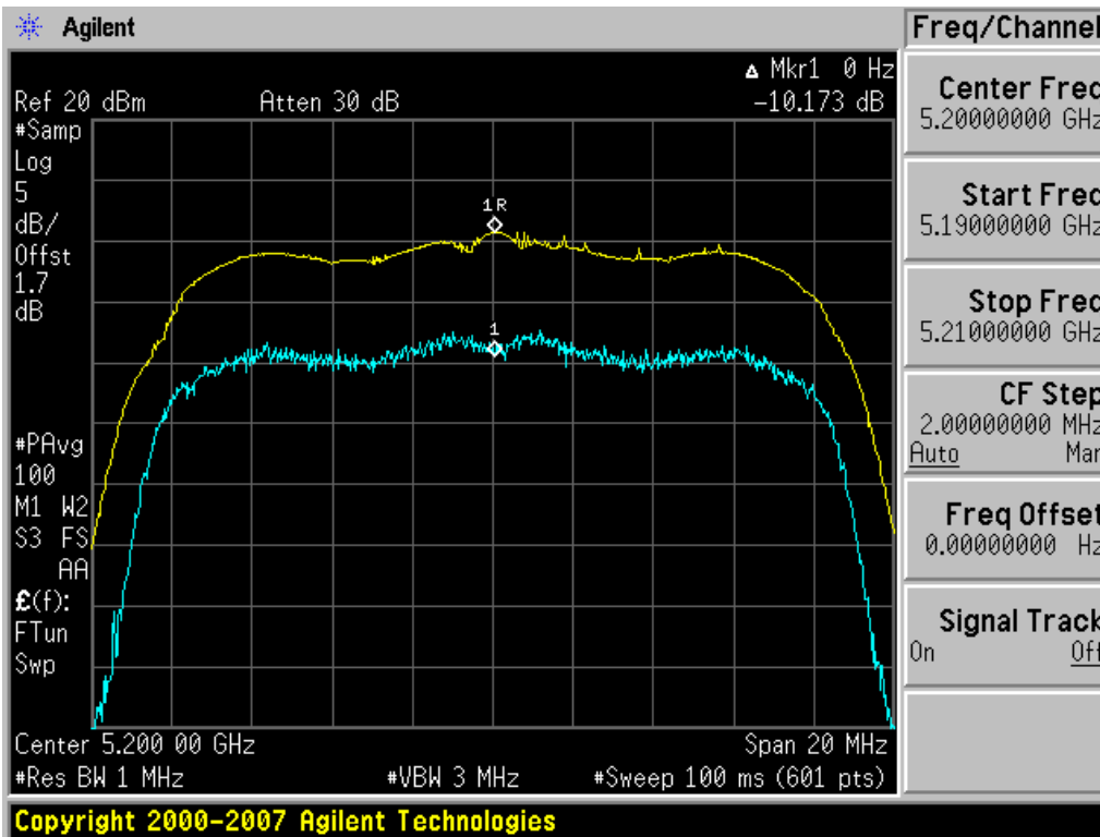
Plot 6-38. Peak Excursion Ratio Plot (802.11a (UNII Band 1) – Ch. 40)
