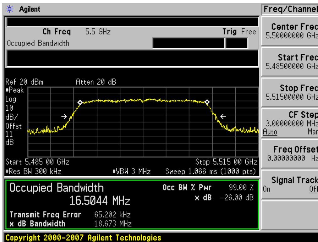
Plot 6-13. 26dB Bandwidth Plot (802.11a (UNII Band 3) – Ch. 100)
