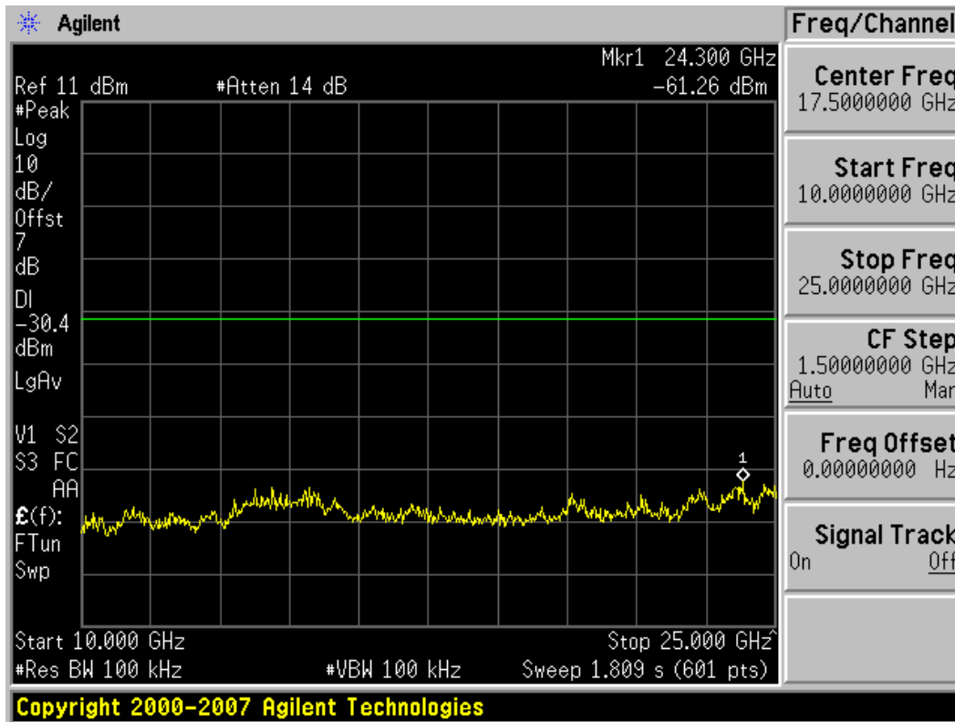
Plot 6-54. Conducted Spurious Plot (802.11a – Ch. 165)
