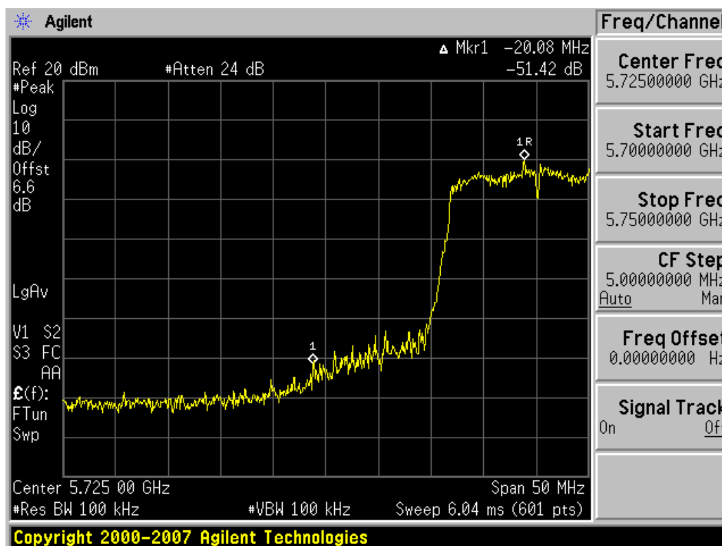
Plot 6-37. Band Edge Plot (802.11a – Ch. 149)
