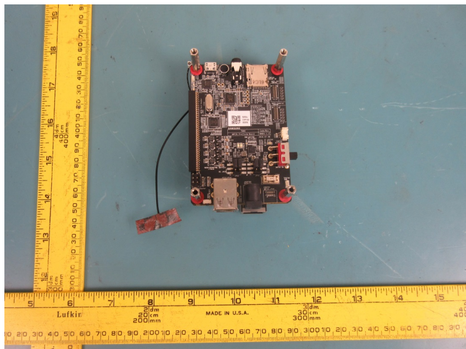
EUT with support board – Bottom View
