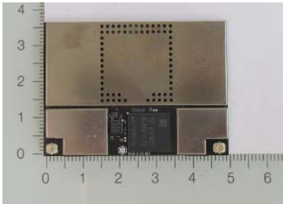
EUT – Module Shielded Top View
