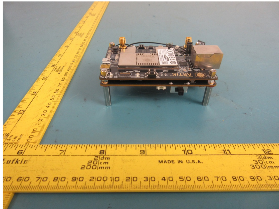
EUT with support board – Left View
