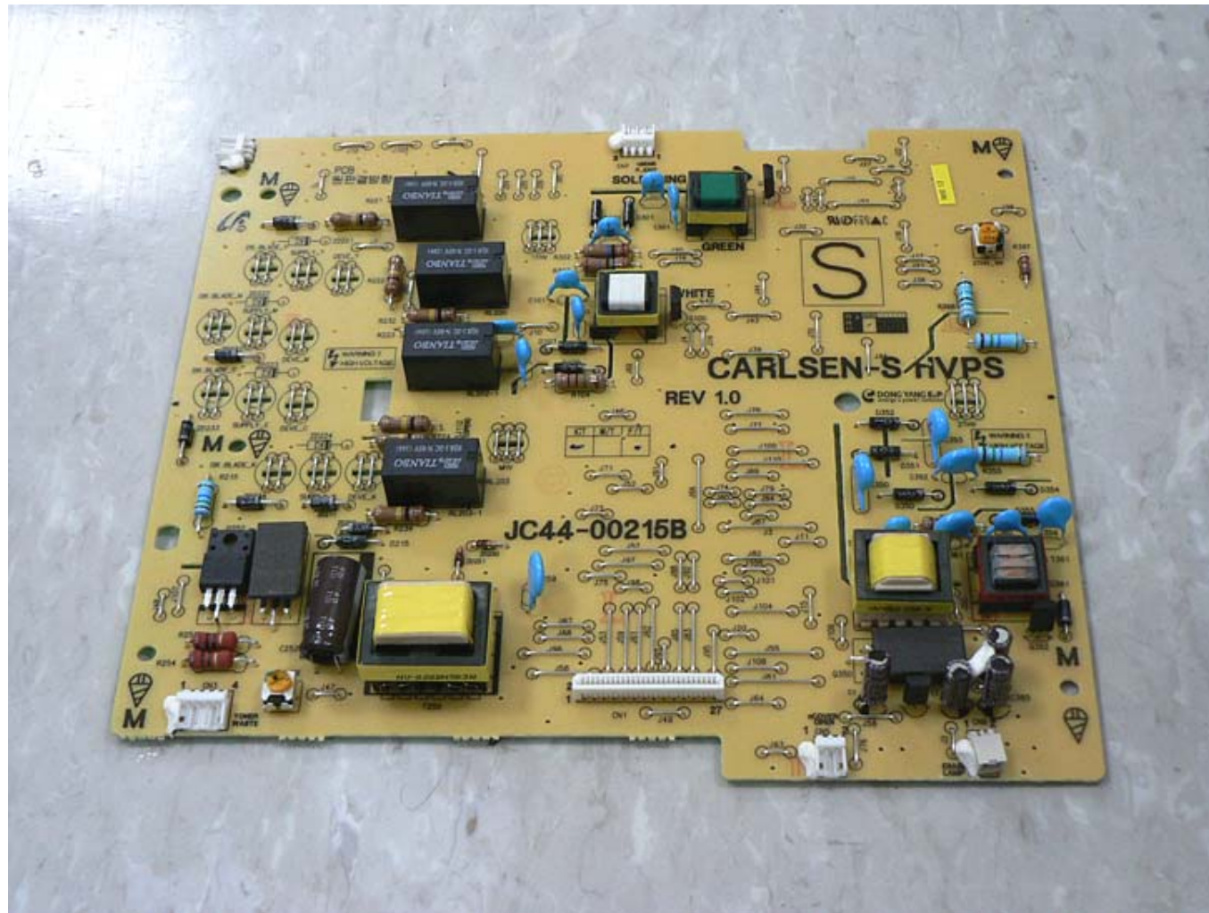
DONGYANG HVPS Xpress C430W_HVPS PBA_Top side
