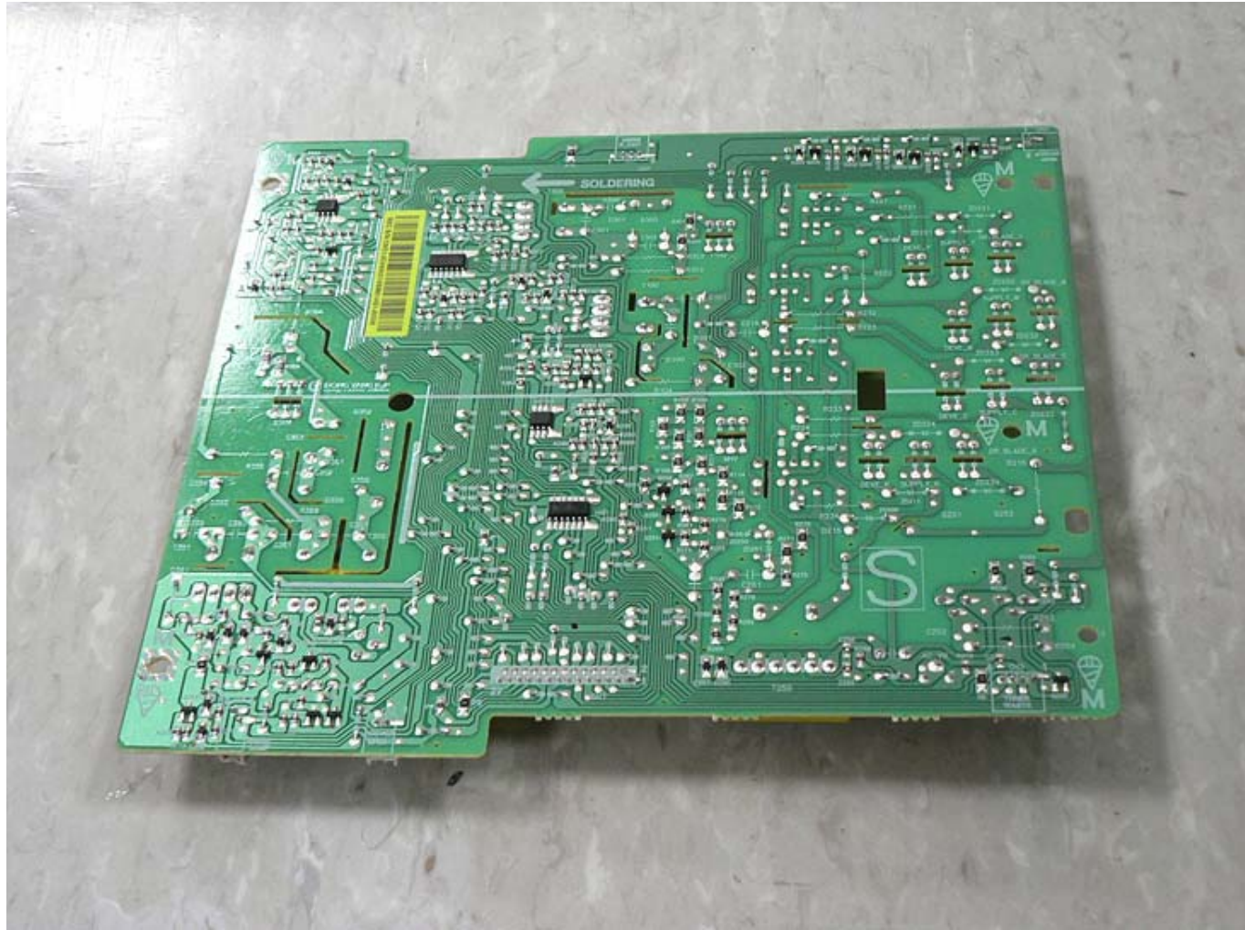
DONGYANG HVPS Xpress C430W_HVPS PBA_Bottom side
