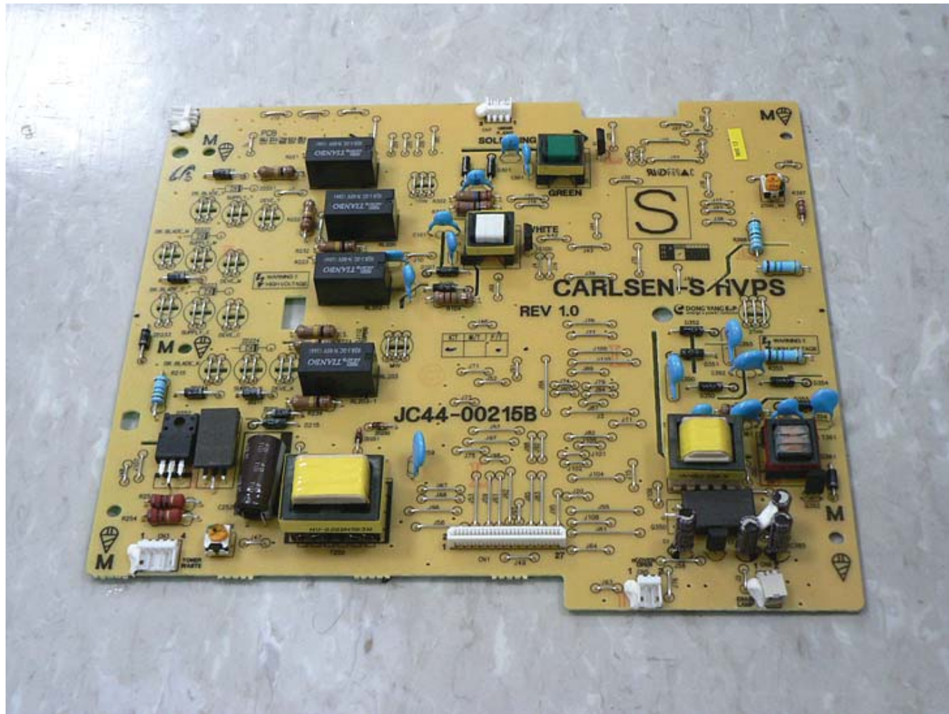
DONGYANG HVPS Xpress C480FW_HVPS PBA_Top side
