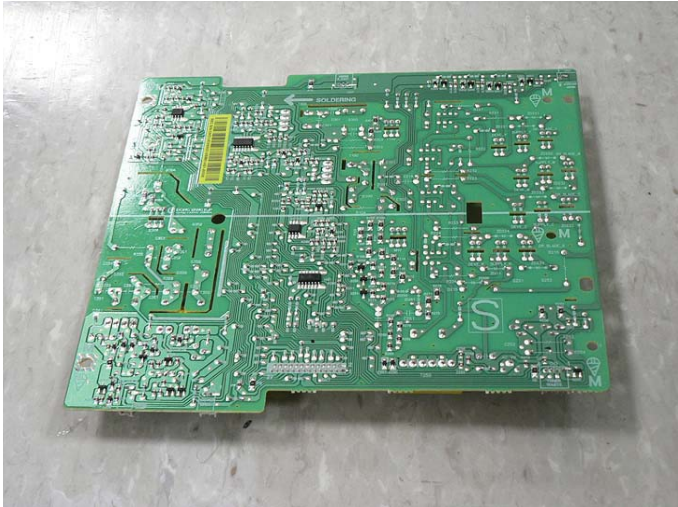
DONGYANG HVPS Xpress C480FW_HVPS PBA_Bottom side
