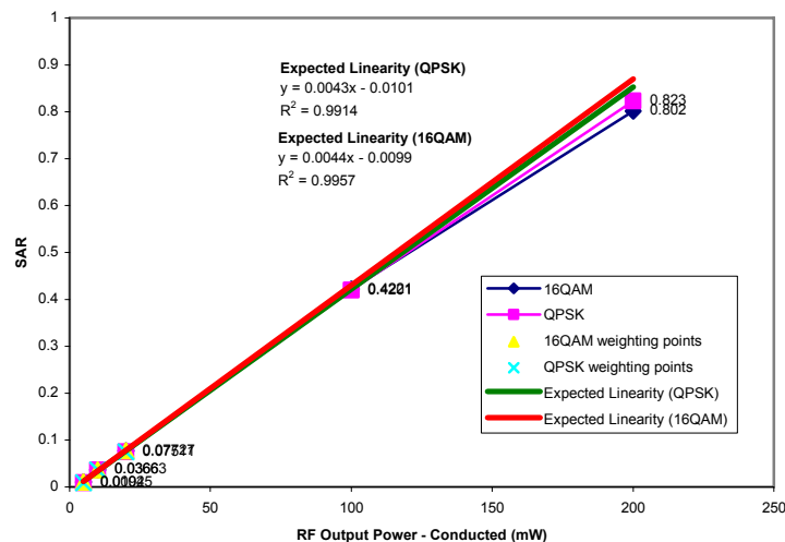
Linearity of SAR Probe Used for FCC ID: A3LSLCU100
