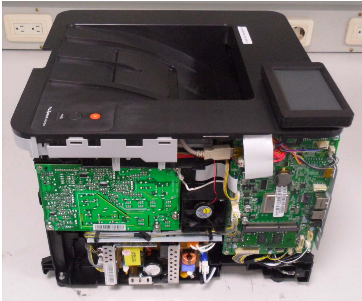
ProXpresss M4020NX Internal_Right
