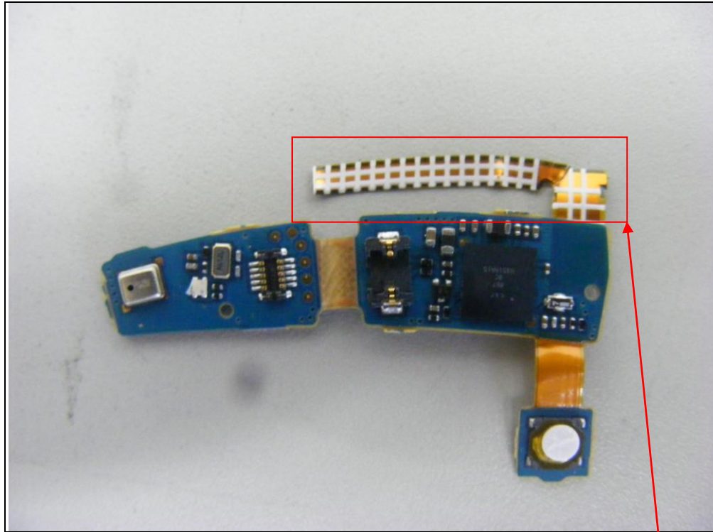
BT Antenna
