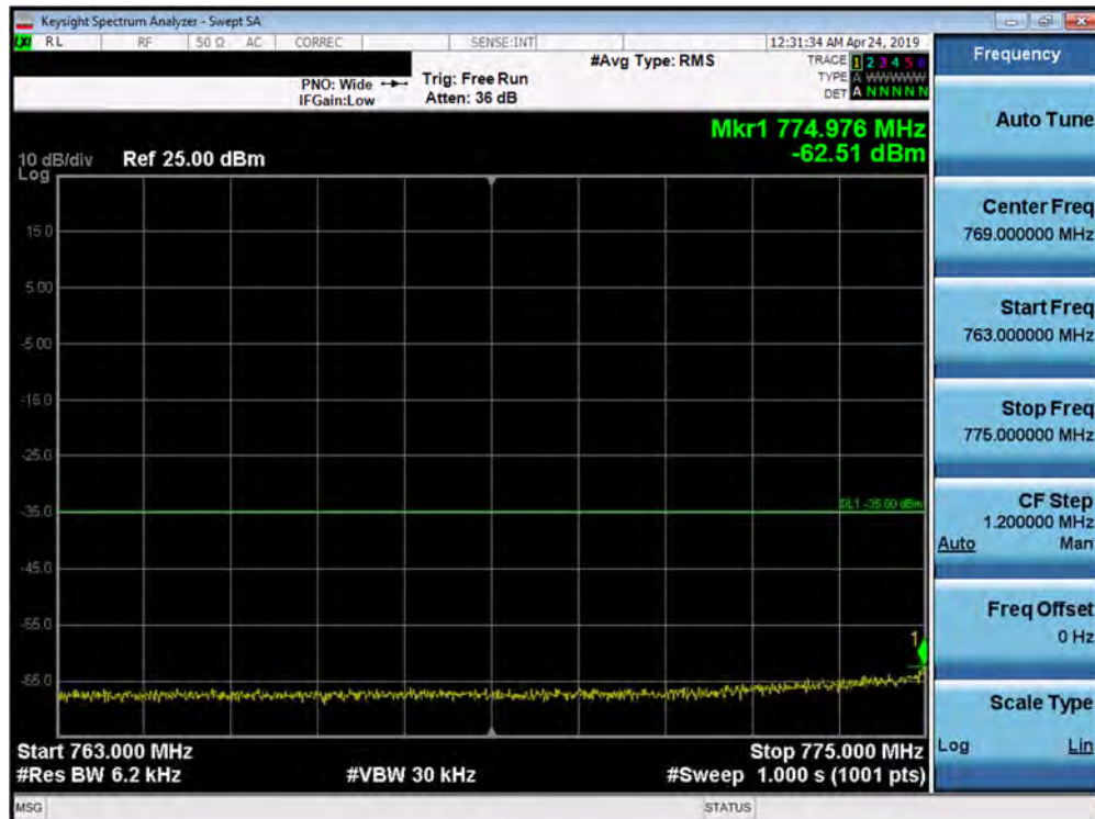
Plot 7-221. Lower Emission Mask Plot (Band 13 - 5.0MHz QPSK - Full RB Configuration)
