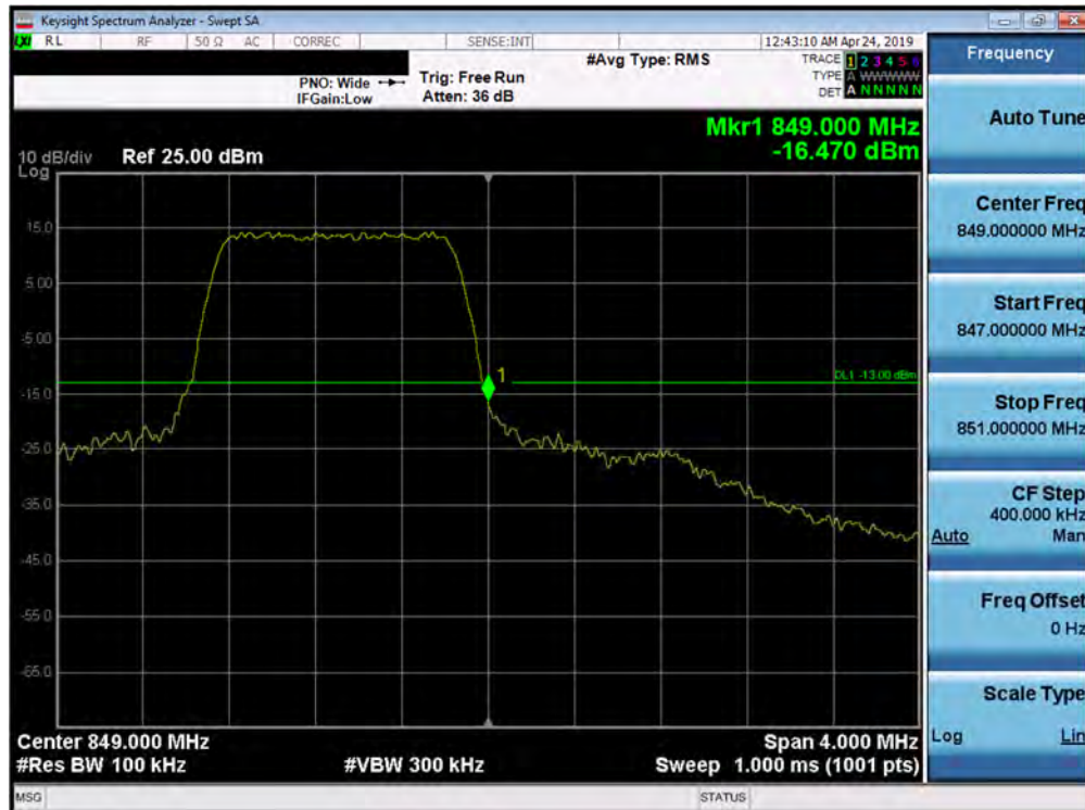
Plot 7-229. Upper Band Edge Plot (Band 26/5 - 1.4MHz QPSK - Full RB Configuration)
