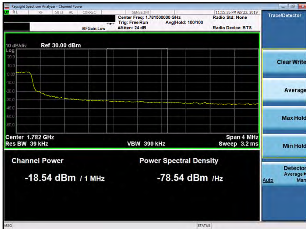
Plot 7-255. Upper Extended Band Edge Plot (Band 66 - 5.0MHz QPSK - Full RB Configuration)
