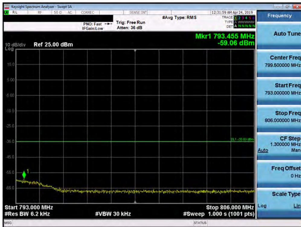
Plot 7-223. Upper Emission Mask Plot (Band 13 - 5.0MHz QPSK - Full RB Configuration)
