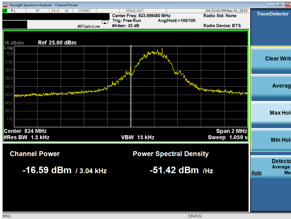
Plot 7-70. Band Edge Plot (Cellular GSM Mode - Low Channel)
