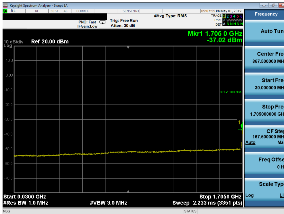
Plot 7-52. Conducted Spurious Plot (AWS WCDMA Mode - Low Channel)
