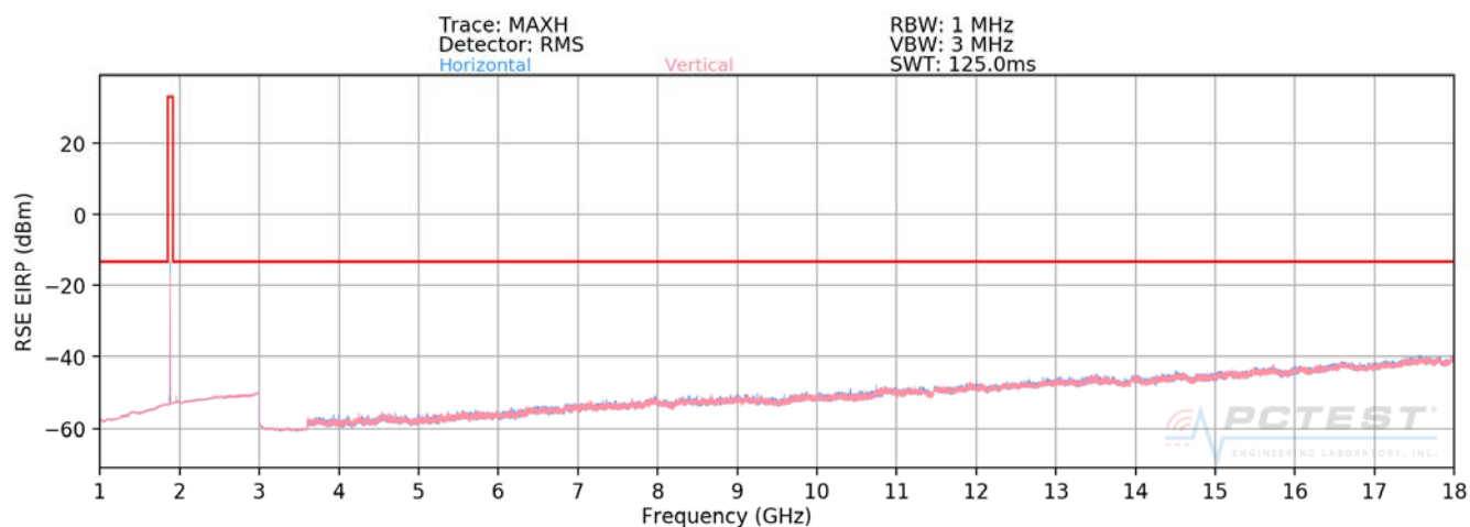
Plot 7-105. Radiated Spurious Plot above 1GHz (PCS WCDMA Mode)
