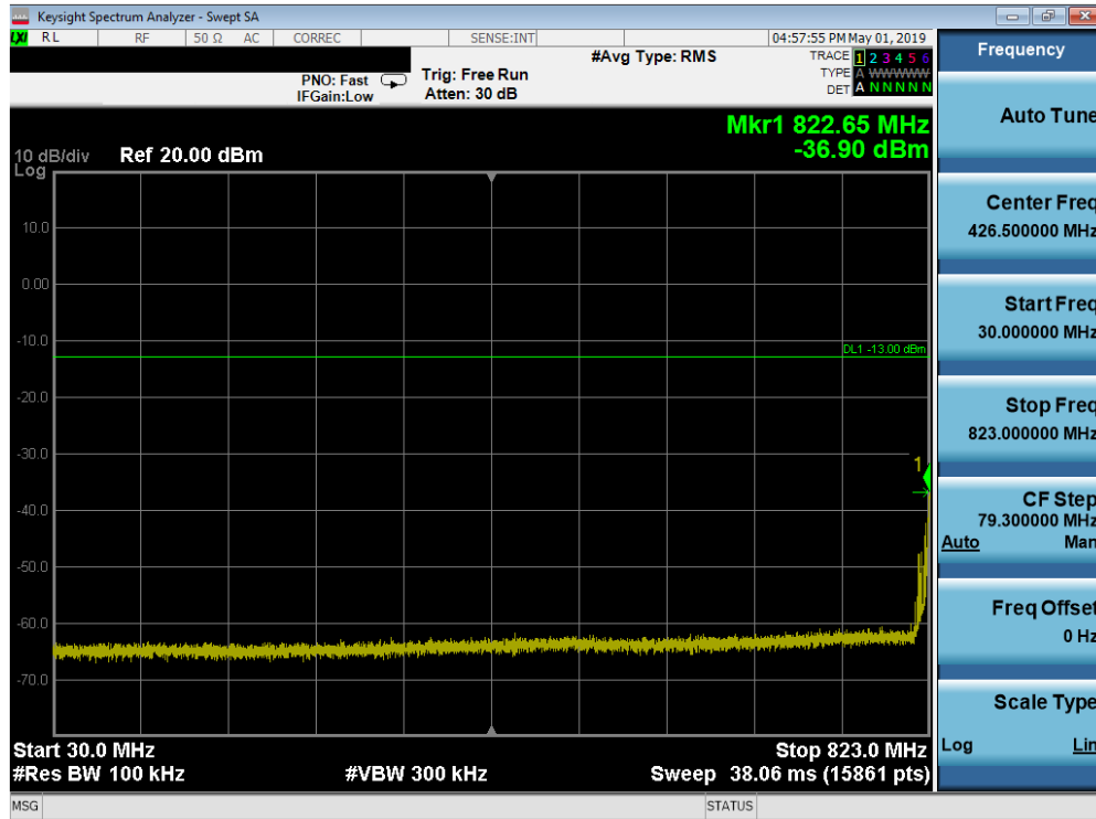
Plot 7-43. Conducted Spurious Plot (Cellular WCDMA Mode - Low Channel)
