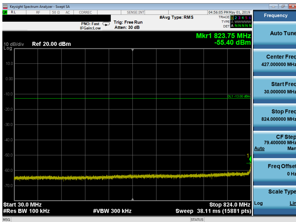
Plot 7-46. Conducted Spurious Plot (Cellular WCDMA Mode - Mid Channel)
