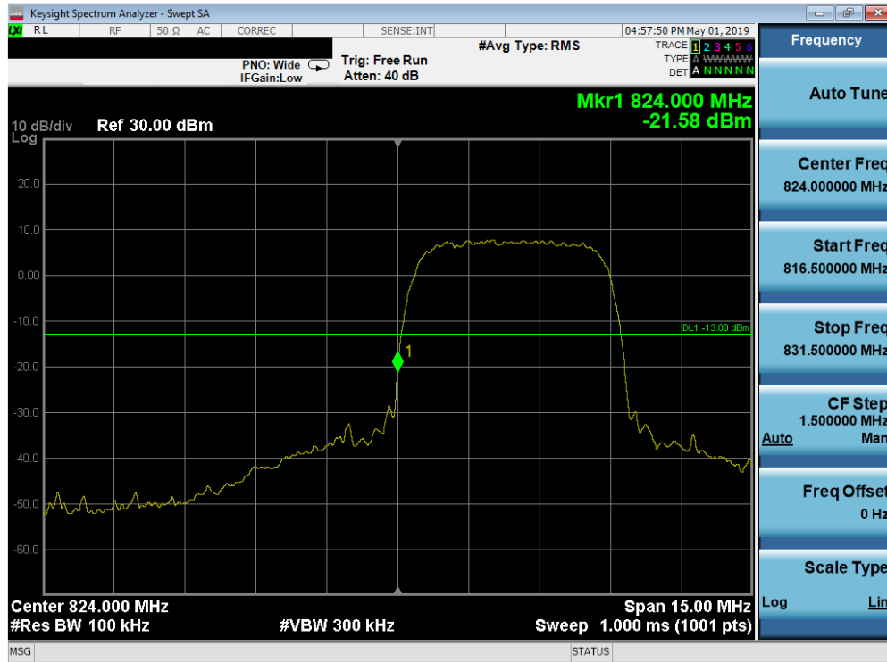
Plot 7-84. Band Edge Plot (Cellular WCDMA Mode - Low Channel)
