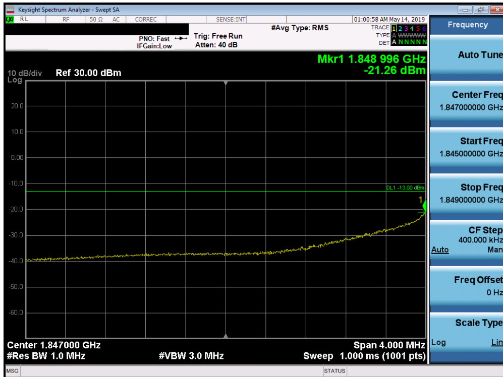
Plot 7-81. 4MHz Span Plot (PCS CDMA Mode - Low Channel)
