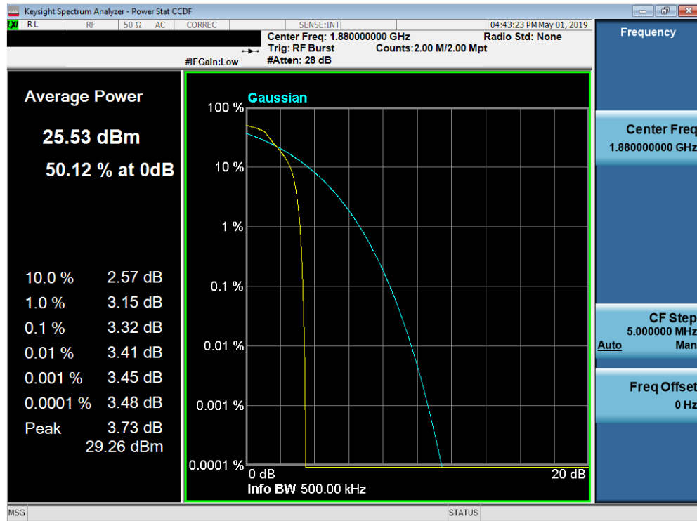
Plot 7-95. Peak-Average Ratio Plot (PCS EDGE Mode)
