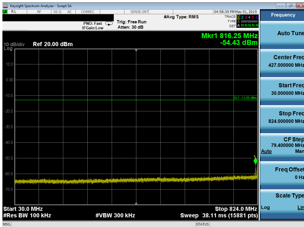
Plot 7-49. Conducted Spurious Plot (Cellular WCDMA Mode - High Channel)
