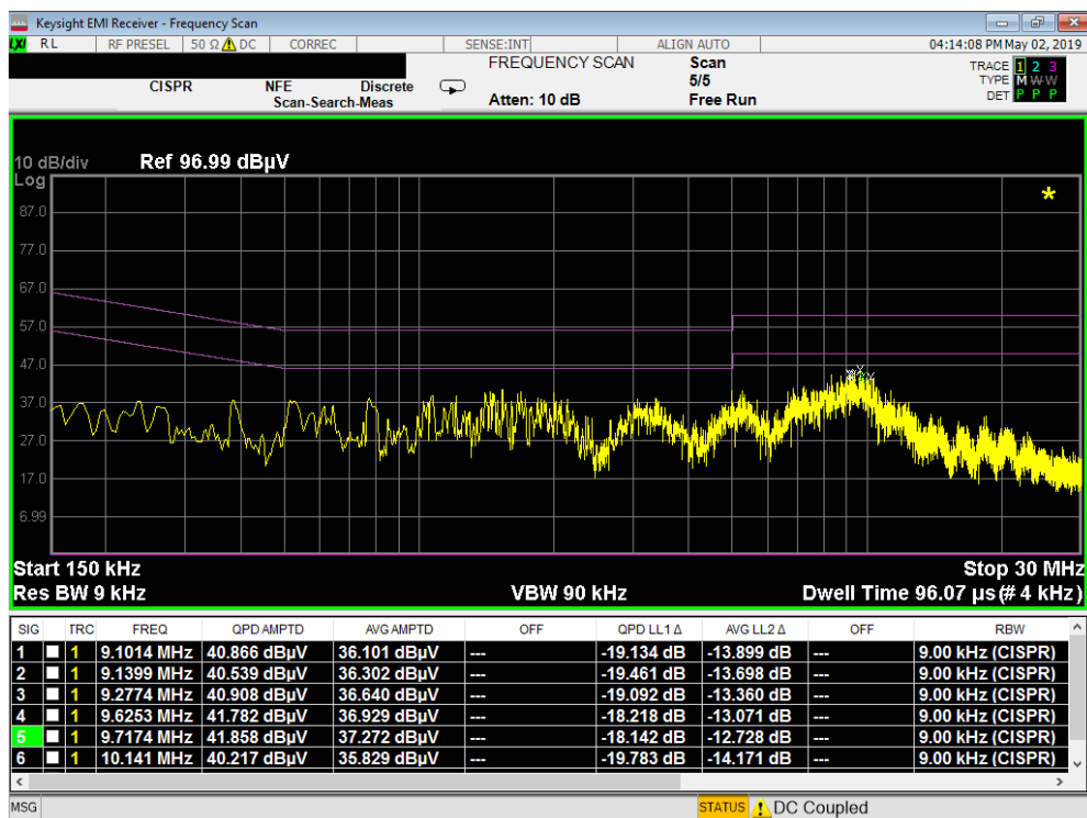
Plot 7-55. Line Conducted Plot with 802.11b (N)
