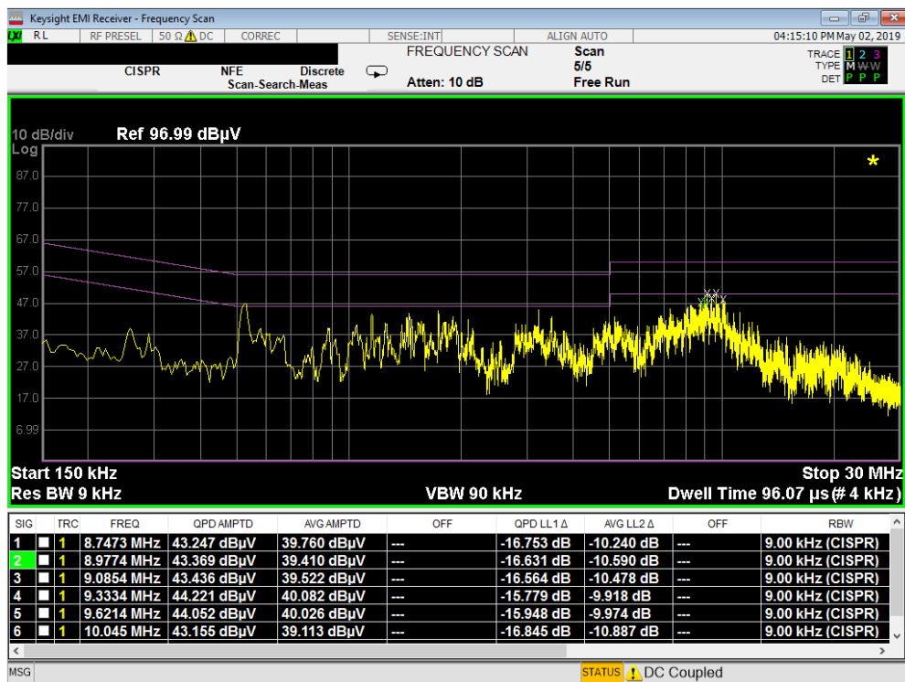
Plot 7-54. Line Conducted Plot with 802.11b (L1)
