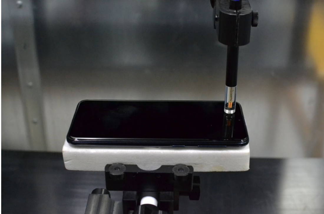
Figure 16-1 Test Setup for Wireless Device
