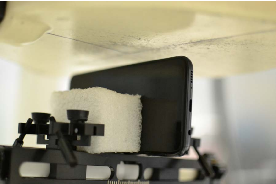
SAR Test Setup Photo 10 – Right Side at 10 mm
