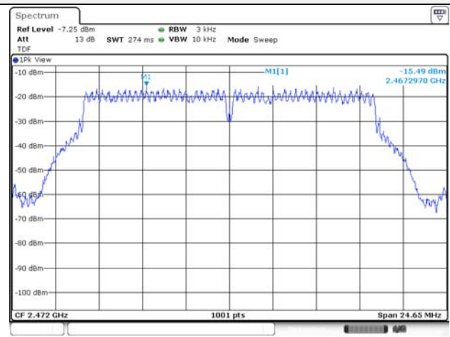
802.11g / 2 472 MHz
