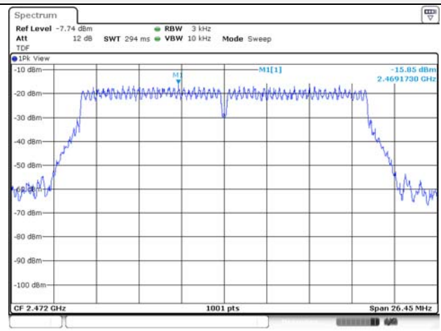
802.11n HT20 / 2 472 MHz
