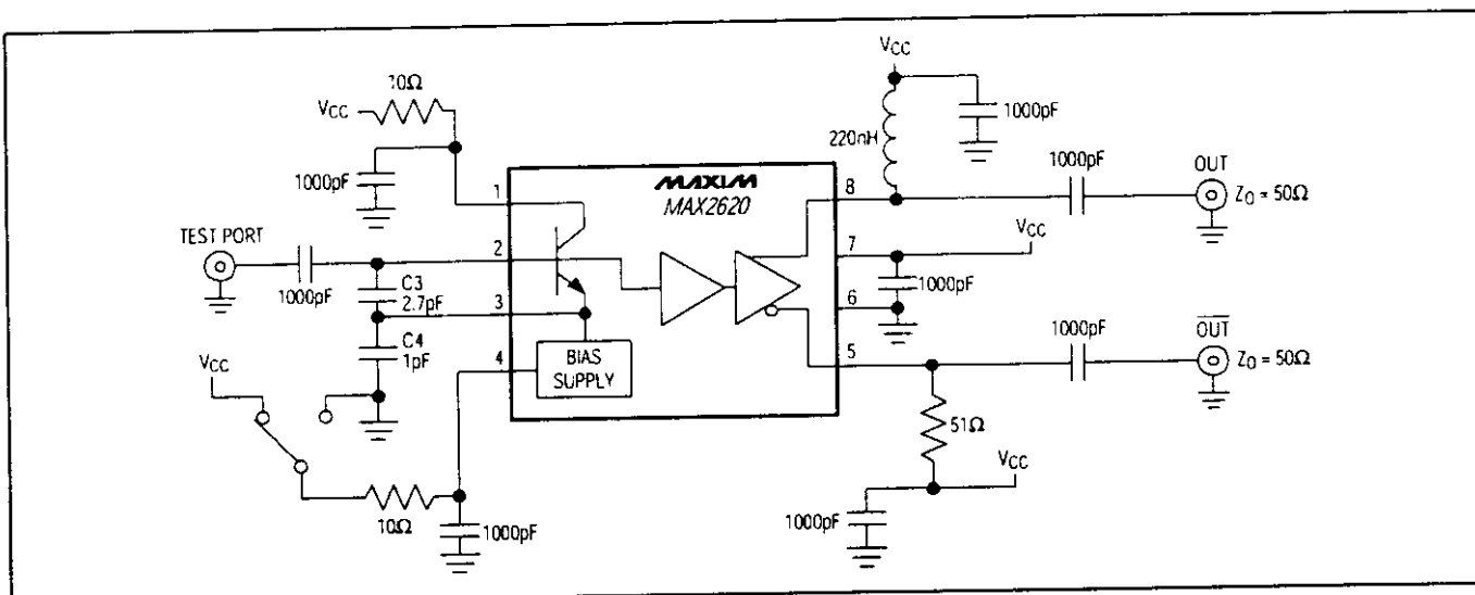
Figure 1. Test Circuit
