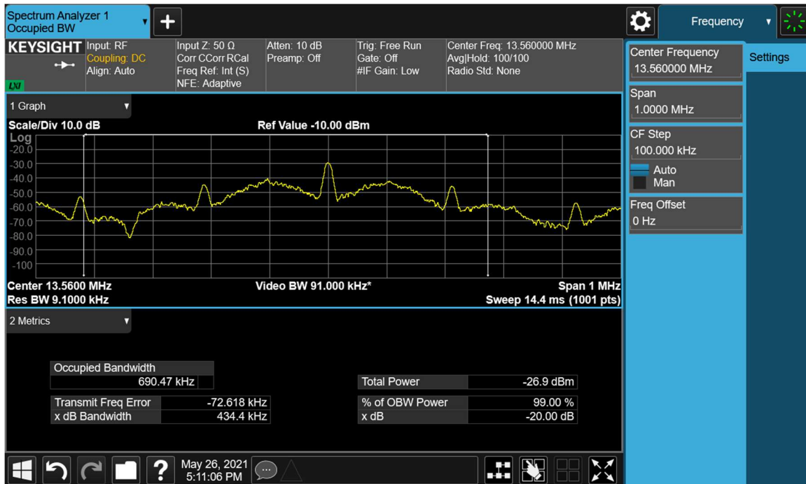
Figure 7-2. Occupied Bandwidth Plot
