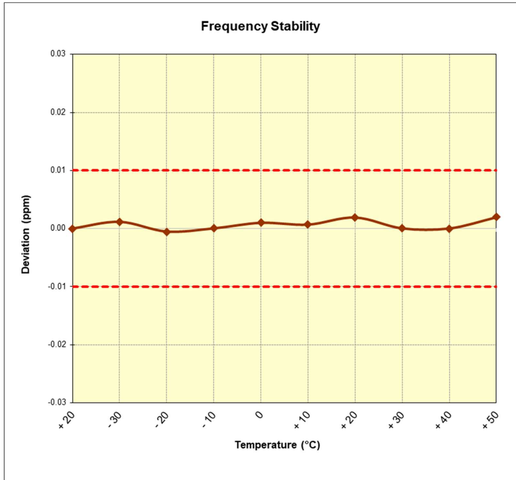
Figure 7-3. Frequency Stability Plot
