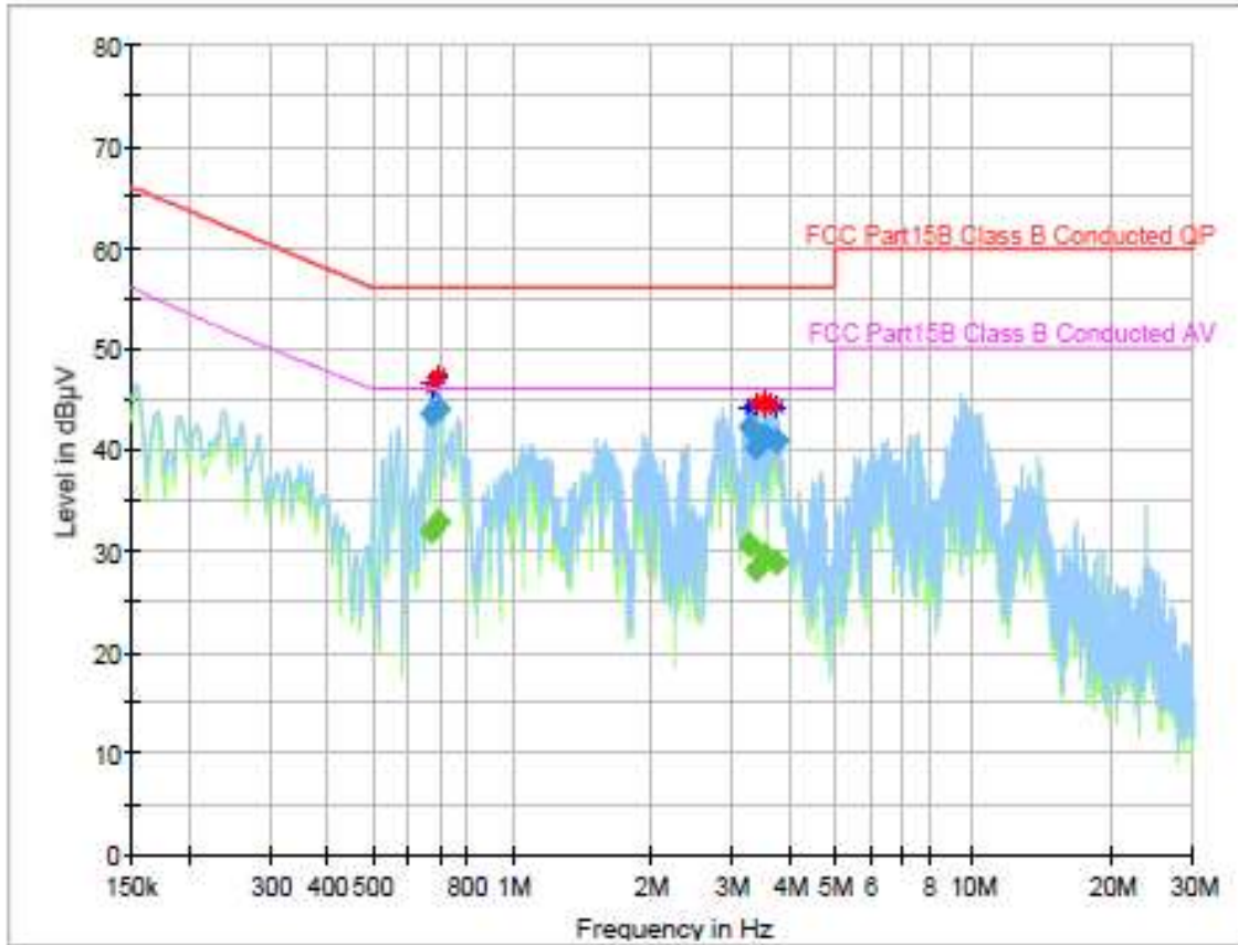
Plot 7-15. Line Conducted Plot (L1)
