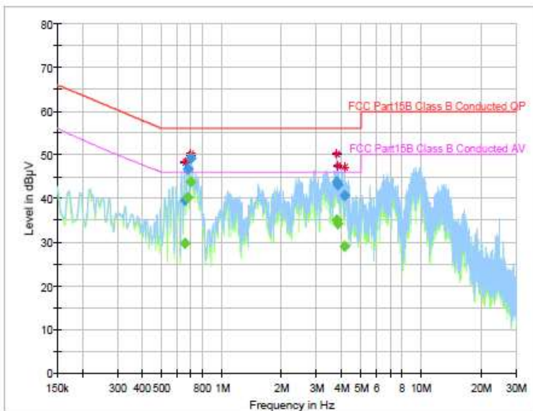
Plot 7-16. Line Conducted Plot (N)
