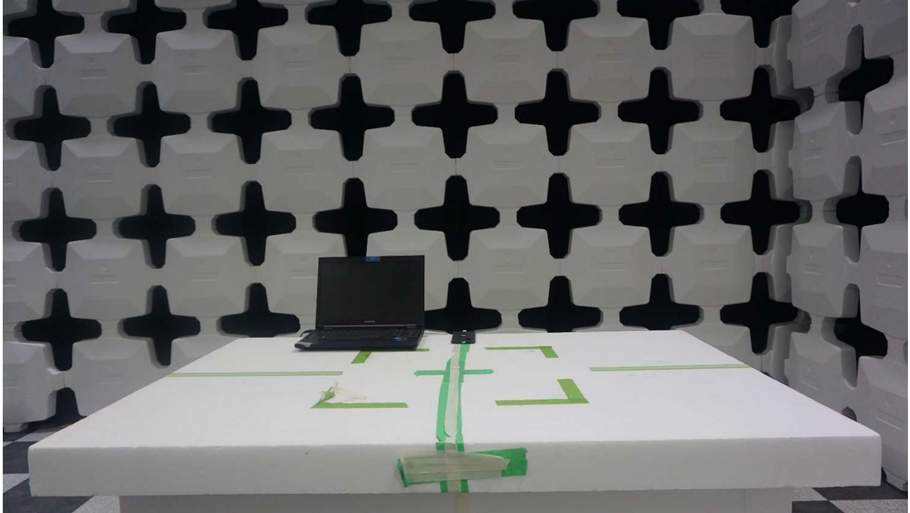
Radiated Test Configuration 2: USB Data Communication with PC (from external memory data)
