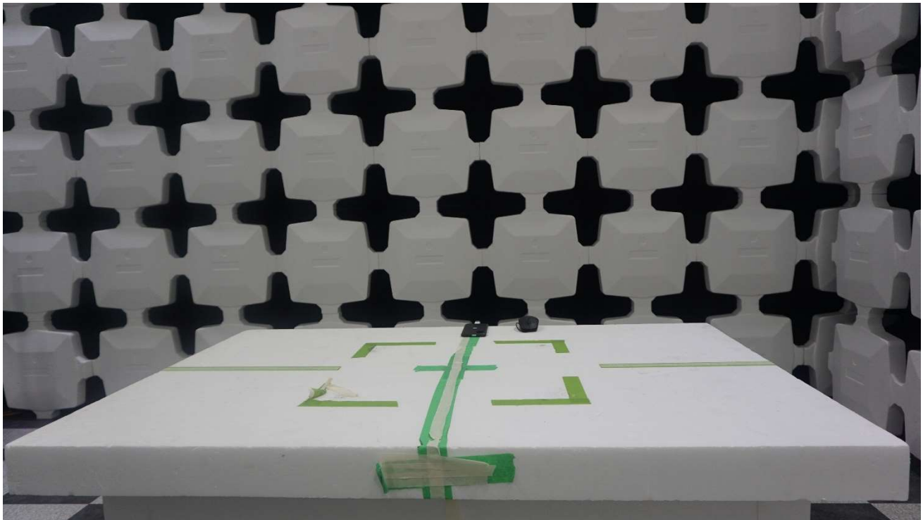
Radiated Test Configuration 3: Camera on (front) + USB OTG (with USB gender: mouse or keyboard)
