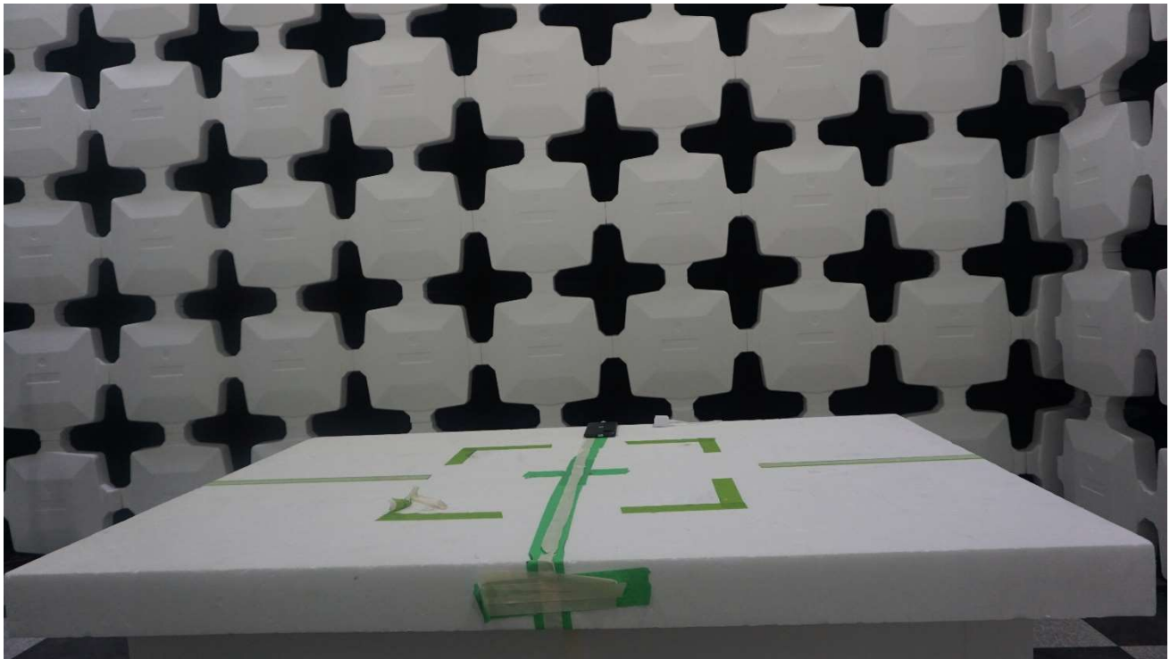
Radiated Test Configuration 1: Camera on (rear) + Charging (with travel adapter)
