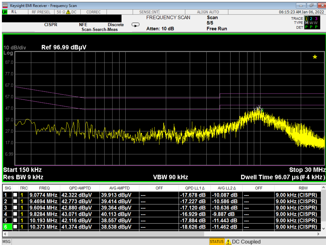
Plot 7-49. Line-Conducted Test Plot (N)
