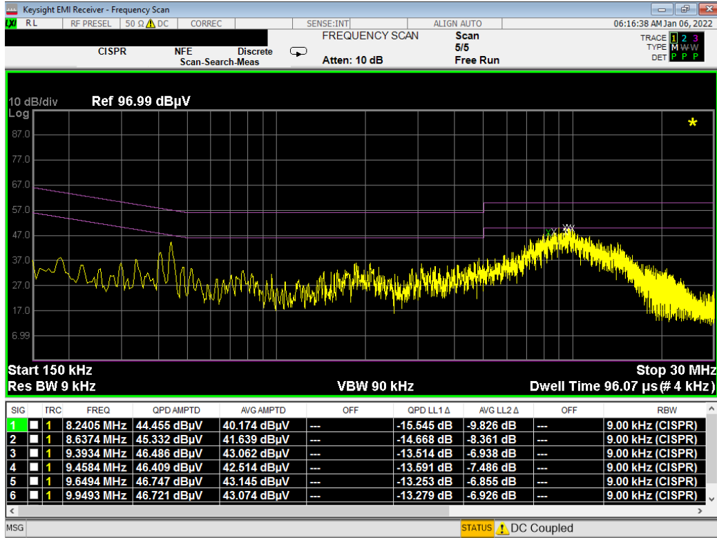
Plot 7-48. Line-Conducted Test Plot (L1)
