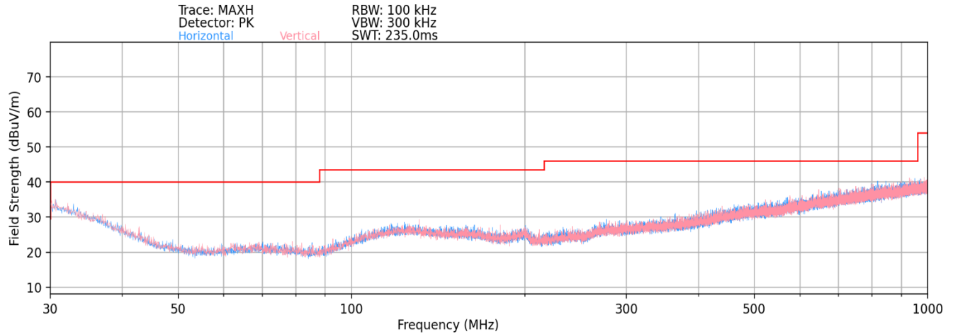
Plot 7-47. Radiated Spurious Plot below 1GHz
