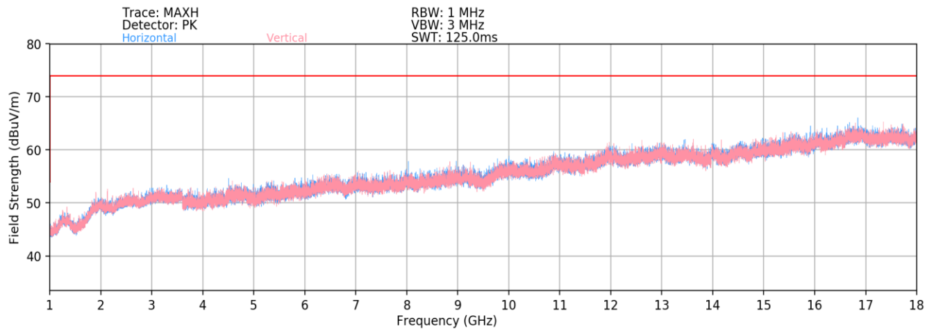
Plot 7-8. Radiated Spurious Plot above 1GHz [Radiated Test Config. 4]
