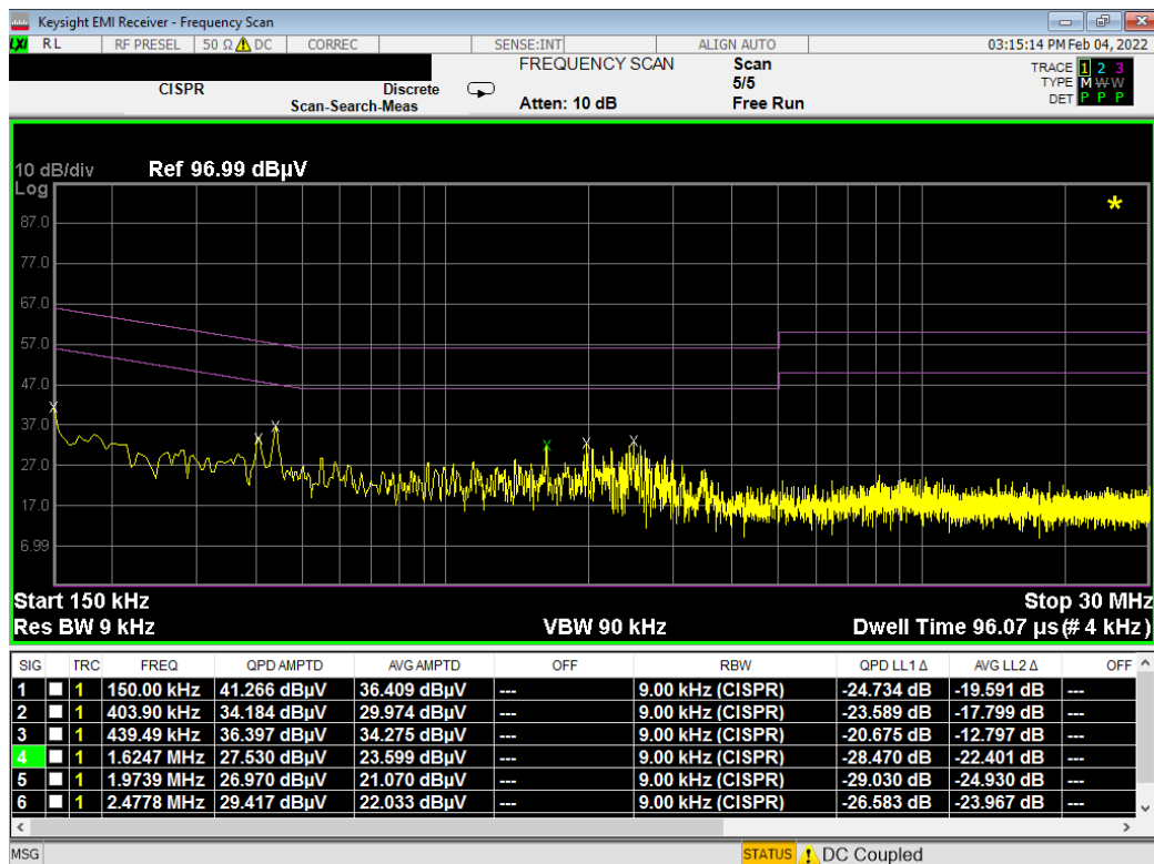
Plot 7-16. Line Conducted Plot (N)- Config 4
