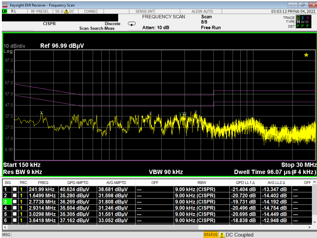
Plot 7-12. Line Conducted Plot (N)- Config 2
