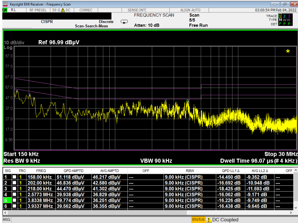
Plot 7-9. Line Conducted Plot (L1)- Config 1
