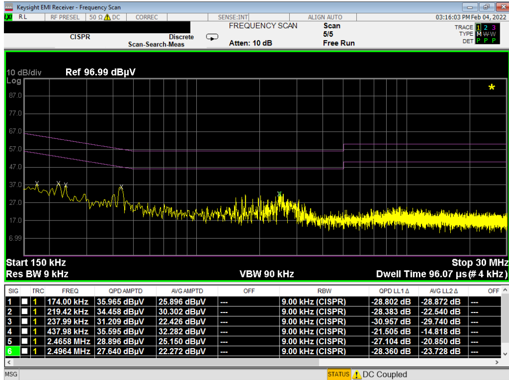
Plot 7-15. Line Conducted Plot (L1)- Config 4
