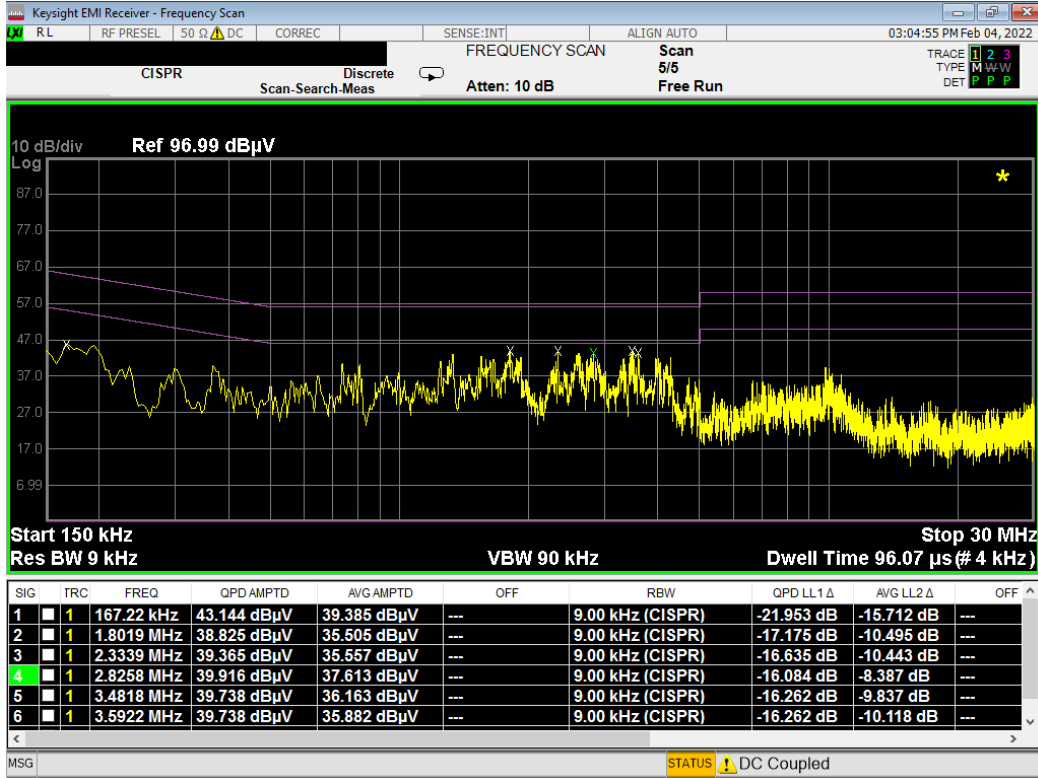
Plot 7-11. Line Conducted Plot (L1)- Config 2
