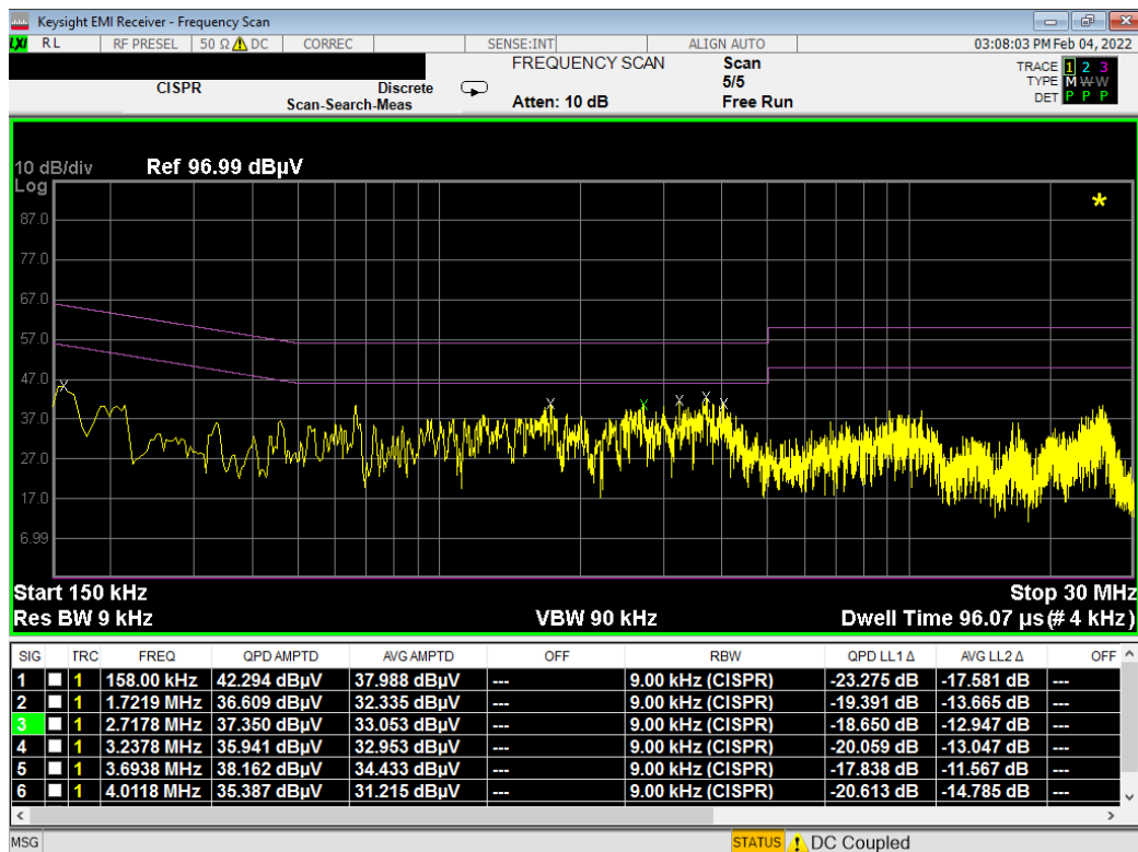
Plot 7-14. Line Conducted Plot (N)- Config 3
