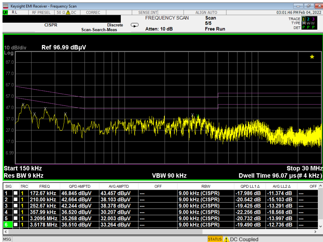
Plot 7-10. Line Conducted Plot (N)- Config 1
