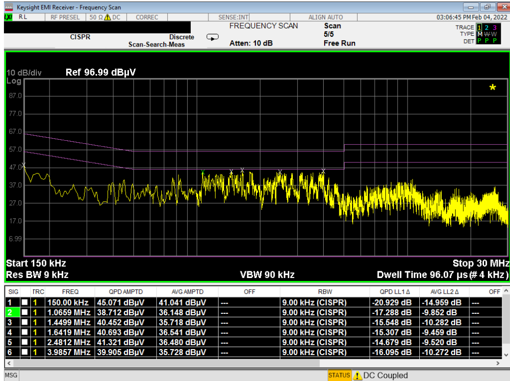
Plot 7-13. Line Conducted Plot (L1)- Config 3
