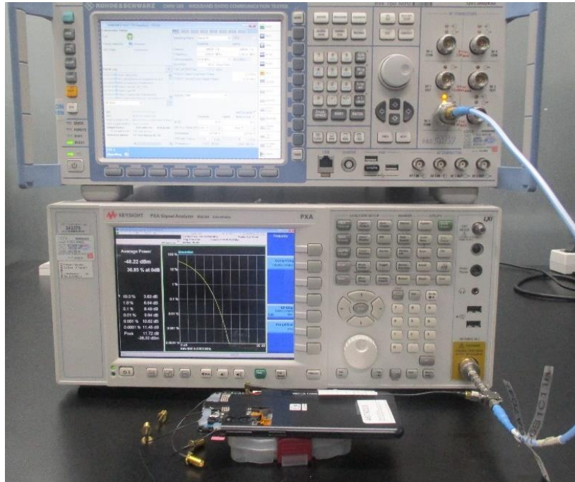
LICENSED BAND TEST PHOTO
