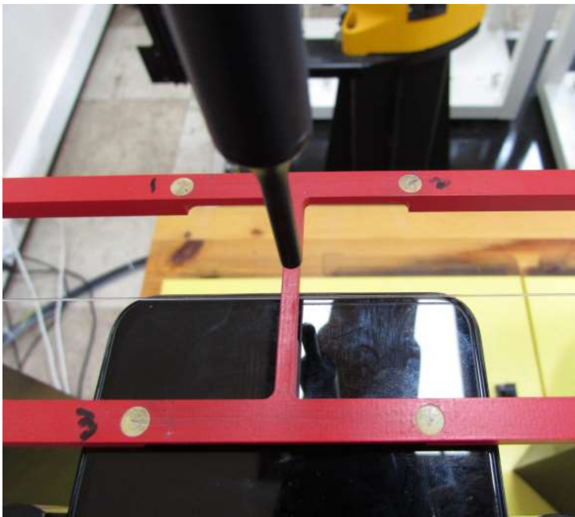
[ Setup Photo _ Front ]
