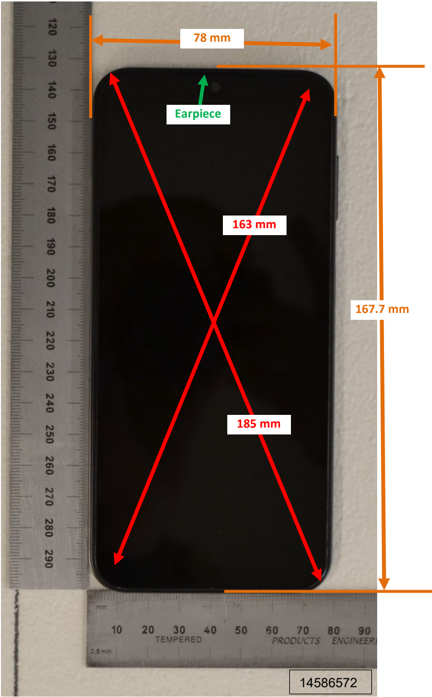
Photograph 1: Overall Dimensions
