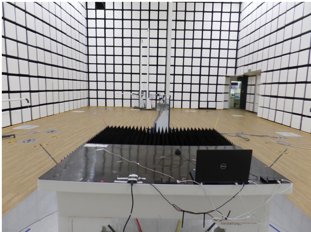
[ Mode 5 : Rear ]
