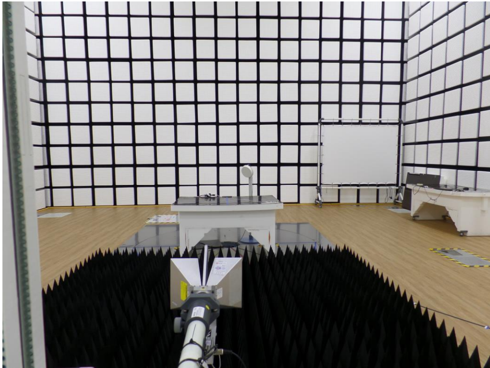
[ Mode 1 : Front ]
