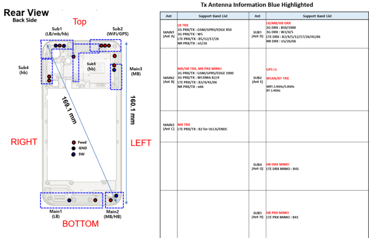
Figure J-1 DUT Antenna Locations
