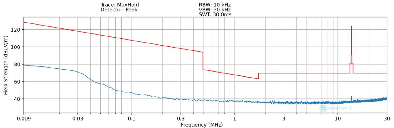
Plot 7-2. Radiated Spurious Plot 9kHz – 30MHz (Pol. Y)
