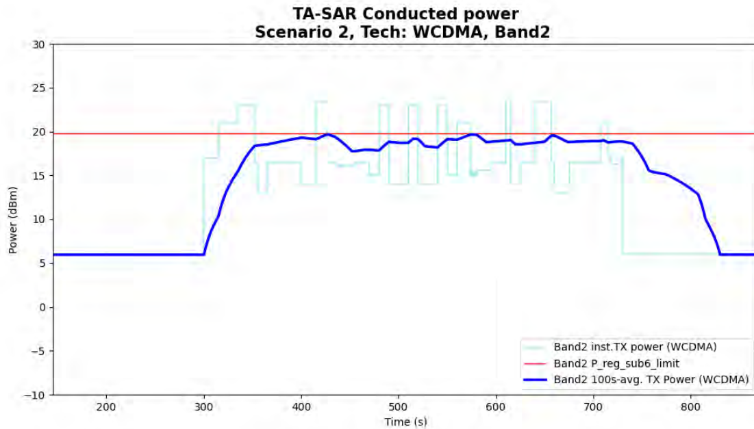
Figure 5- 30 Time-averaged conducted TX power over time for case 9 (WCDMA B2)
