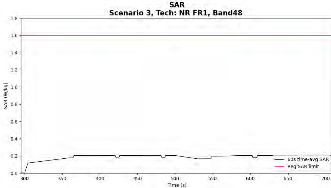
Figure 5- 43 Time-averaged SAR for case 13 (sub NR B48)
