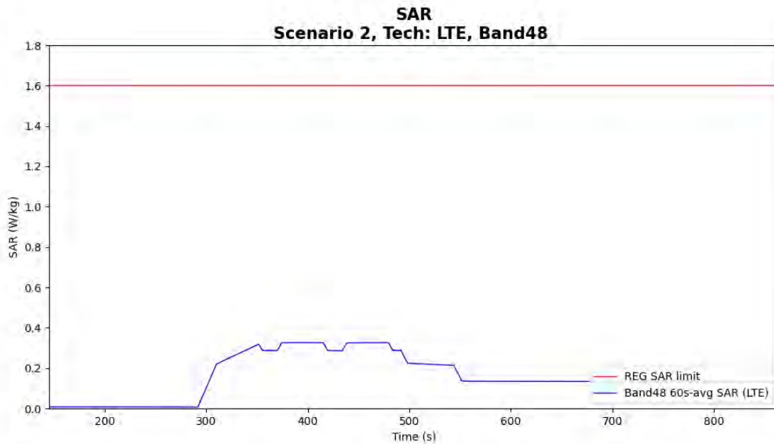
Figure 6-8 Time-averaged SAR for case 4 in table 6-1 (LTE B48)
