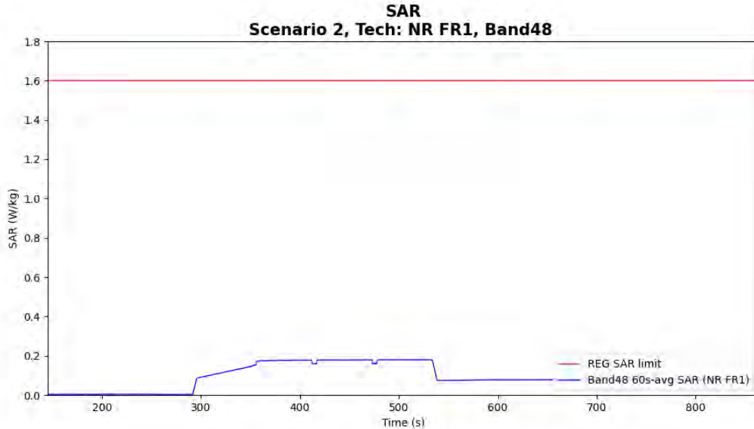
Figure 6-3 Time-averaged SAR for case 5 in table 6-1 (sub6 NR n48)
