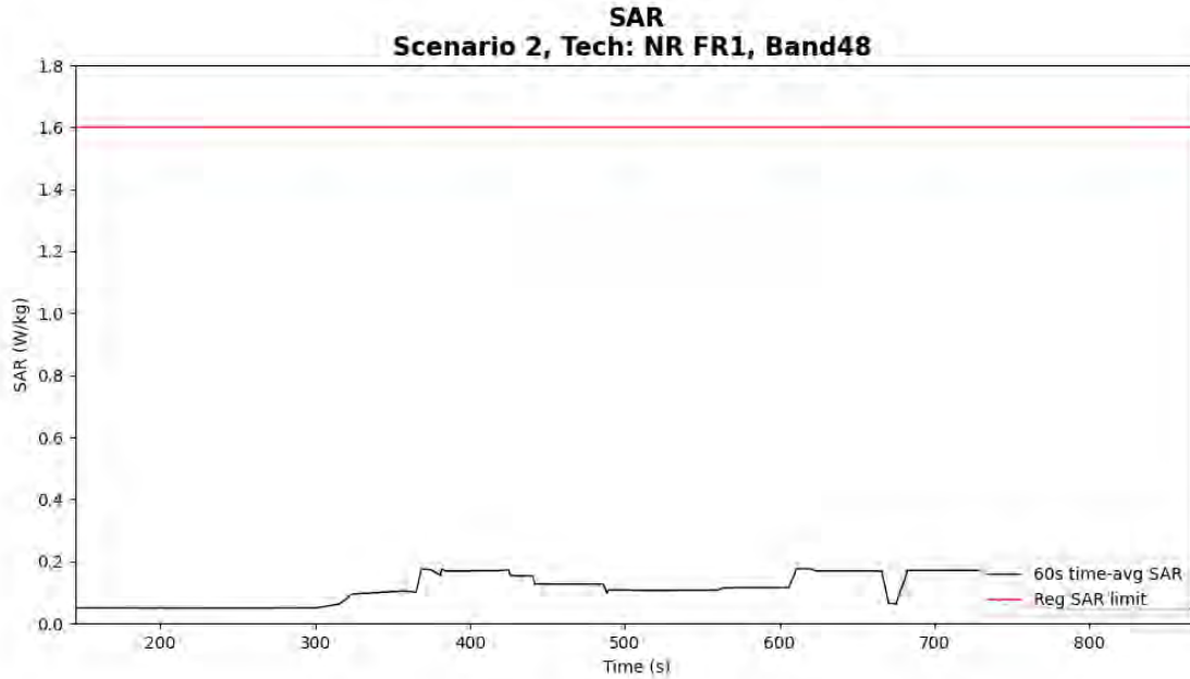
Figure 5- 15 Time-averaged SAR for case 11 (sub6 NR n48)
