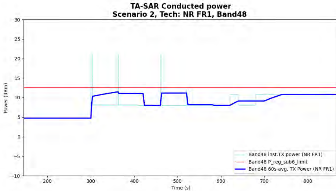
Figure 5- 10 Time-averaged conducted TX power over time for case 5 (sub6 NR n48)
