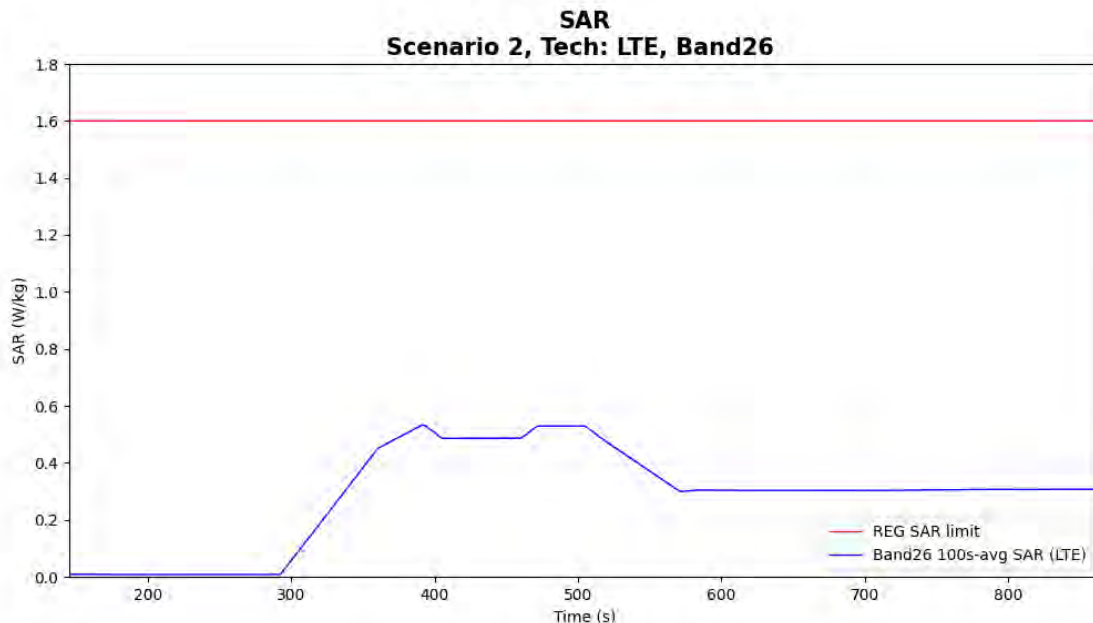
Figure 6-7 Time-averaged SAR for case 3 in table 6-1 (LTE B26)
