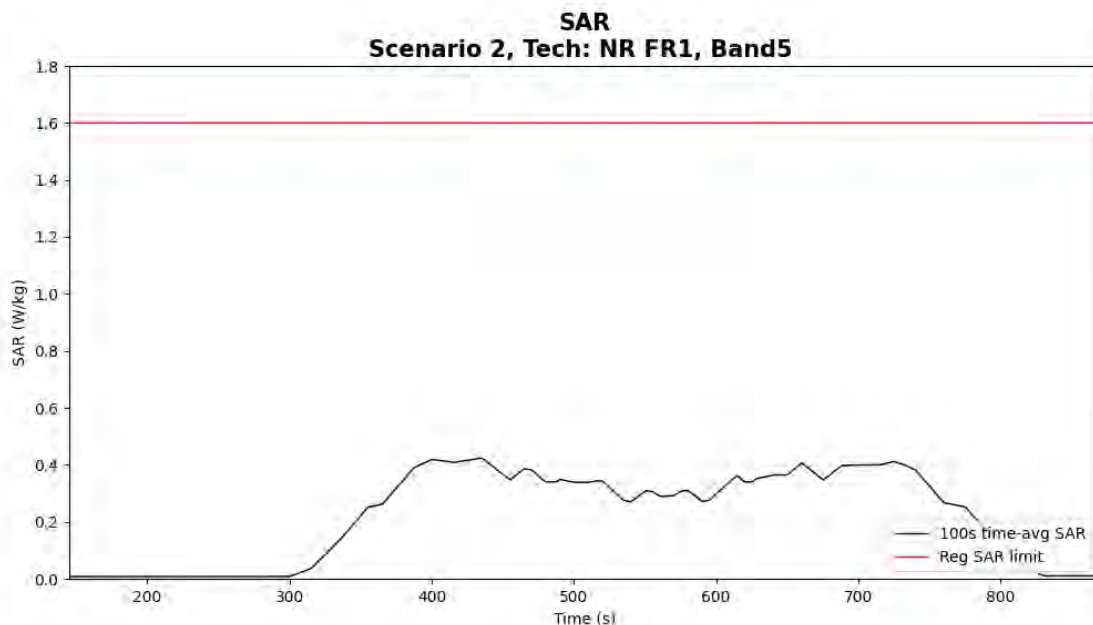
Figure 5- 17 Time-averaged SAR for case 12 (sub6 NR n5)
