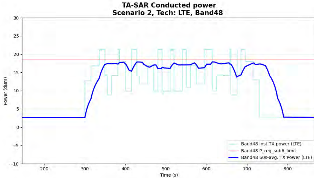
Figure 5- 24 Time-averaged conducted TX power over time for case 10 (LTE B48)
