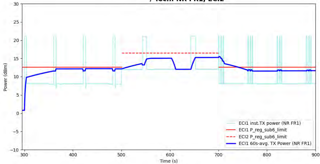
Figure 5- 46 Time-averaged conducted TX power over time for case 15 (sub6 NR B48)
