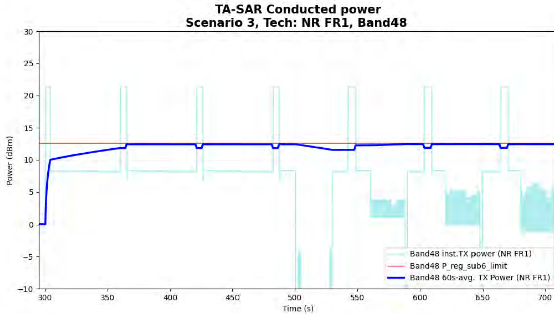
Figure 5- 42 Time-averaged conducted TX power over time for case 13 (sub NR B48)
