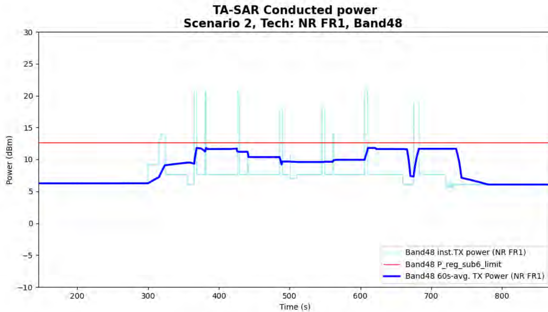
Figure 5- 14 Time-averaged conducted TX power over time for case 11 (sub6 NR n48)
