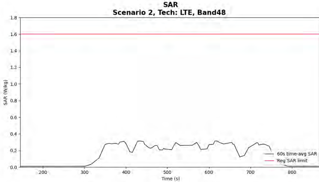
Figure 5- 25 Time-averaged SAR for case 10 (LTE B48)
