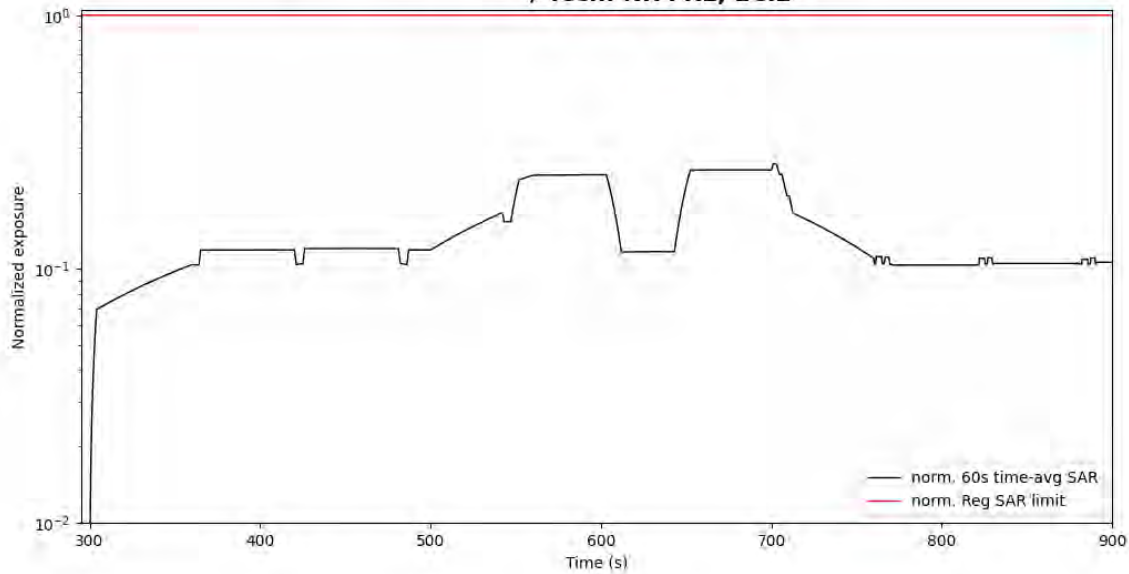
Figure 5- 47 Normalized time-averaged SAR for case 15 (sub6 NR B48)
