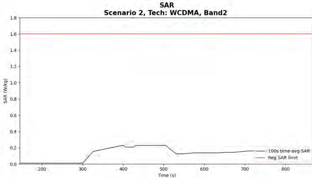
Figure 5- 27 Time-averaged SAR for case 2 (WCDMA B2)
