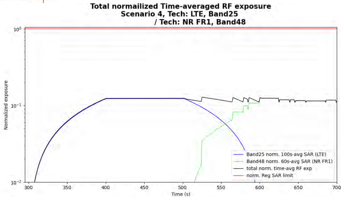
Figure 5- 45 Normalized time-averaged SAR for case 14 (LTE B25, sub6 NR B48)
