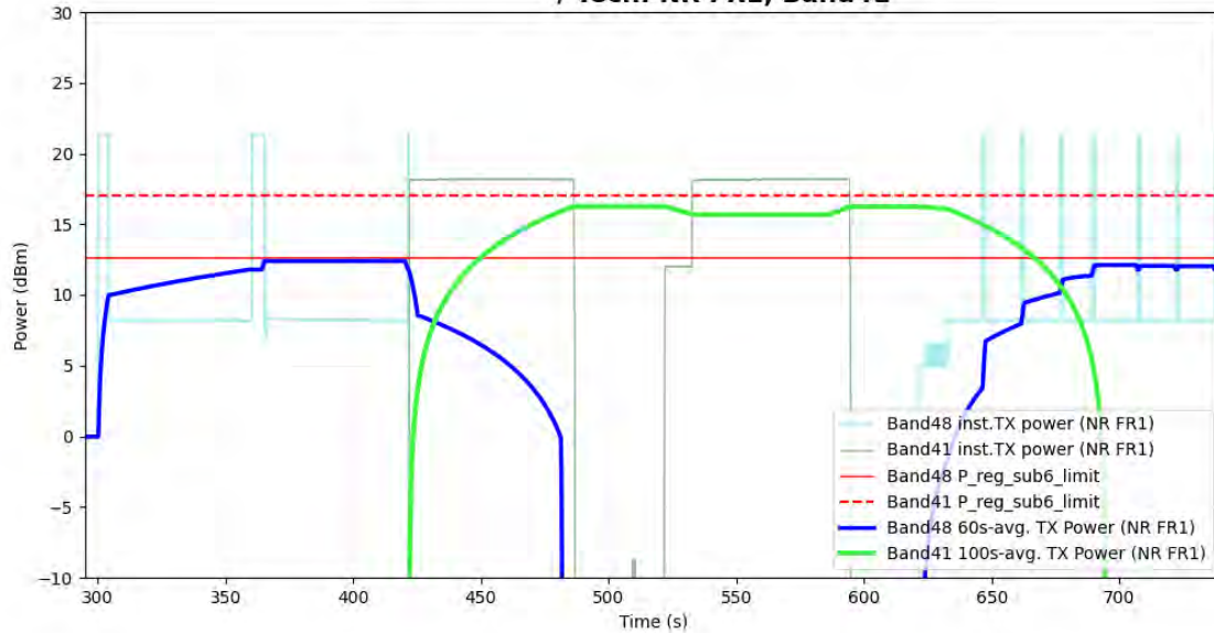
Figure 5- 50 Time-averaged conducted TX power over time for case 16 (sub6 NR B48 and B41)
