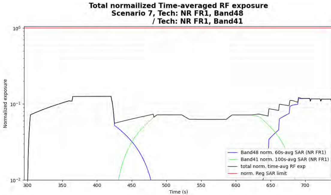
Figure 5- 51 Normalized time-averaged SAR for case 16 (sub6 NR B48 and B41)
