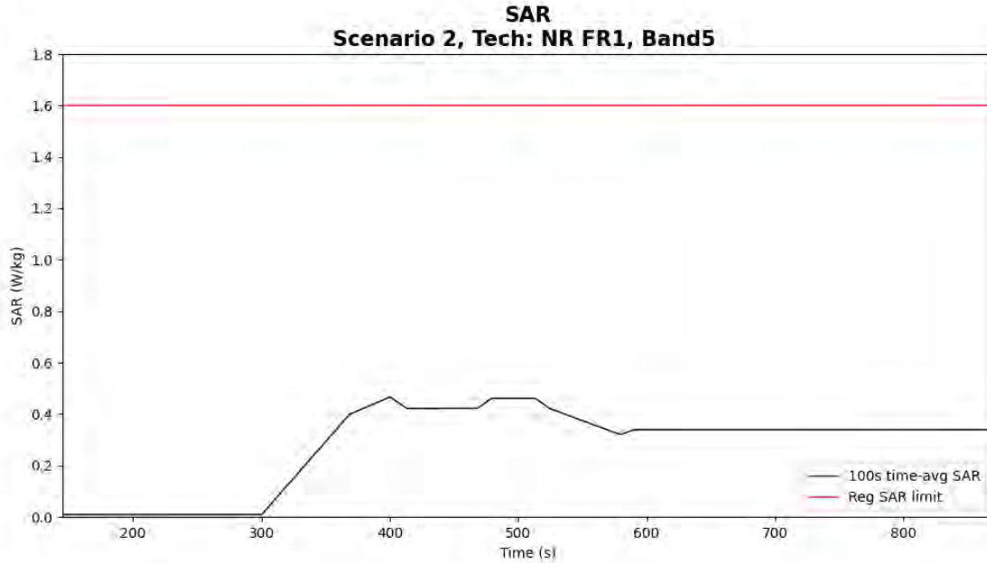
Figure 5- 13 Time-averaged SAR for case 6 (sub6 NR n5)
