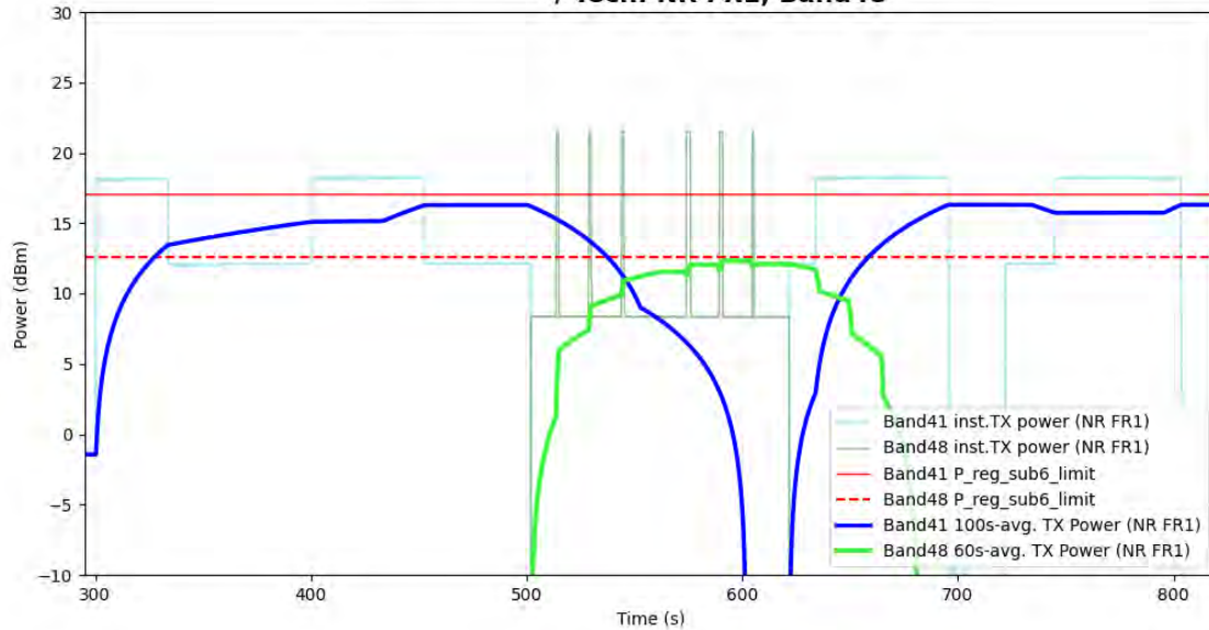
Figure 5- 52 Time-averaged conducted TX power over time for case 17 (sub6 NR B41 and B48)
