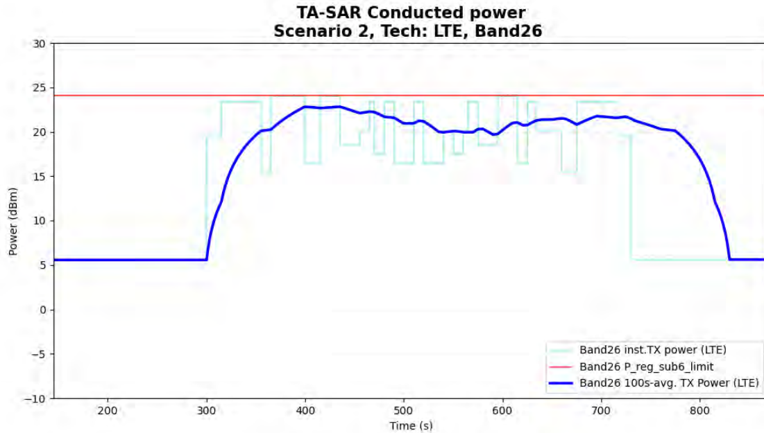
Figure 5- 22 Time-averaged conducted TX power over time for case 9 (LTE B26)
