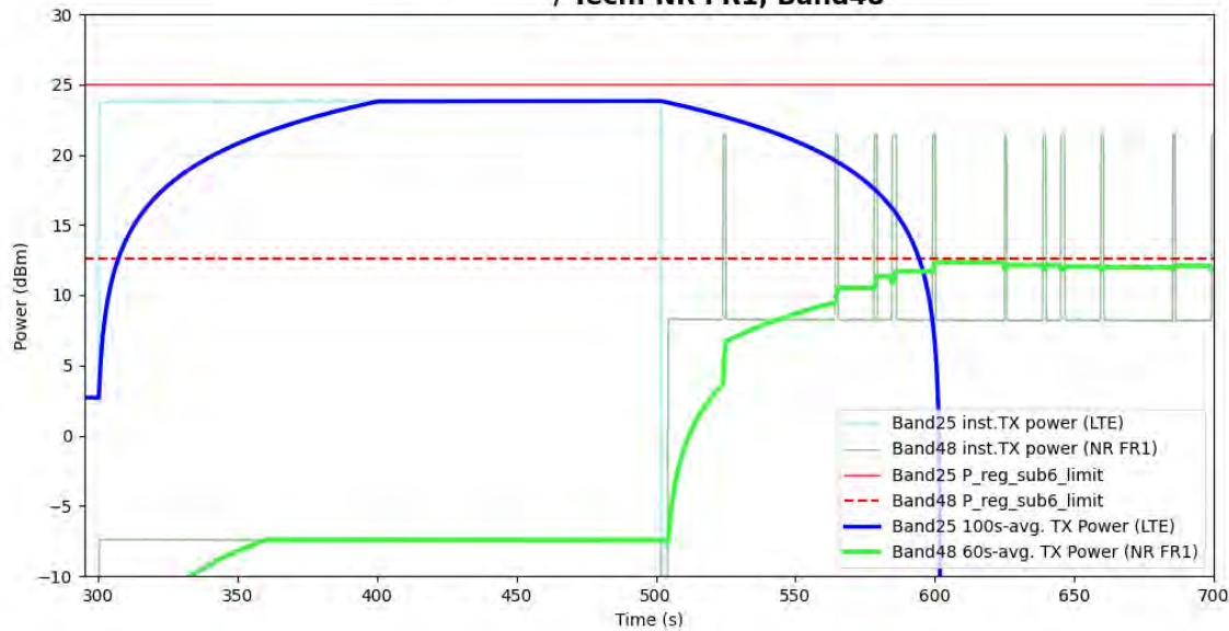
Figure 5- 44 Time-averaged conducted TX power over time for case 14 (LTE B25, sub6 NR B48)
