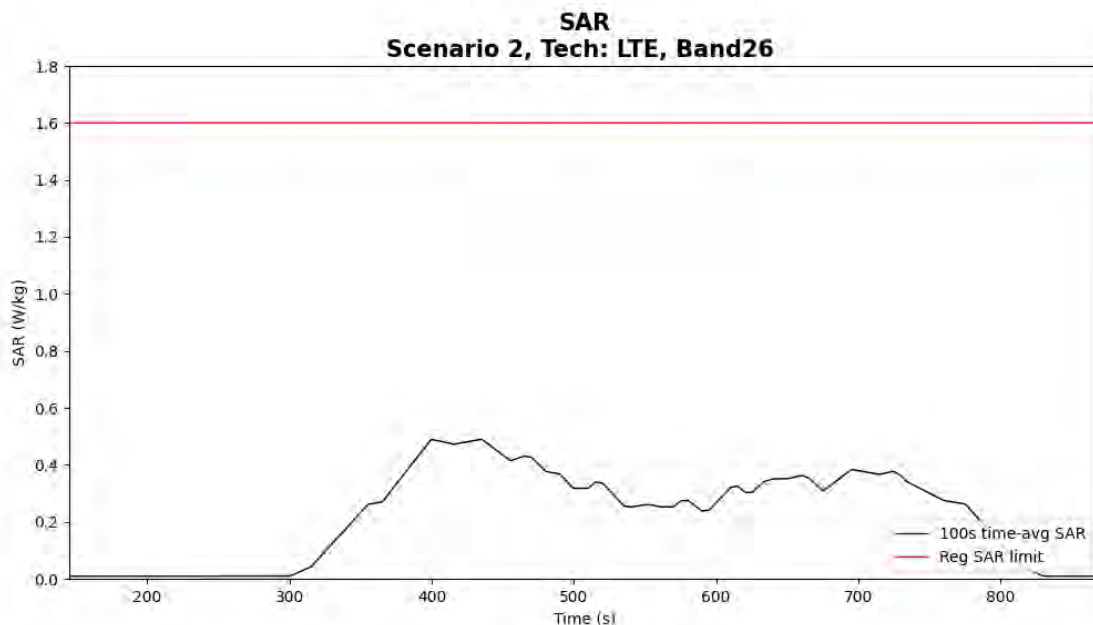
Figure 5- 23 Time-averaged SAR for case 9 (LTE B26)
