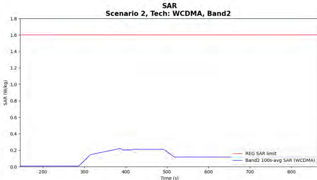
Figure 6-11 Time-averaged SAR for case 1 in table 6-1 (WCDMA B2)
