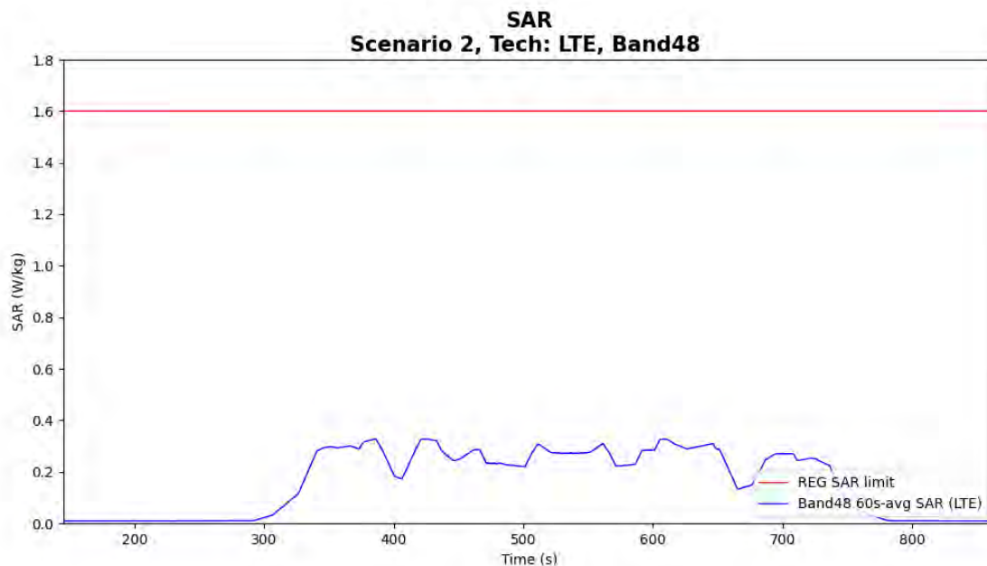
Figure 6-10 Time-averaged SAR for case 10 in table 6-1 (LTE B48)
