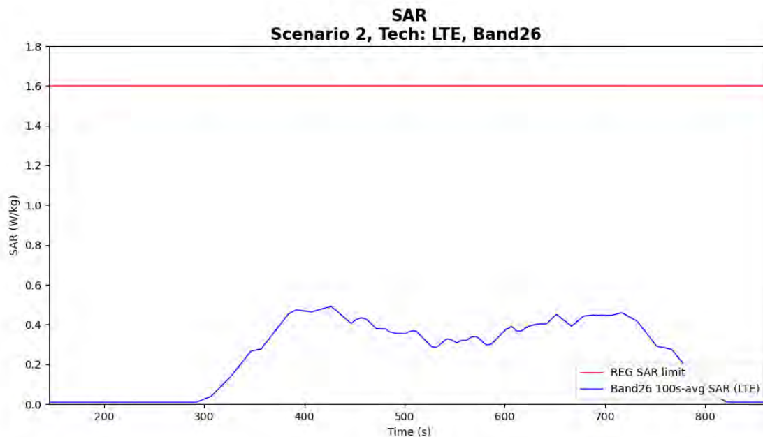
Figure 6-9 Time-averaged SAR for case 9 in table 6-1 (LTE B26)
