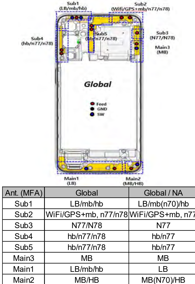
Figure 5- 1 Antenna placement of the phone
