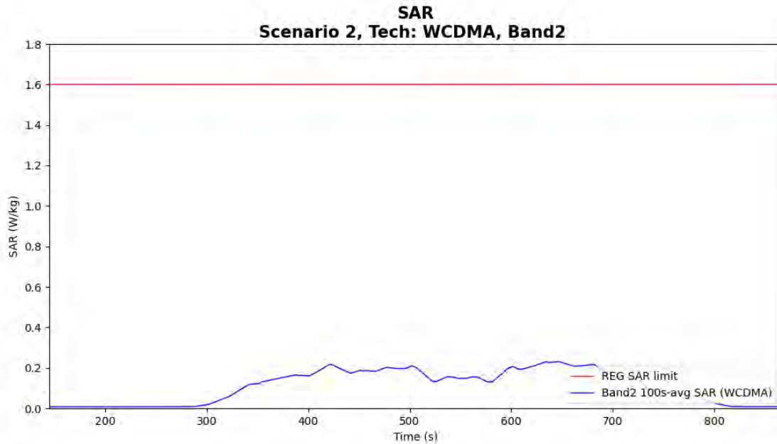
Figure 6-13 Time-averaged SAR for case 7 in table 6-1 (WCDMA B2)
