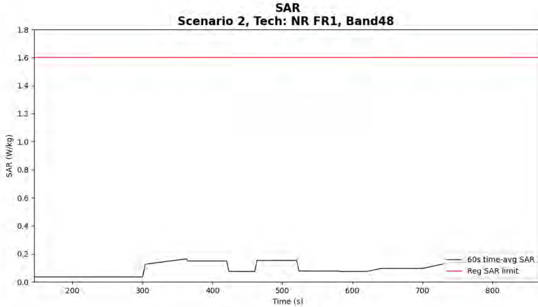
Figure 5- 11 Time-averaged SAR for case 5 (sub6 NR n48)
