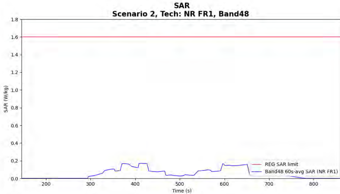
Figure 6-5 Time-averaged SAR for case 11 in table 6-1 (sub6 NR n48)
