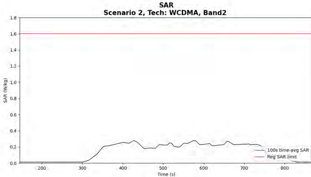
Figure 5- 31 Time-averaged SAR for case 9 (WCDMA B2)
