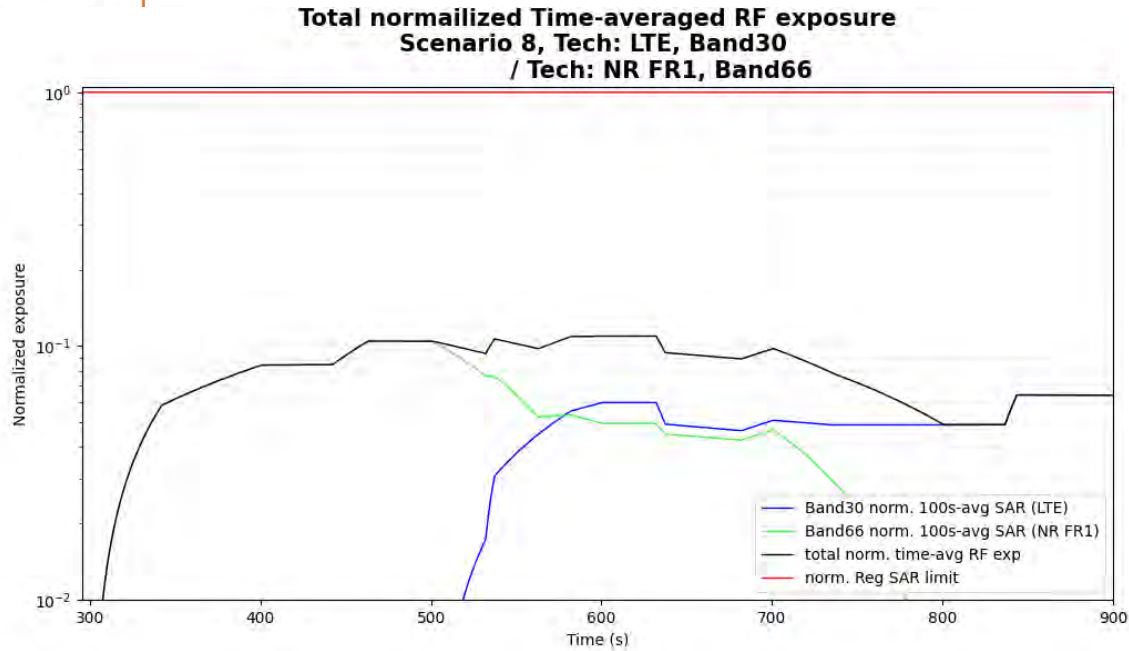
Figure 5- 55 Normalized time-averaged SAR for case 18 (LTE B30, sub6 NR n66)
