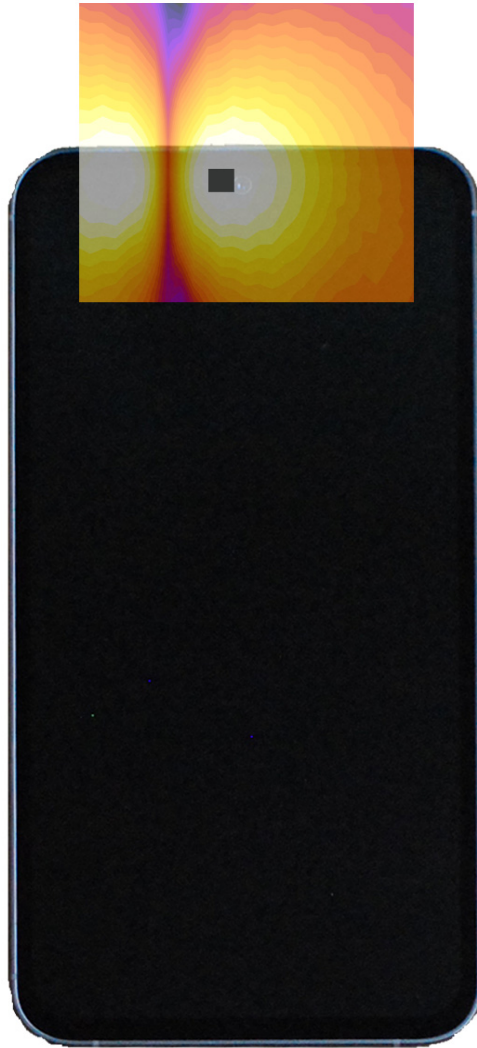
Radial (Transverse) Figure 18-3 T-Coil Scan Overlay Magnetic Field Distributions
