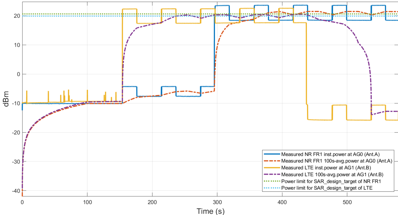
Plot.1 : Conducted Tx power for NR :
