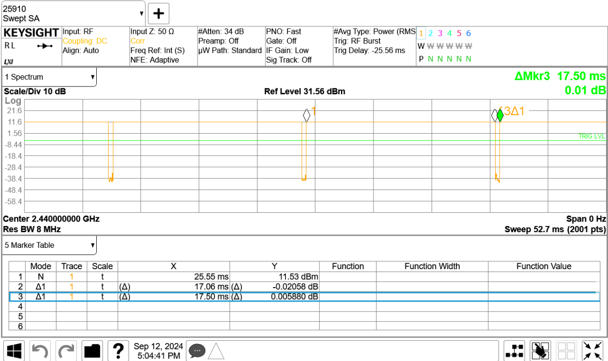
Duty Cycle plot (BLE-125kbps 255pkt)
