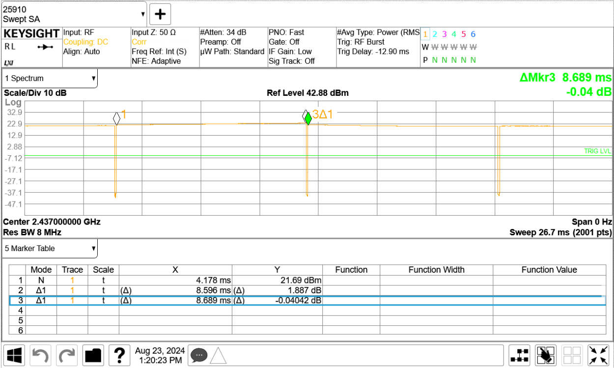
Duty Cycle plot (802.11b)
