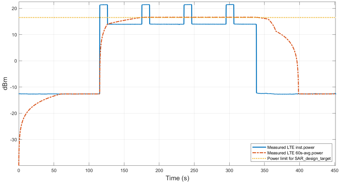
Plot.1 : Conducted Tx power for LTE Uplink CA:
