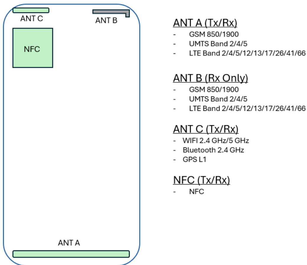
Figure A SAR Test Setup – Antenna Diagram
