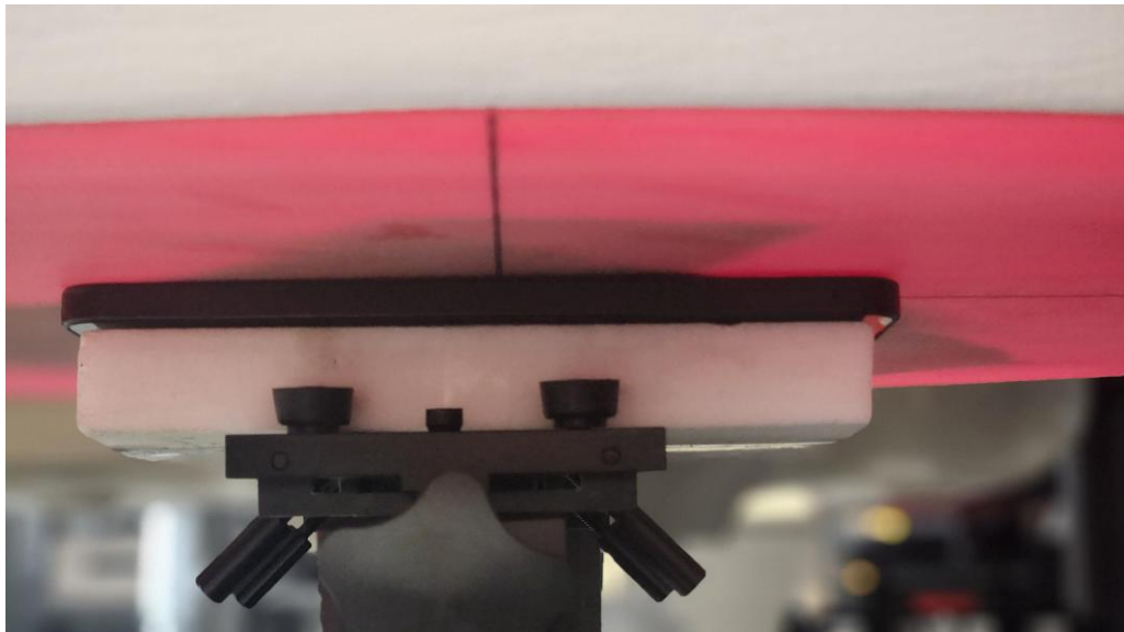
Figure U SAR Test Setup – Phablet on ELI – Back 0mm
