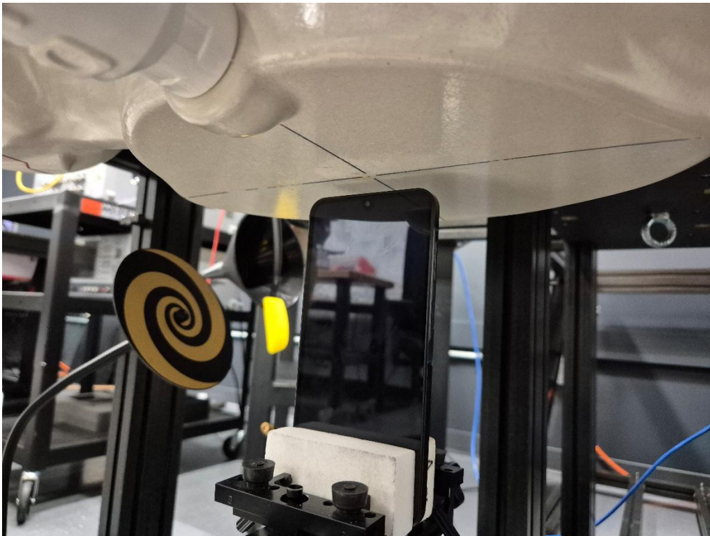
Figure O SAR Test Setup – Hotspot – Top 10mm
