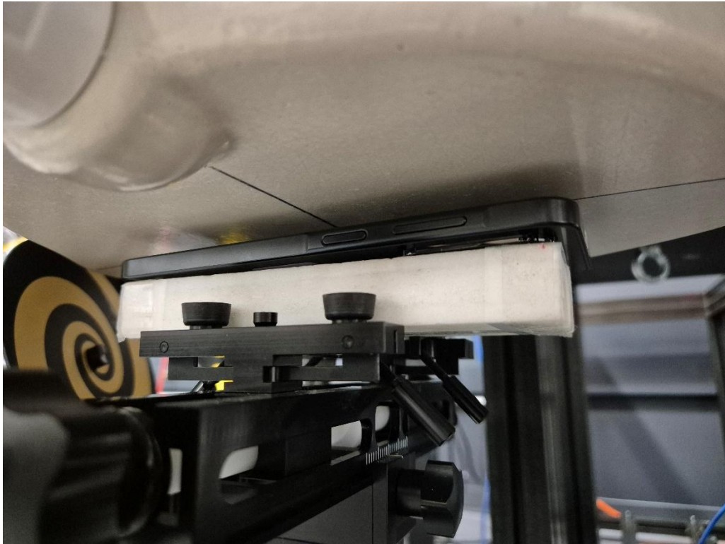
Figure L SAR Test Setup – Hotspot – Front 10mm
