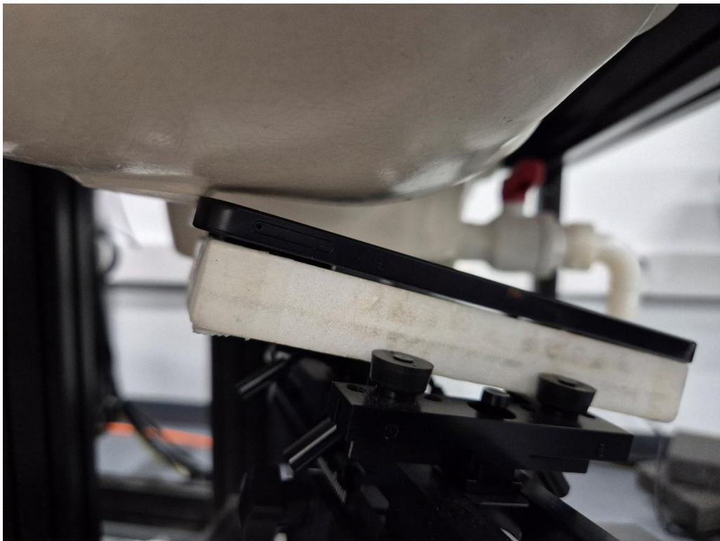
Figure C SAR Test Setup – Head – Right Tilt 0mm
