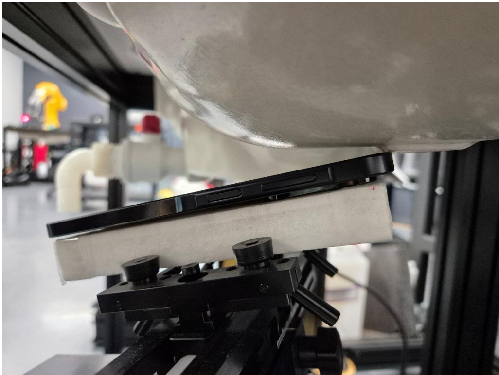
Figure E SAR Test Setup – Head – Left Tilt 0mm
