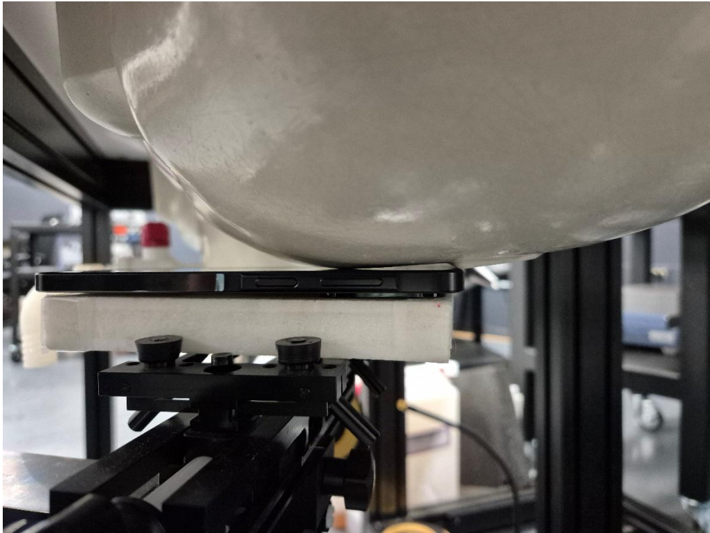
Figure D SAR Test Setup – Head – Left Cheek 0mm
