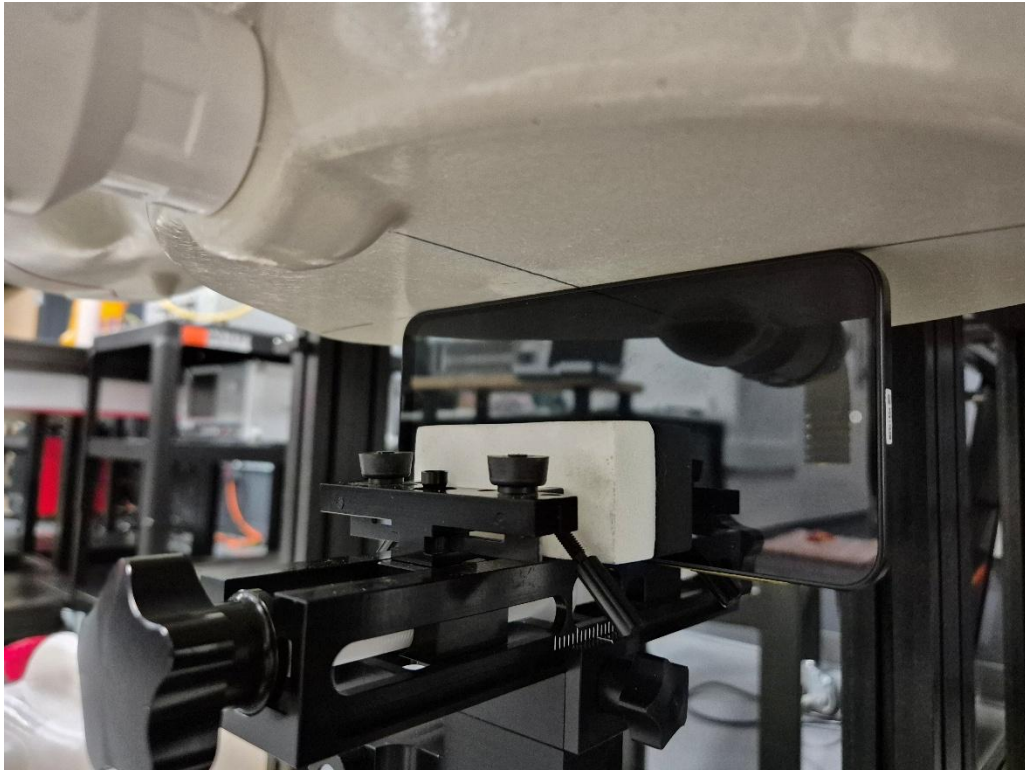
Figure T SAR Test Setup – Phablet – Left 0mm
