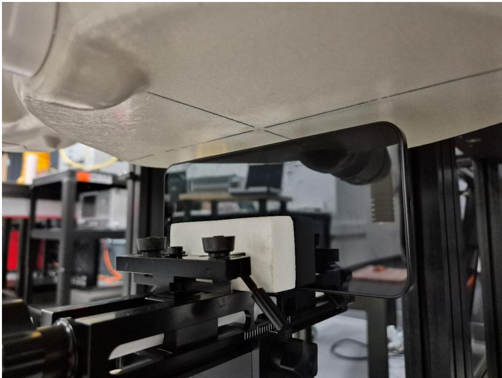
Figure R SAR Test Setup – Hotspot – Right 10mm
