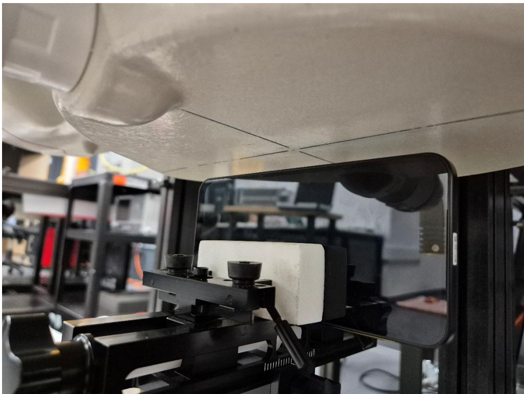
Figure S SAR Test Setup – Hotspot – Left 10mm
