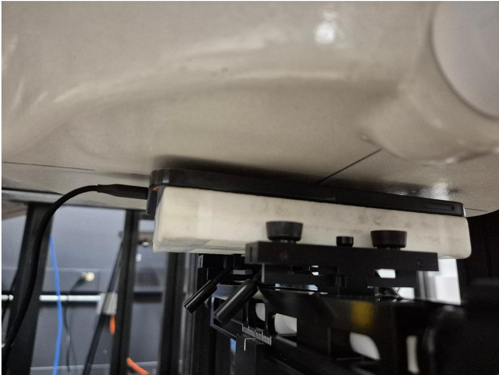
Figure J SAR Test Setup – Body-worn – Back 5mm with a Headset
