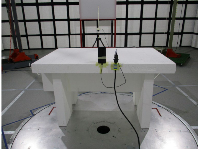
RADIATED PHOTO (<30 MHz WWAN Tx)
