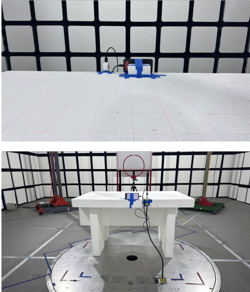
RADIATED PHOTO (<30 MHz BT/BLE/2.4GHz WLAN)
