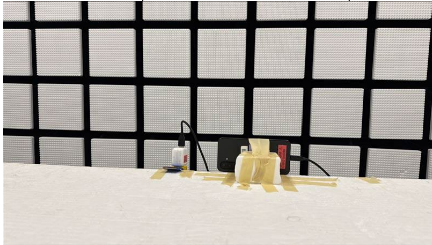
RADIATED PHOTO (>1GHz BT/BLE/2.4GHz WLAN)
