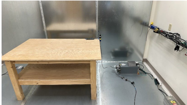
BT/BLE/2.4GHz WLAN/5GHz WLAN Tx AC MAINS SETUP
