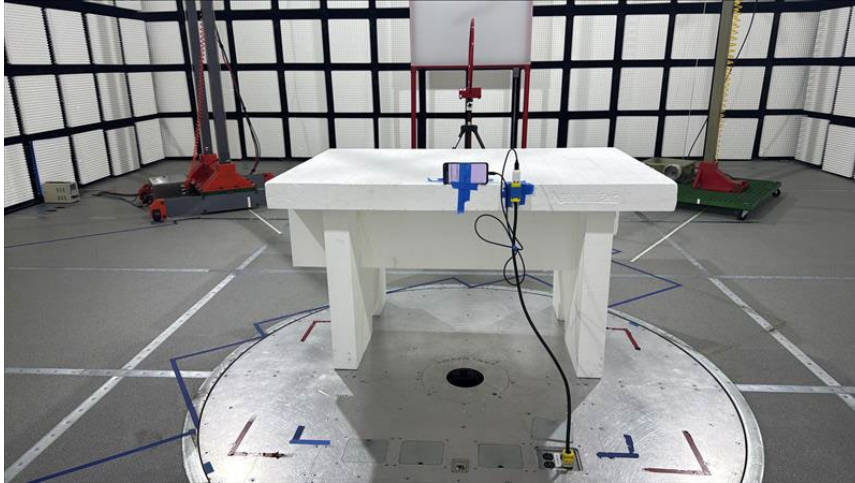
RADIATED PHOTO (<30 MHz BT/BLE/2.4GHz WLAN)
