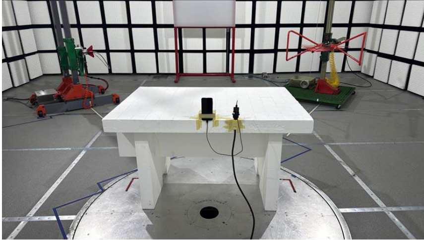
RADIATED PHOTO (30-1000MHz WWAN Tx)
