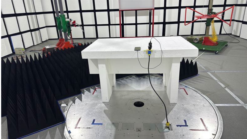
RADIATED PHOTO (>1GHz WWAN Rx and 15B)
