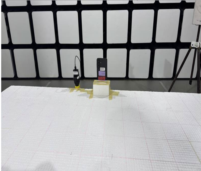
RADIATED PHOTO (<30 MHz WWAN Tx)
