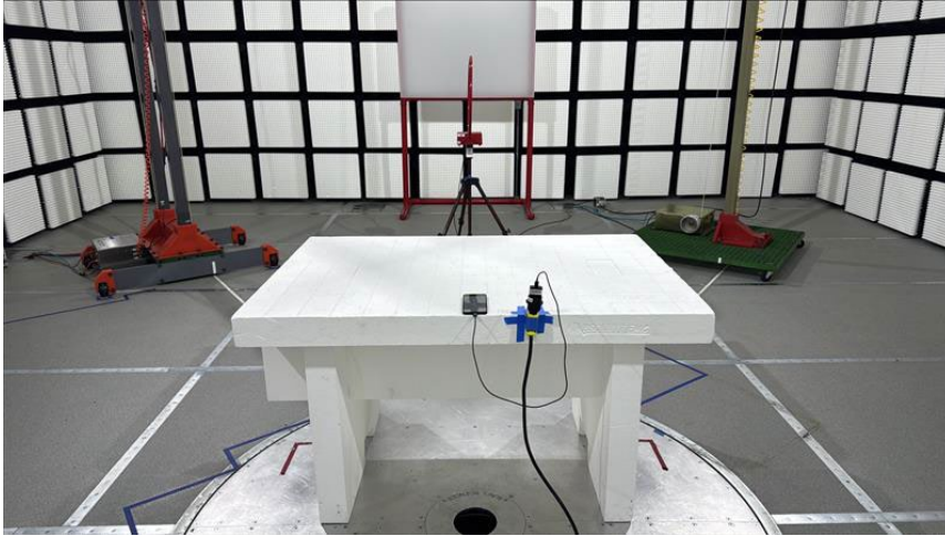
RADIATED PHOTO (<30 MHz 5GHz WLAN)
