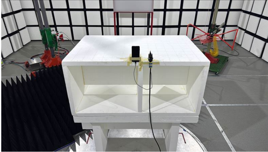
RADIATED PHOTO (>1GHz LOWBAND WWAN Tx)
