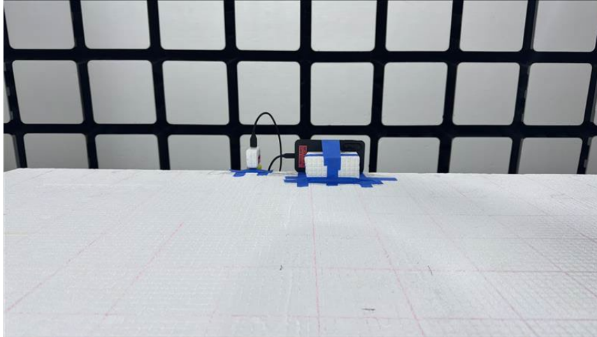
RADIATED PHOTO (30-1000MHz BT/BLE/2.4GHz WLAN)
