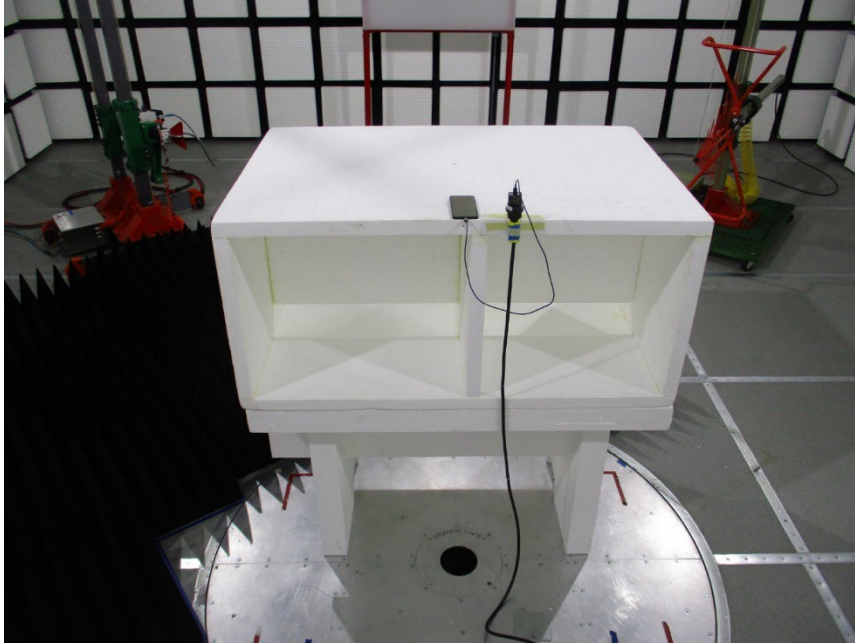
RADIATED PHOTO (>1GHz MIDBAND WWAN Tx)
