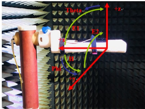
Figure 4: Geometry for SM-A175F for Radiation patterns.
