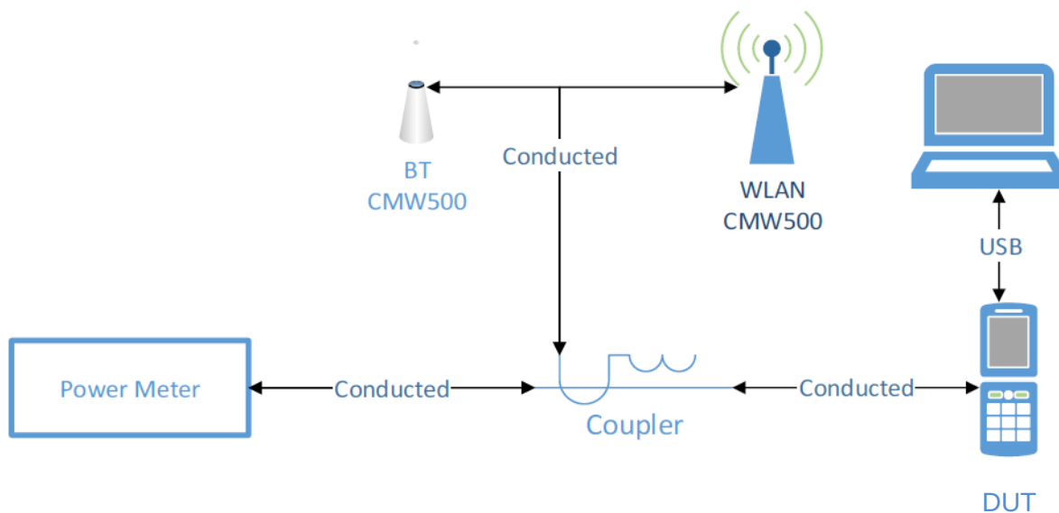
Figure 5.1-2 Test set-up for WLAN/BT
