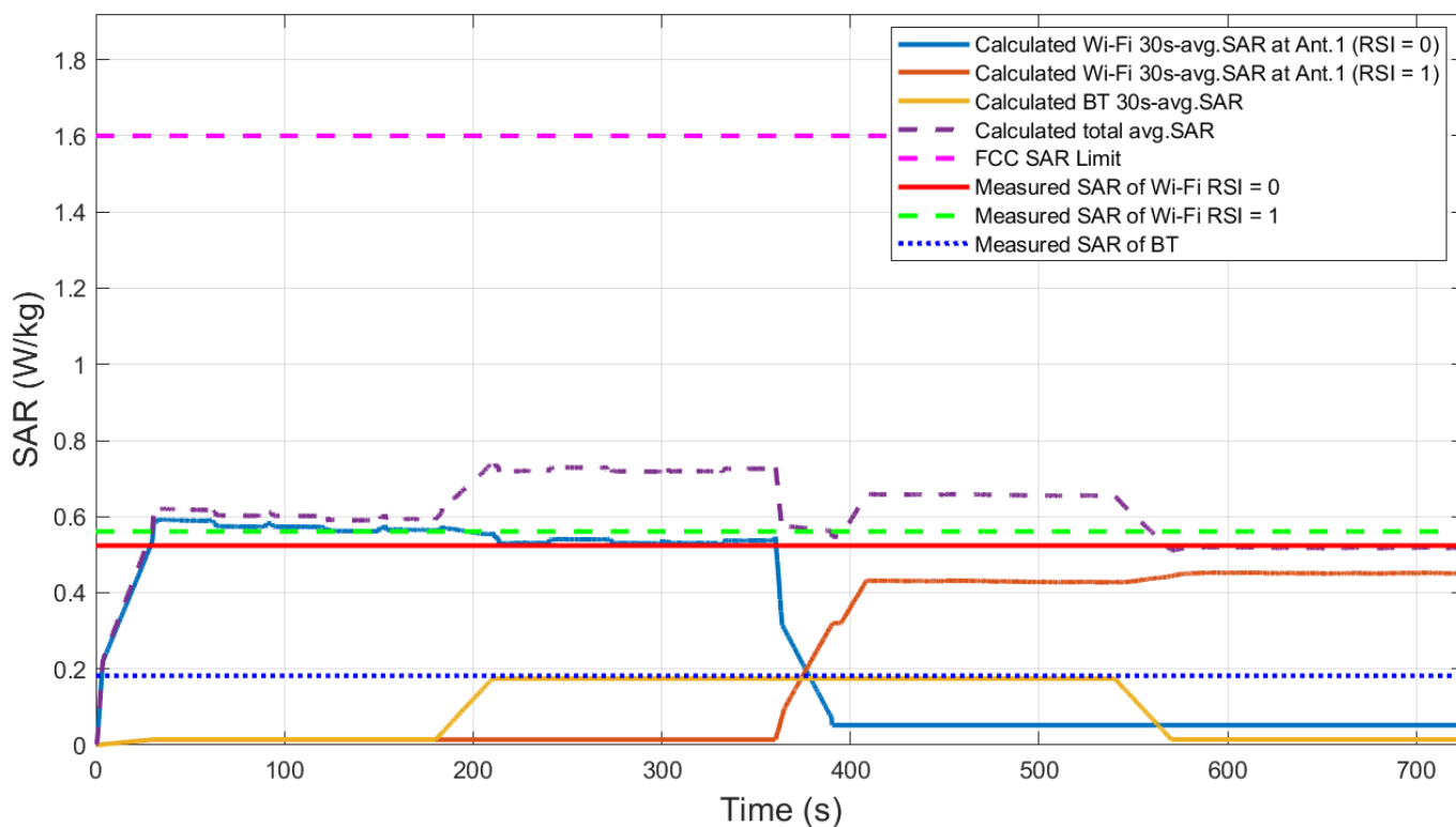
Plot.2 : Total time-averaged SAR Result :
