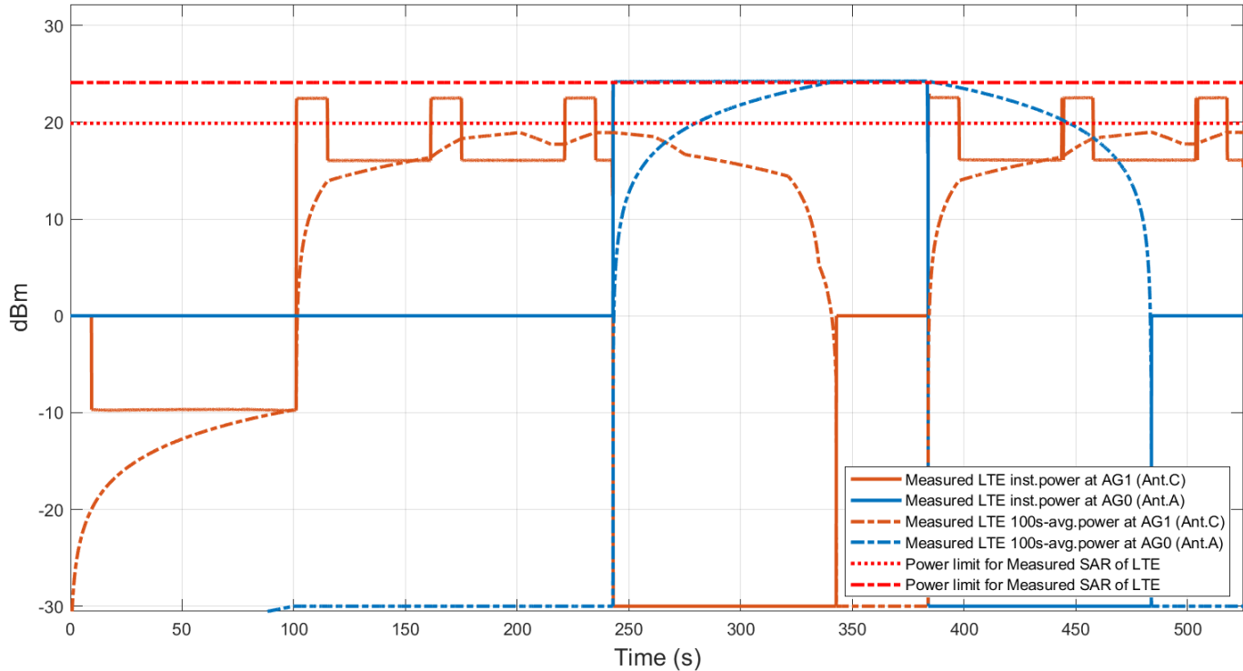
Plot.1 : Conducted Tx power for LTE :
