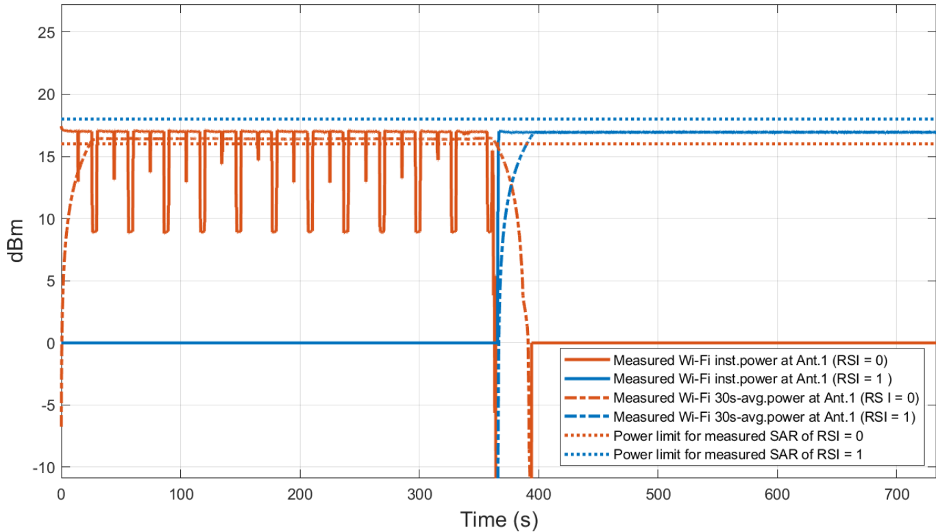
Plot.1 : Conducted Tx power for WLAN 2.4GHz :
