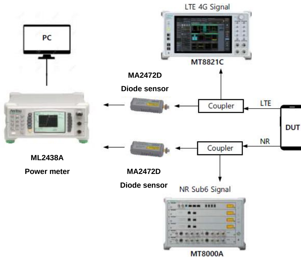
Figure 5.1-1 Test set-up for WWAN(legacy and sub 6GHz)
