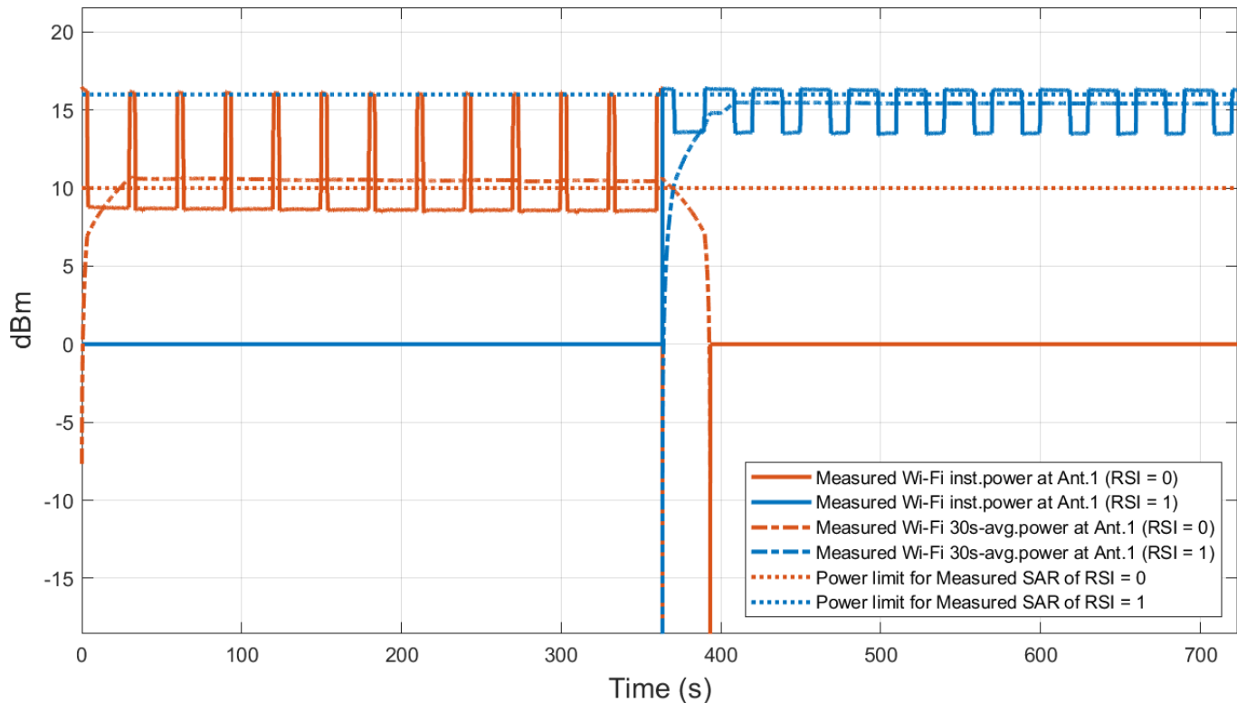
Plot.1 : Conducted Tx power for WLAN 5GHz :
