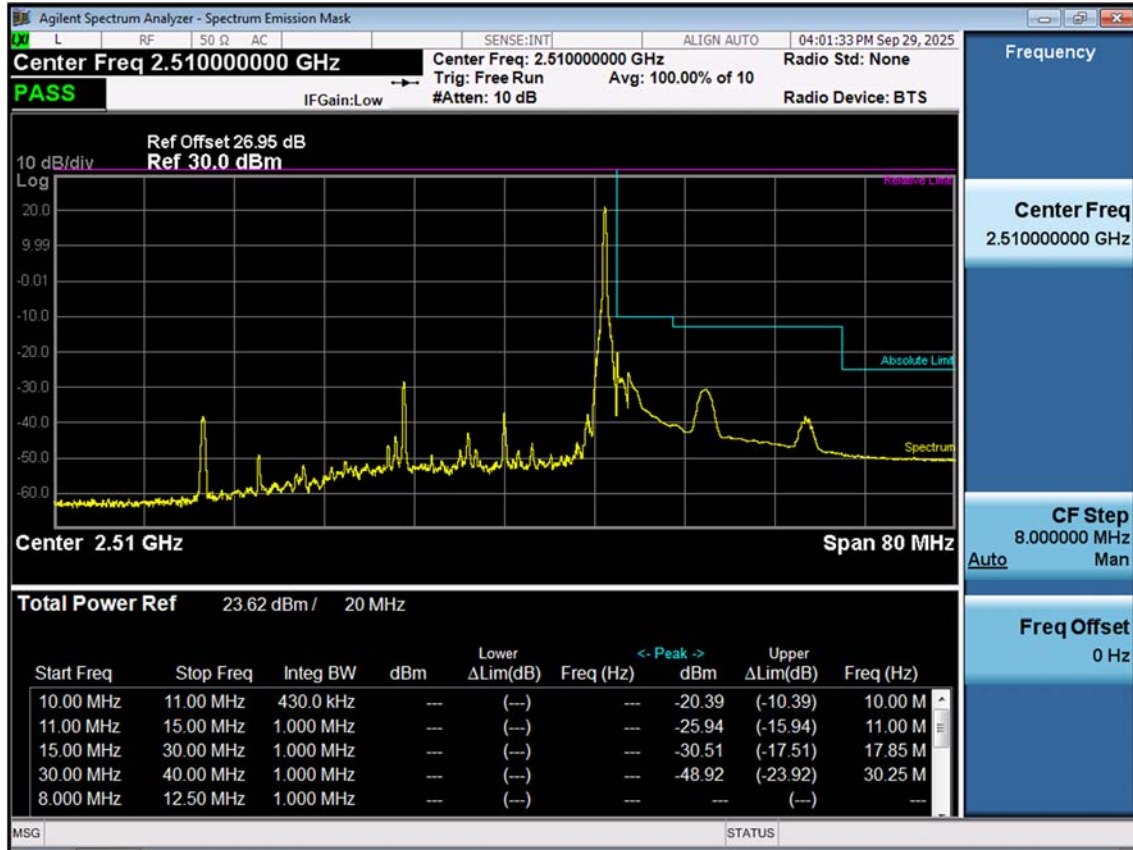
LTE B7_20 M_Channel Edge_Low_QPSK_1RB (2)
