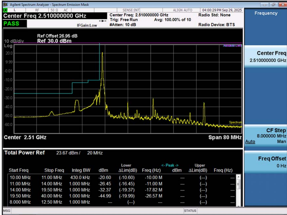
LTE B7_20 M_Channel Edge_Low_QPSK_1RB (1)
