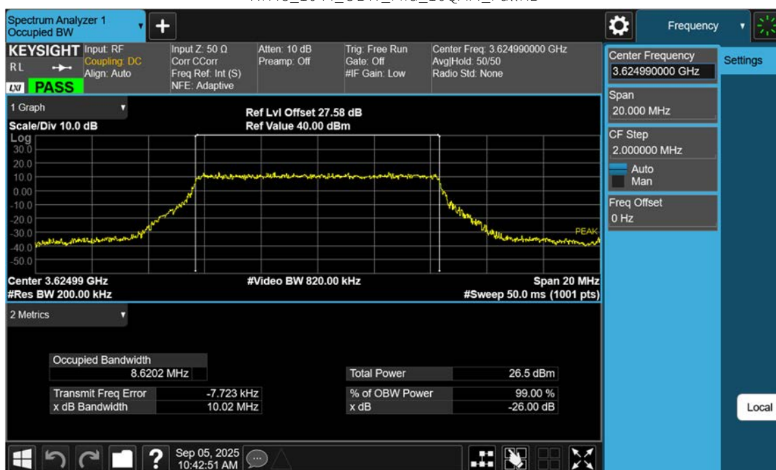
NR48_10 M_OBW_Mid_16QAM_FullRB
