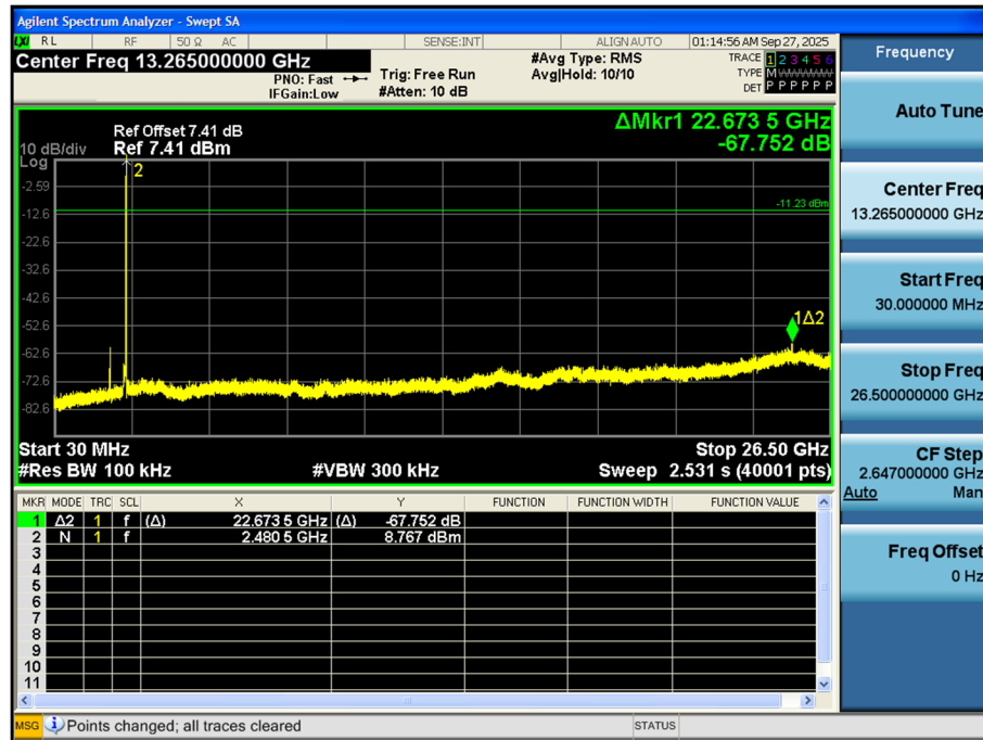
Spurious Emissions (30 MHz - 26.50 GHz) \pi/4 DQPSK Ch. 78
