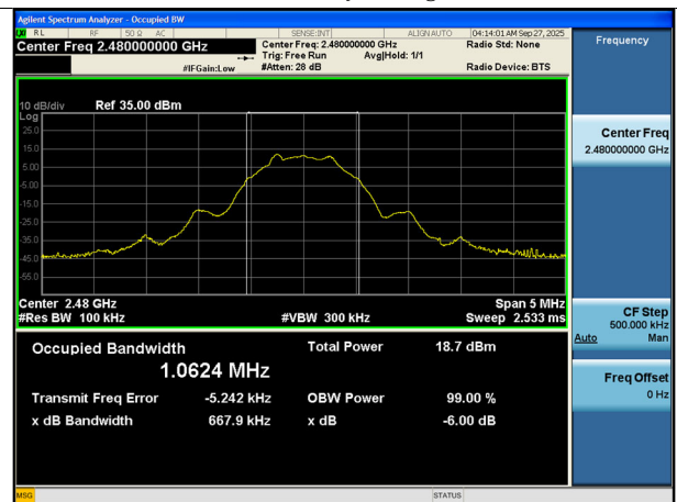
500k Bit/s 255 Byte (High-CH 39)
