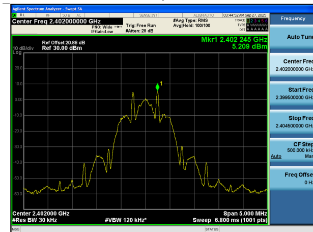
125k Bit/s 37 Byte (Low-CH 37)
