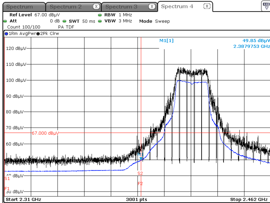
Radiated Restricted Band Edges plot – Average Result (802.11n (HT20)_MCS0, Ch.2, Z-V)
