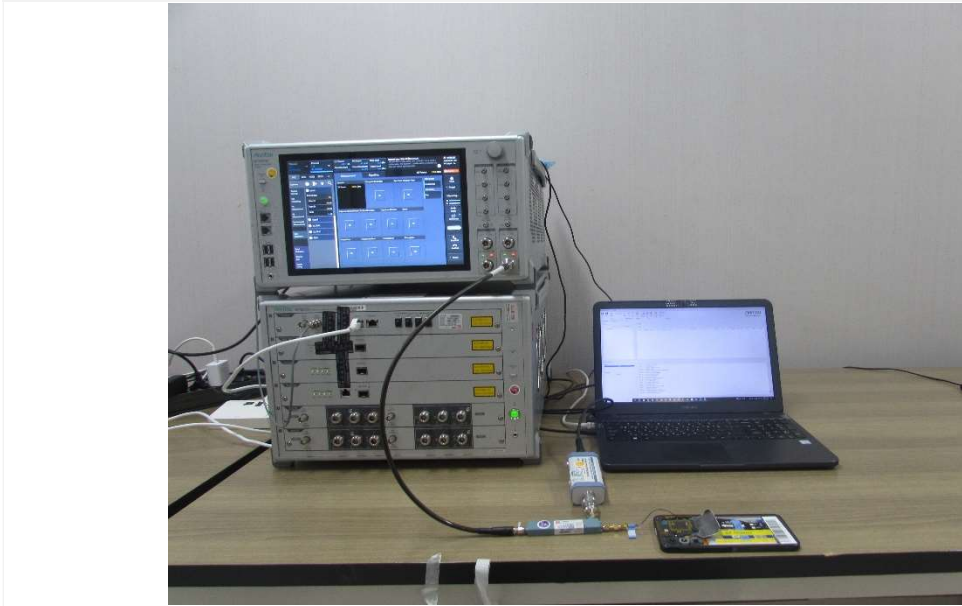
Test setup photo-1 TC01,03,04,05,07,08,09,10,16
