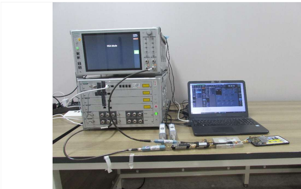
Test setup photo-6 TC15
