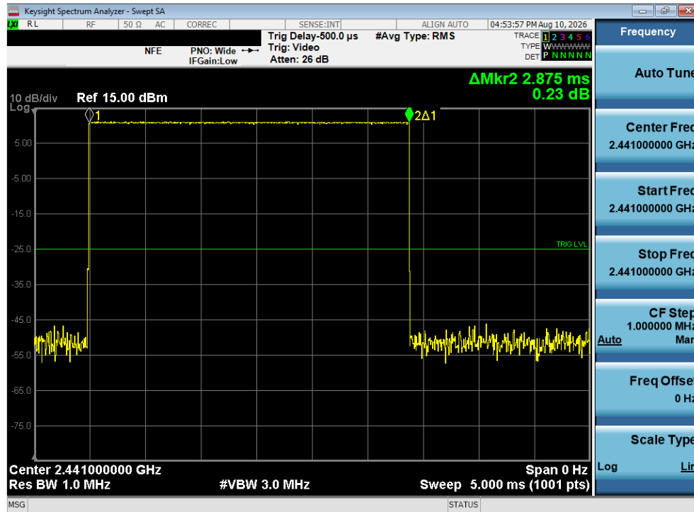
Plot 7-33. Time of Occupancy Plot (Bluetooth)
