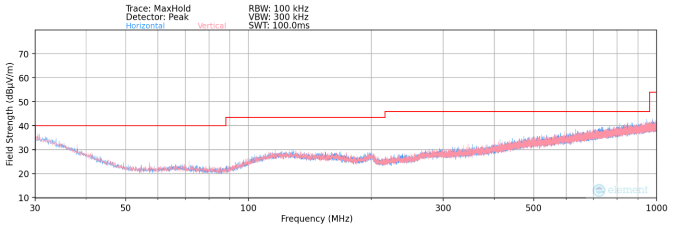
Plot 7-48. Radiated Spurious Plot below 1GHz
