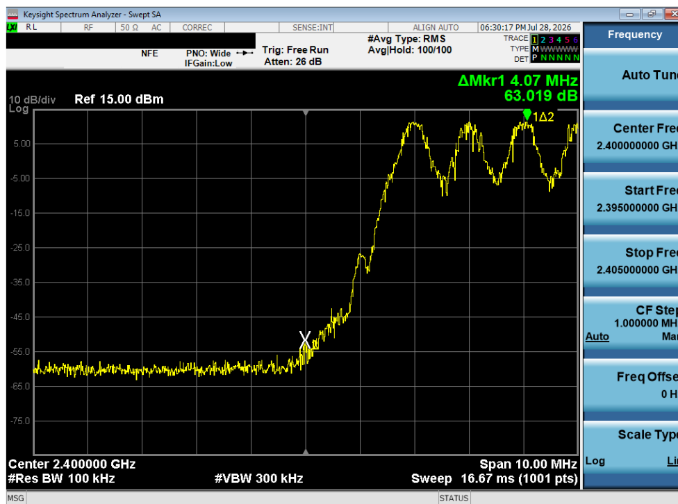
Plot 7-30. Band Edge Plot (Bluetooth with Hopping Enabled, 1 Mbps)
