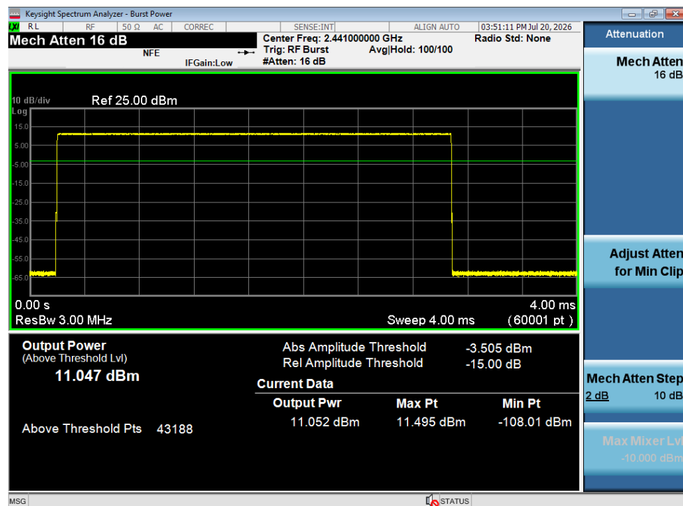
Plot 7-20. Average Conducted Power (1Mbps – Ch. 39)
