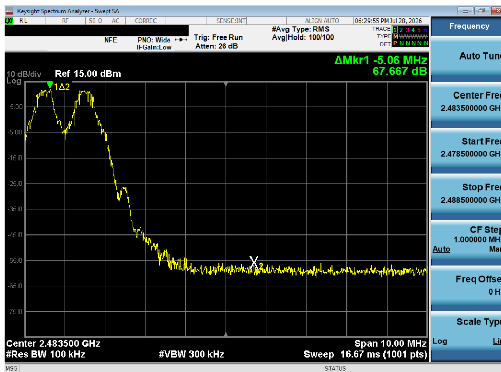
Plot 7-31. Band Edge Plot (Bluetooth with Hopping Enabled, 1 Mbps)
