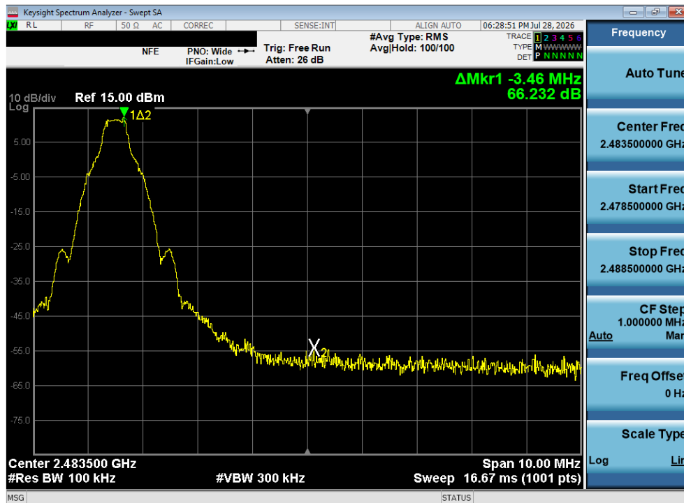
Plot 7-29. Band Edge Plot (Bluetooth with Hopping Disabled, 1 Mbps – Ch. 78)
