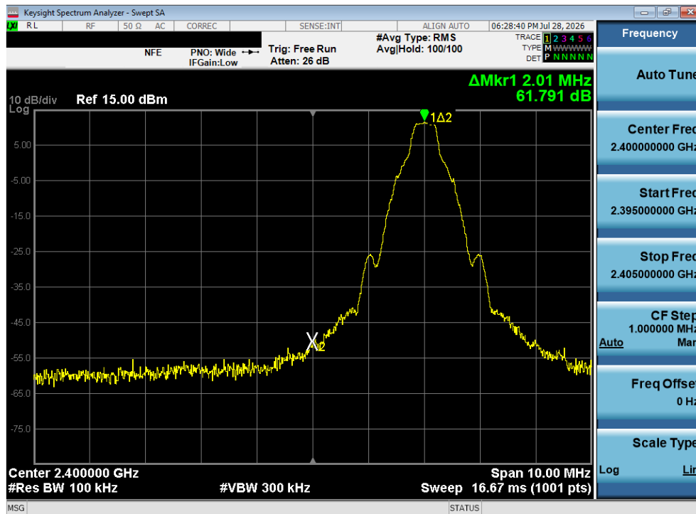
Plot 7-28. Band Edge Plot (Bluetooth with Hopping Disabled, 1 Mbps – Ch. 0)
