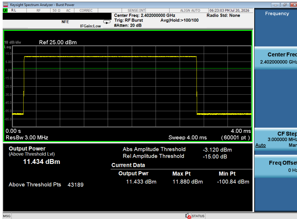
Plot 7-19. Average Conducted Power (1Mbps – Ch. 0)
