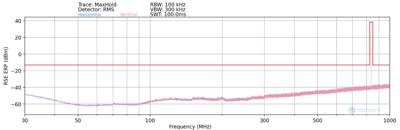
Plot 7-41. Radiated Spurious Plot (GPRS Cell)
