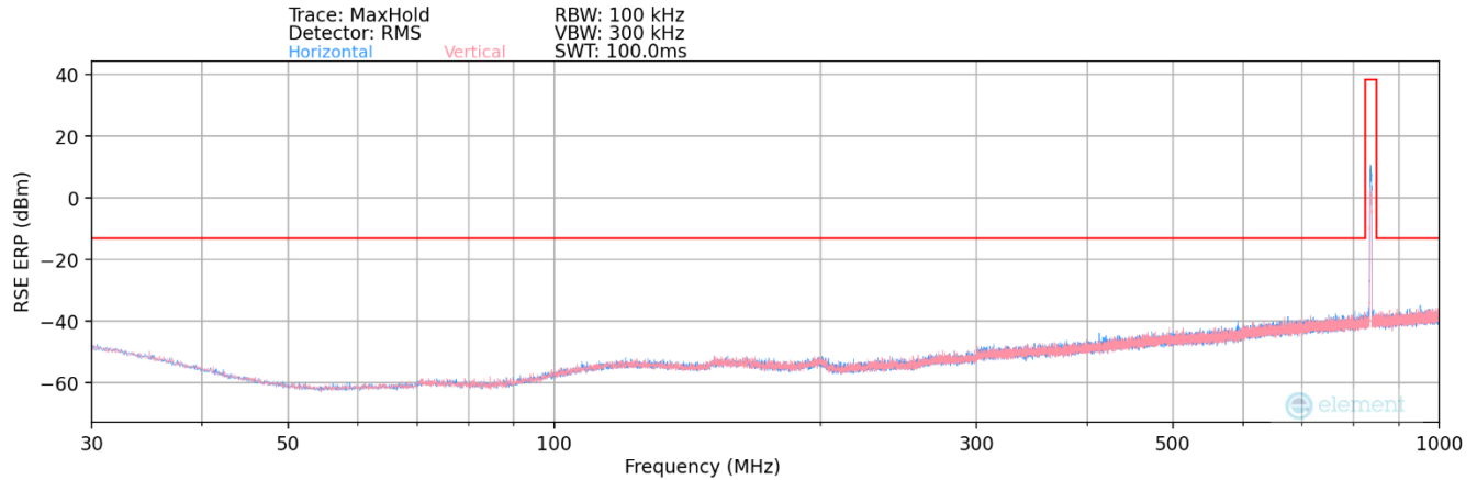
Plot 7-43. Radiated Spurious Plot (WCDMA Cell)
