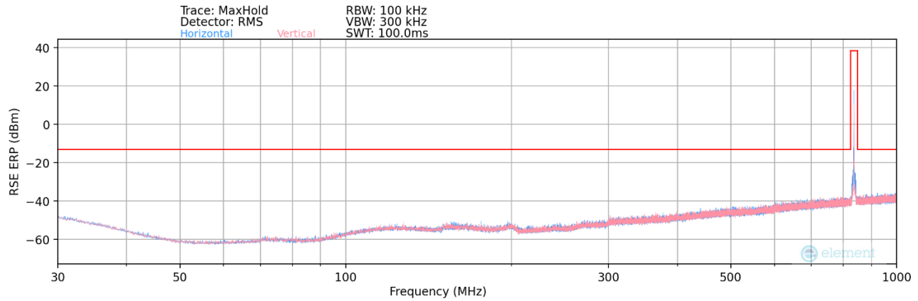
Plot 7-37. Radiated Spurious Plot (LTE Band 26)
