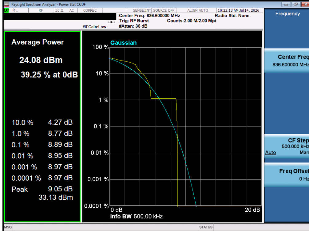
Plot 7-35. Peak-Average Ratio Plot (GPRS Edge Cell – Ch. 190)
