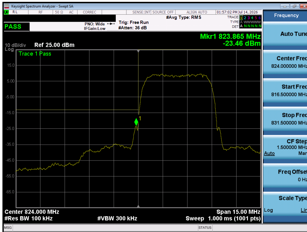
Plot 7-27. Lower Band Edge Plot (WCDMA Cell – Ch. 4132)
