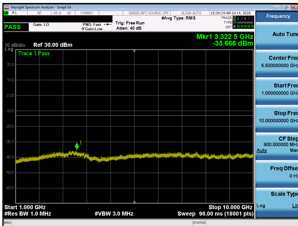
Plot 7-19. Conducted Spurious Plot (GPRS Cell Ch. 251)
