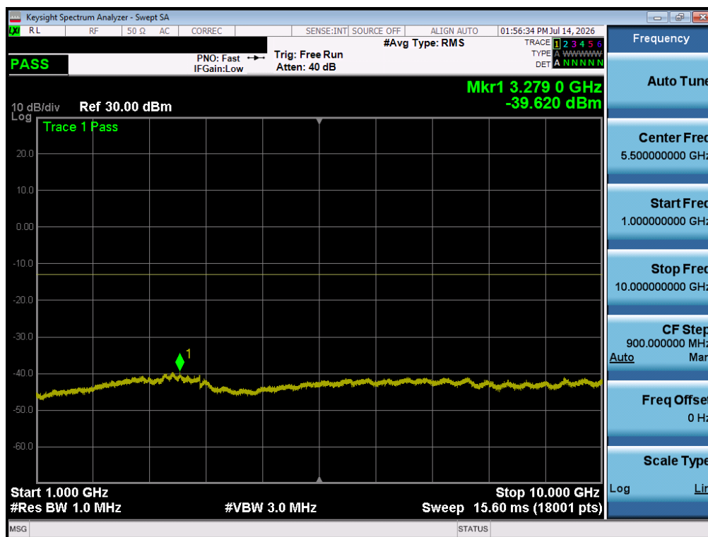
Plot 7-22. Conducted Spurious Plot (WCDMA Cell Ch. 4132)
