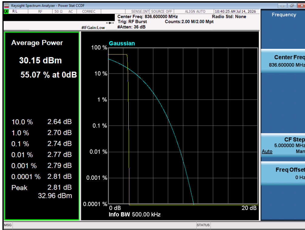
Plot 7-34. Peak-Average Ratio Plot (GPRS Cell – Ch. 190)
