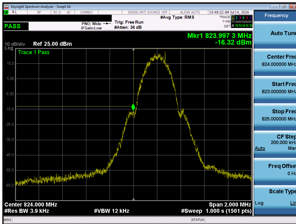
Plot 7-25. Lower Band Edge Plot (GPRS Cell – Ch. 128)
