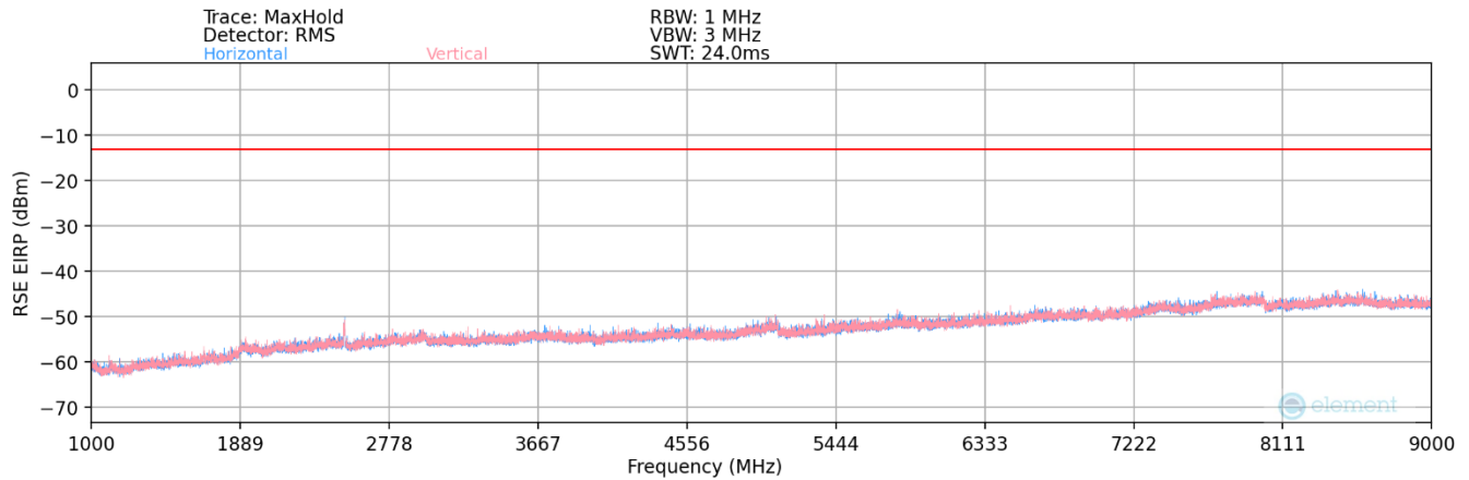
Plot 7-44. Radiated Spurious Plot (WCDMA Cell)
