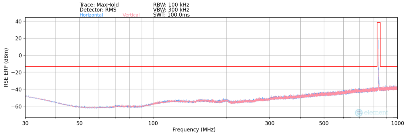
Plot 7-39. Radiated Spurious Plot (LTE Band 5)
