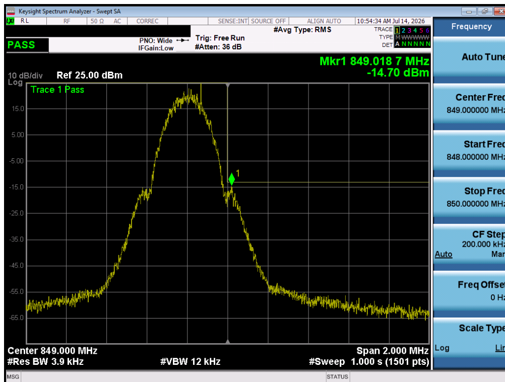
Plot 7-26. Upper Band Edge Plot (GPRS Cell – Ch. 251)
