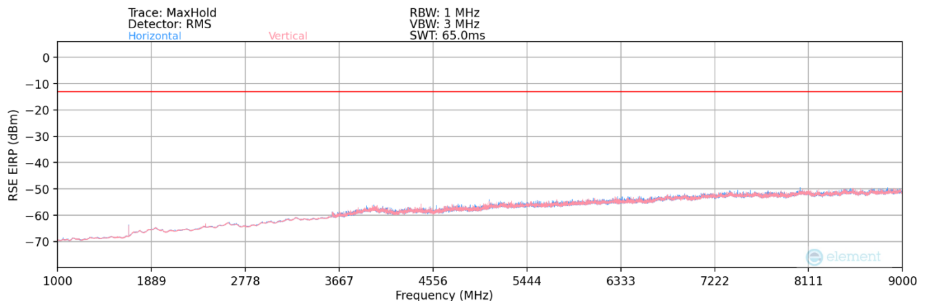
Plot 7-42. Radiated Spurious Plot (GPRS Cell)
