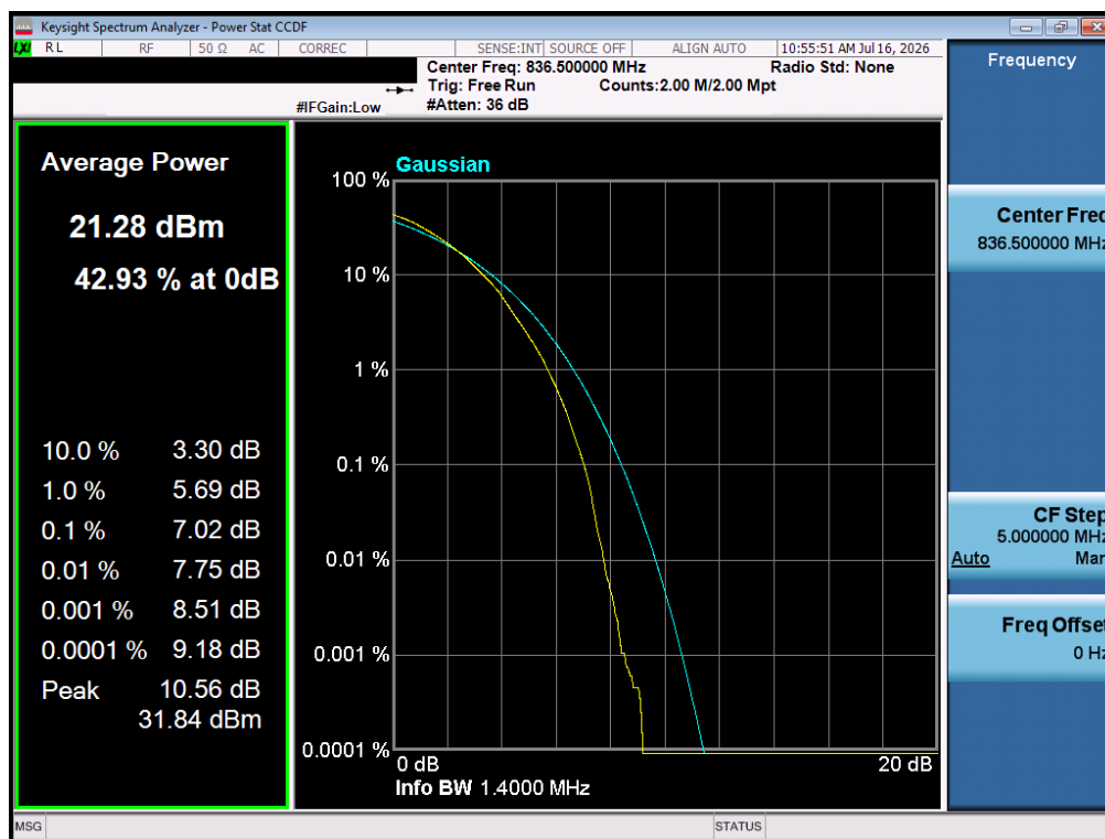
Plot 7-33. Peak-Average Ratio Plot (LTE Band 26/5 – 1.4MHz 64QAM – Full RB)
