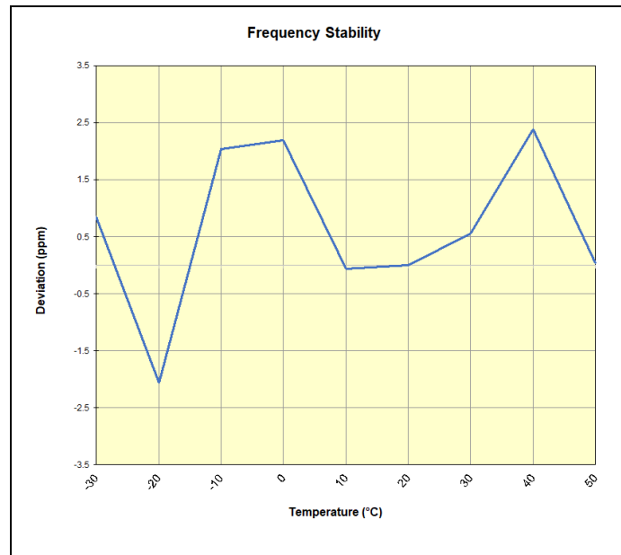
Plot 7-46. GSM/GPRS Cell Frequency Stability Chart
