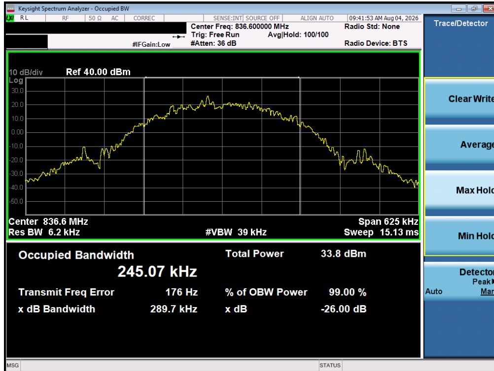
Plot 7-12. Occupied Bandwidth Plot (GPRS Edge Cell, Ch. 190)
