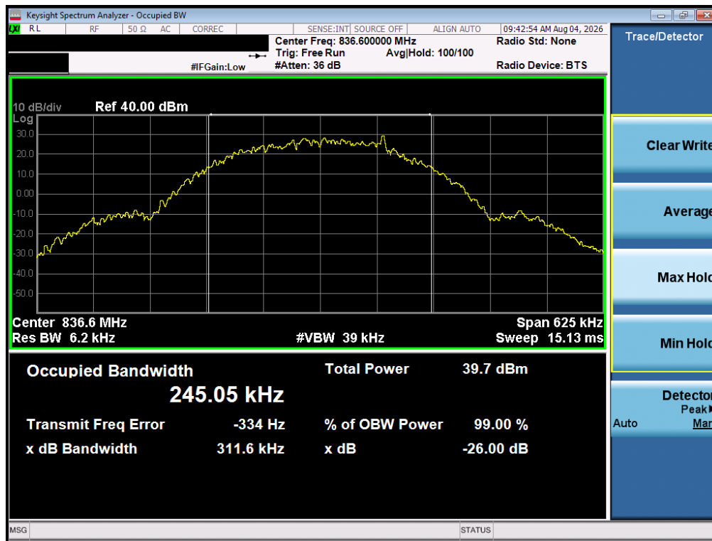
Plot 7-11. Occupied Bandwidth Plot (GPRS Cell, Ch. 190)
