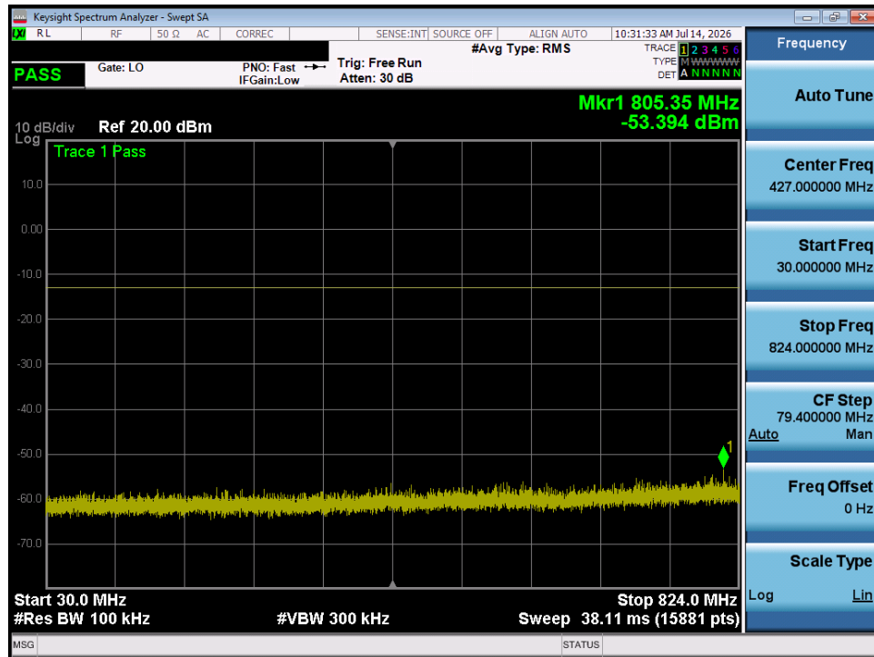
Plot 7-17. Conducted Spurious Plot (GPRS Cell Ch. 251)
