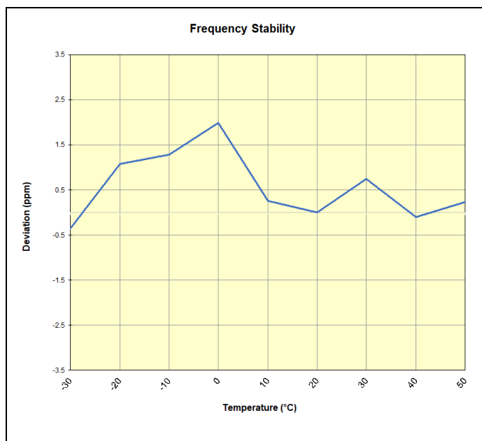
Plot 7-47. WCDMA Cell Frequency Stability Chart
