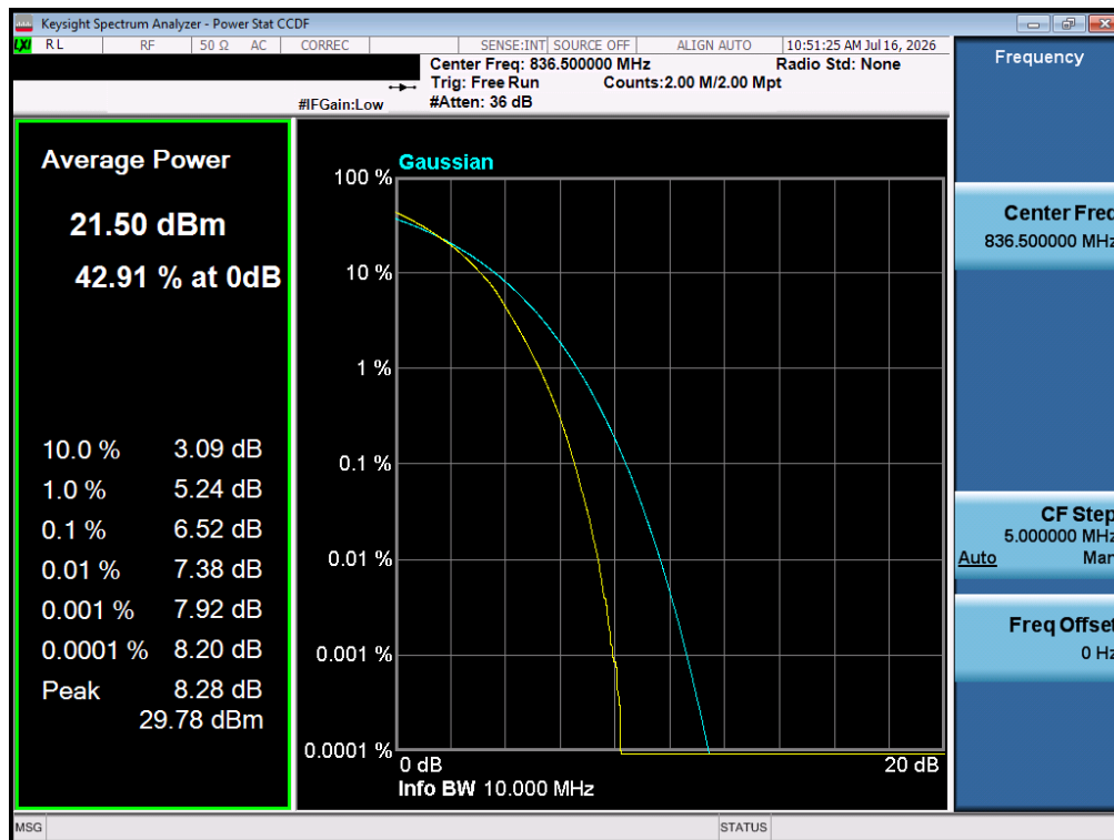
Plot 7-30. Peak-Average Ratio Plot (LTE Band 26/5 – 10MHz 64QAM – Full RB)
