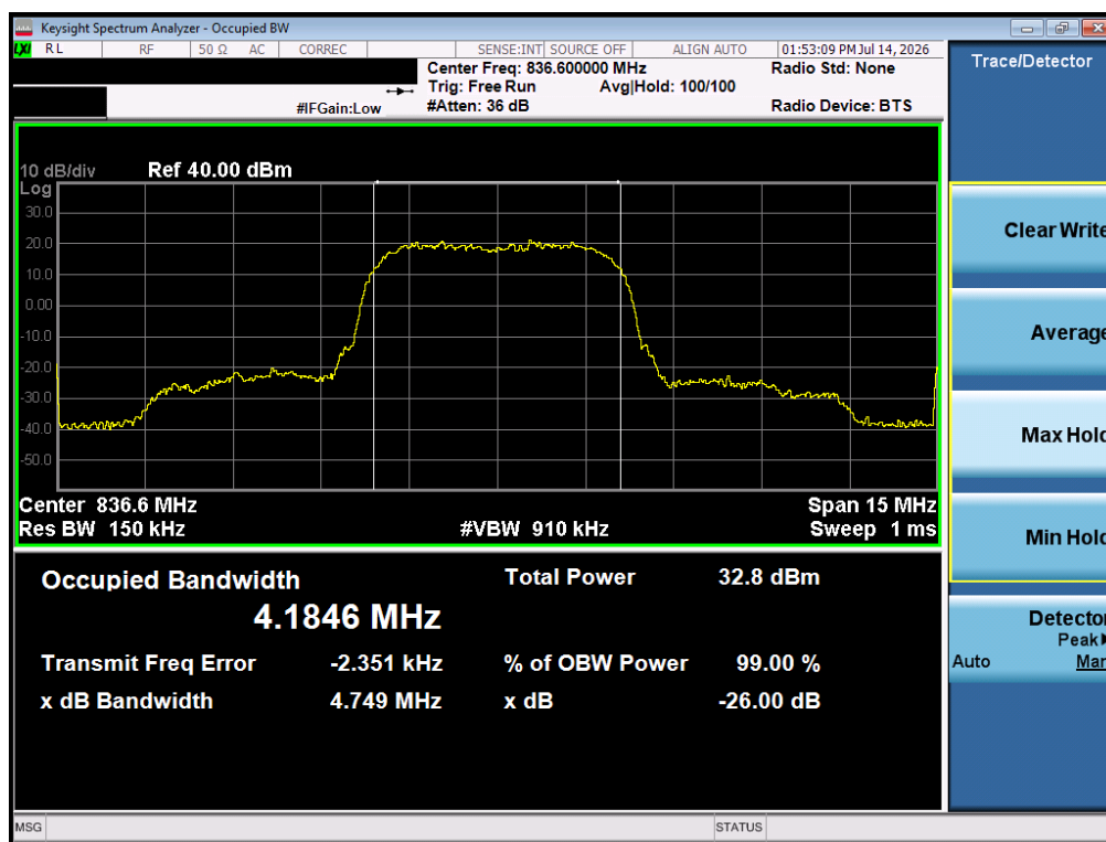
Plot 7-13. Occupied Bandwidth Plot (WCDMA Cell, Ch. 4183)
