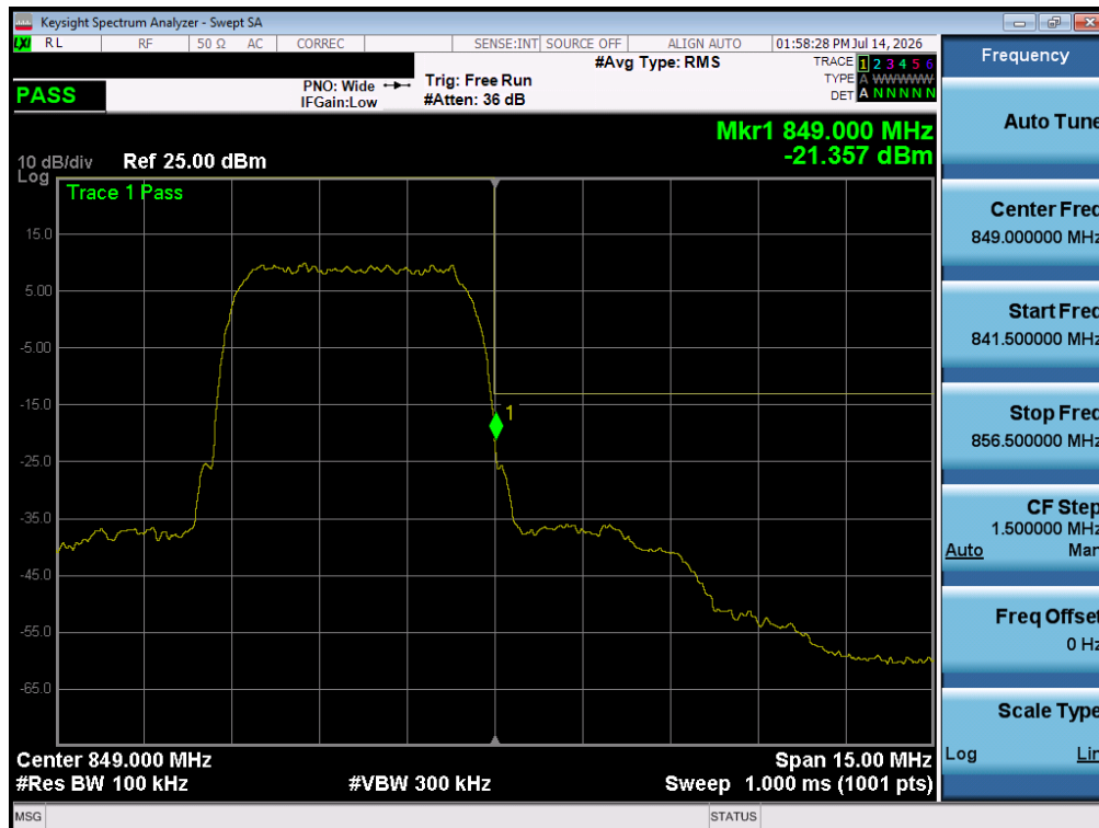
Plot 7-28. Upper Band Edge Plot (WCDMA Cell – Ch. 4233)
