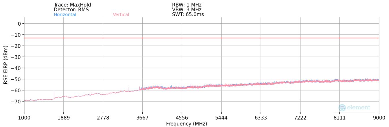
Plot 7-40. Radiated Spurious Plot (LTE Band 5)
