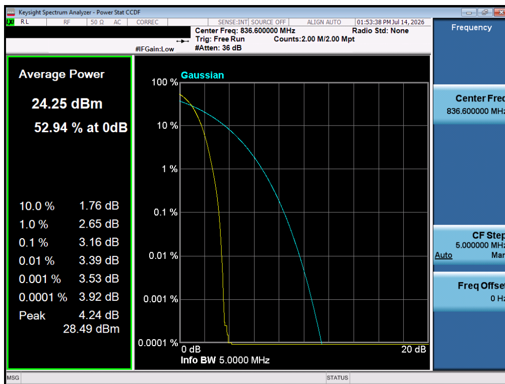
Plot 7-36. Peak-Average Ratio Plot (WCDMA Cell – Ch. 4183)
