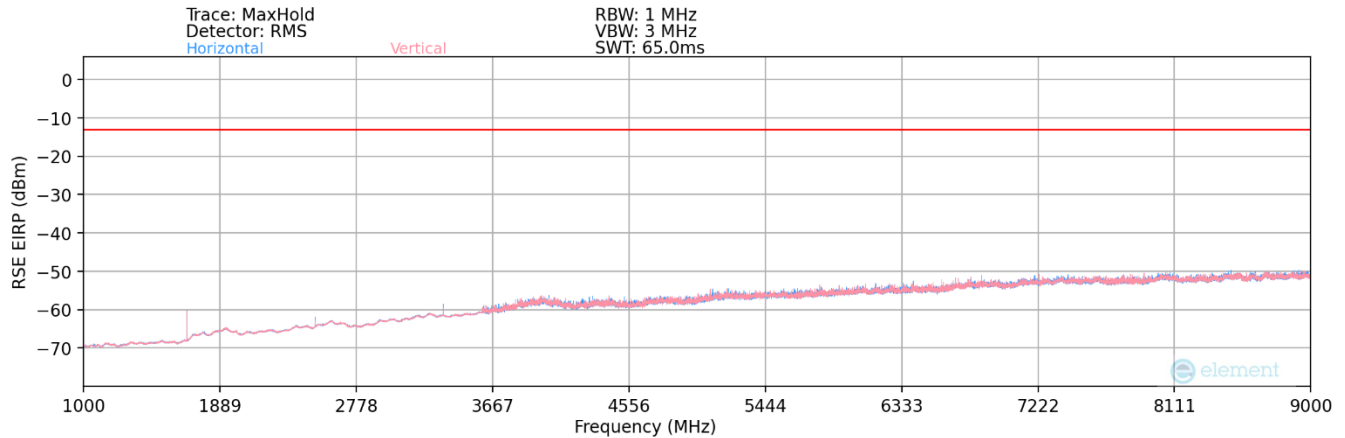
Plot 7-38. Radiated Spurious Plot (LTE Band 26)
