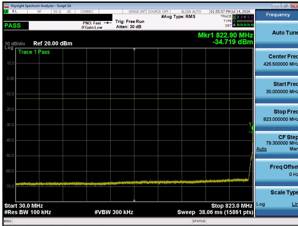
Plot 7-20. Conducted Spurious Plot (WCDMA Cell Ch. 4132)
