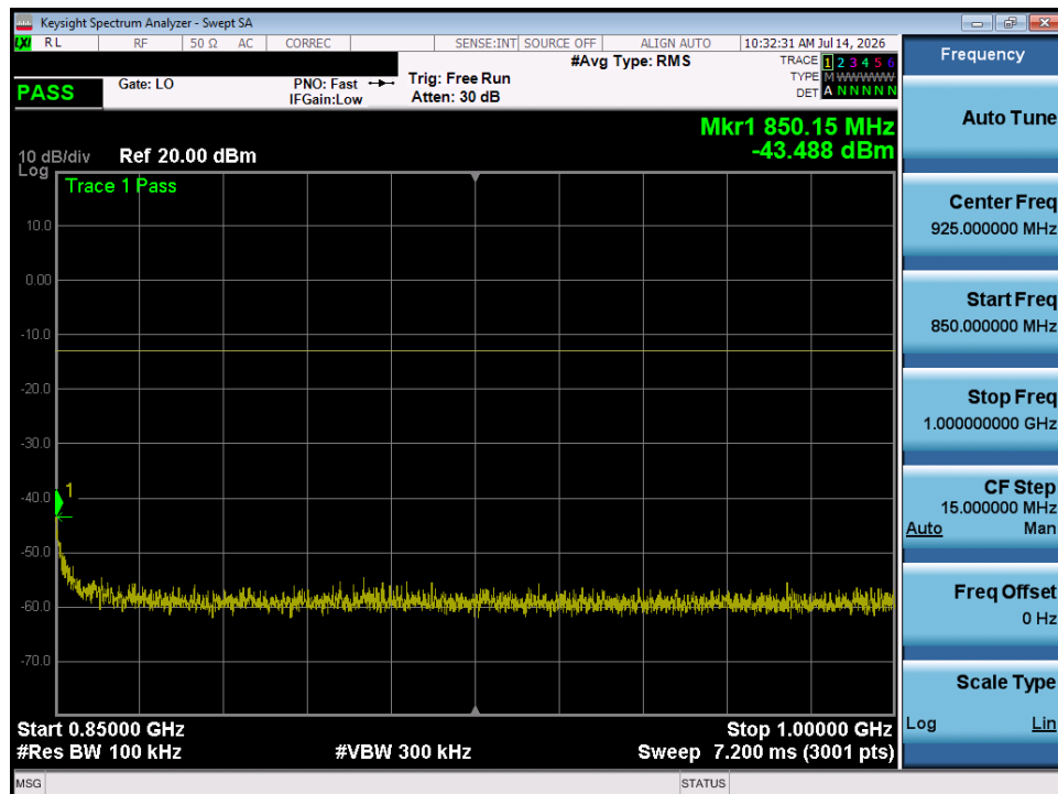
Plot 7-18. Conducted Spurious Plot (GPRS Cell Ch. 251)
