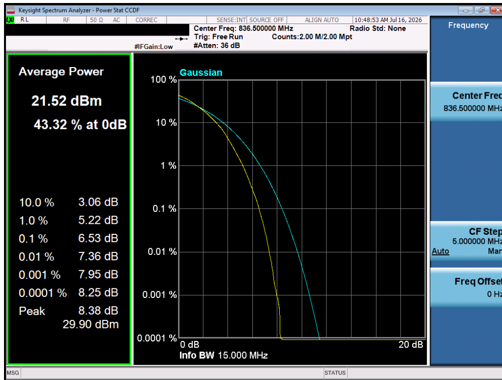
Plot 7-29. Peak-Average Ratio Plot (LTE Band 26 – 15MHz 64QAM – Full RB)
