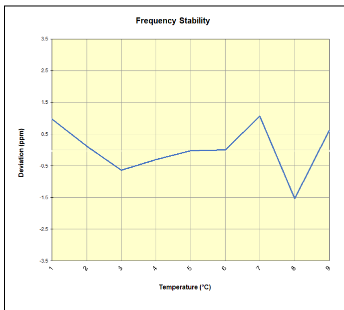
Plot 7-45. LTE Band 26/5 Frequency Stability Chart
