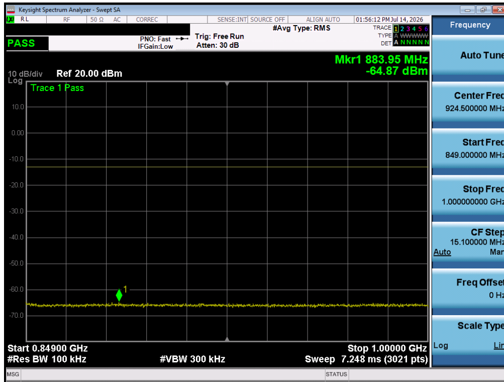
Plot 7-21. Conducted Spurious Plot (WCDMA Cell Ch. 4132)
