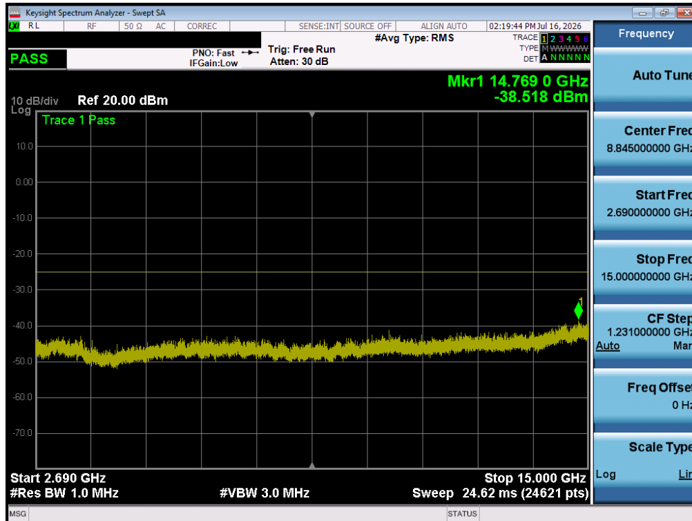
Plot 7-10. Conducted Spurious Plot (LTE Band 41 PC3 - 20MHz QPSK - 1 RB - Mid Channel)
