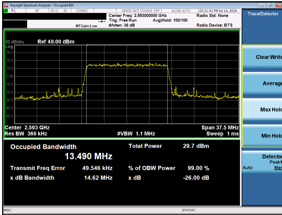
Plot 7-3. Occupied Bandwidth Plot (LTE Band 41 (PC3) - 15MHz QPSK - Full RB)
