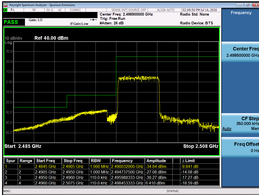
Plot 7-12. Lower Band Edge Plot (LTE Band 41 PC3 – 5MHz QPSK – Full RB)
