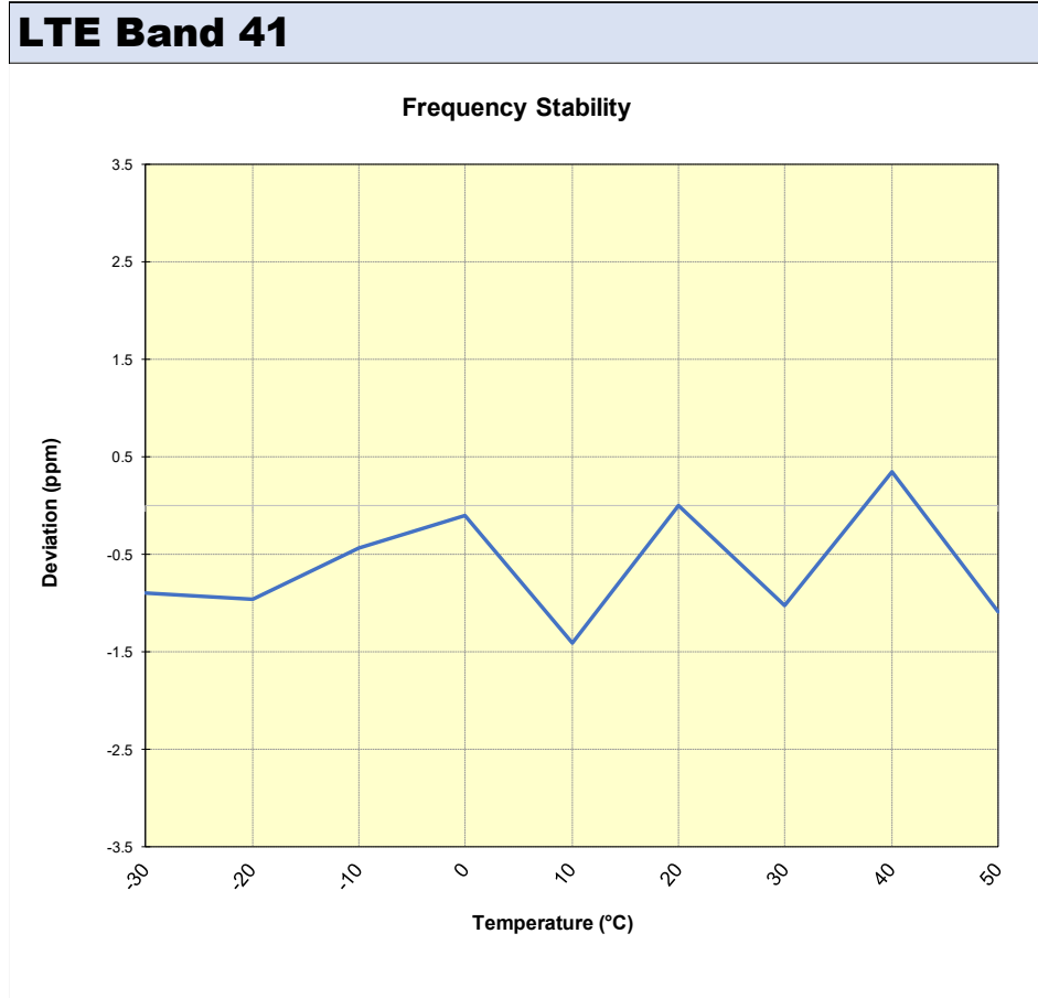
Plot 7-16. LTE Band 41 PC3 Frequency Stability Chart
