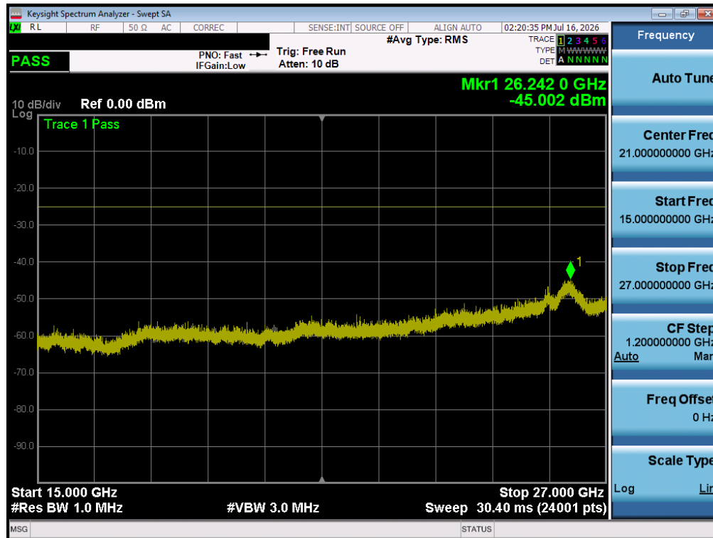
Plot 7-11. Conducted Spurious Plot (LTE Band 41 PC3 - 20MHz QPSK - 1 RB - Mid Channel)
