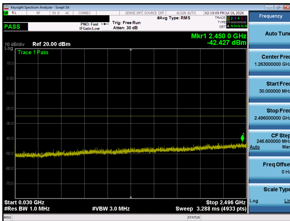
Plot 7-9. Conducted Spurious Plot (LTE Band 41 PC3 - 20MHz QPSK - 1 RB - Mid Channel)
