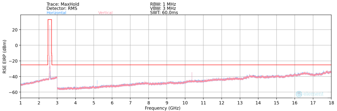
Plot 7-15. Radiated Spurious Plot (LTE Band 41 PC3)
