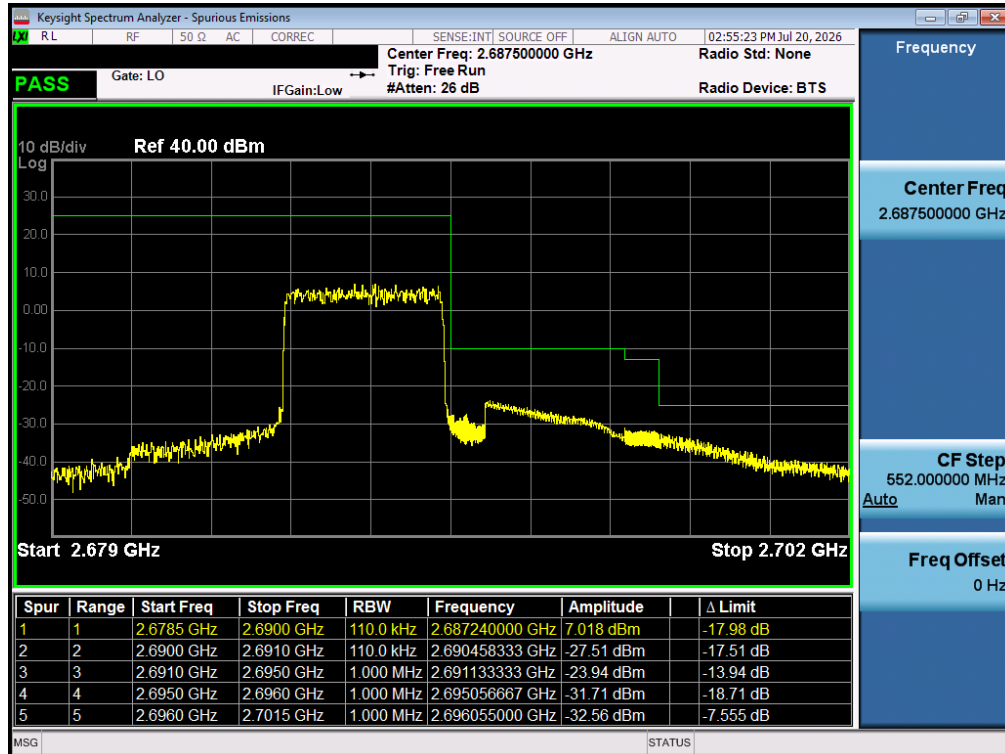
Plot 7-13. Upper Band Edge Plot (LTE Band 41 PC3 – 5MHz QPSK – Full RB)
