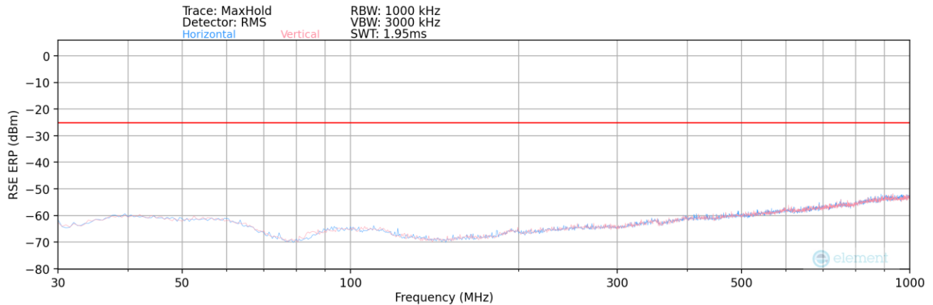
Plot 7-14. Radiated Spurious Plot (LTE Band 41 PC3)
