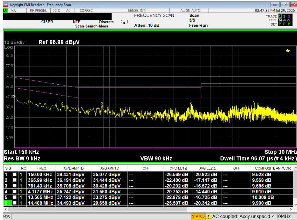
Plot 7-5. Line-Conducted Test Plot (L1)
