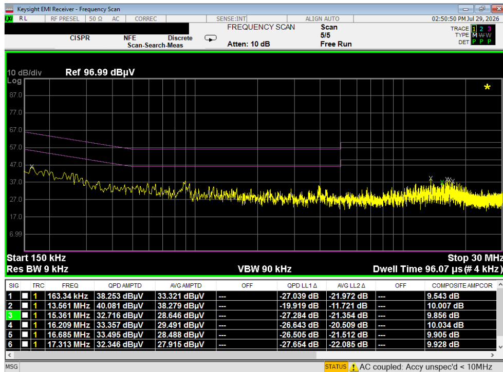
Plot 7-6. Line-Conducted Test Plot (N)
