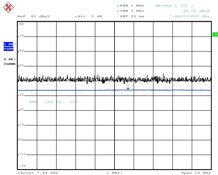
Radiated Spurious Emissions plot – Average Reading (Ch.39 3rd Harmonic_X-H)
