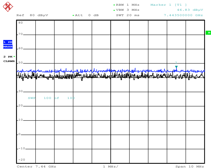
Radiated Spurious Emissions plot – Peak Reading (Ch.39 3rd Harmonic_X-H)
