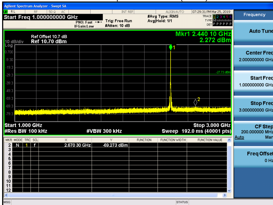
Conducted Spurious Emission (CH 19)
