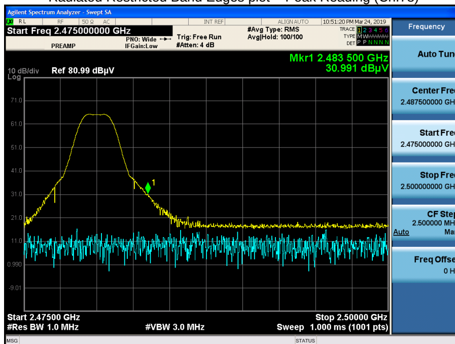
Radiated Restricted Band Edges plot – Peak Reading (Ch.78)
