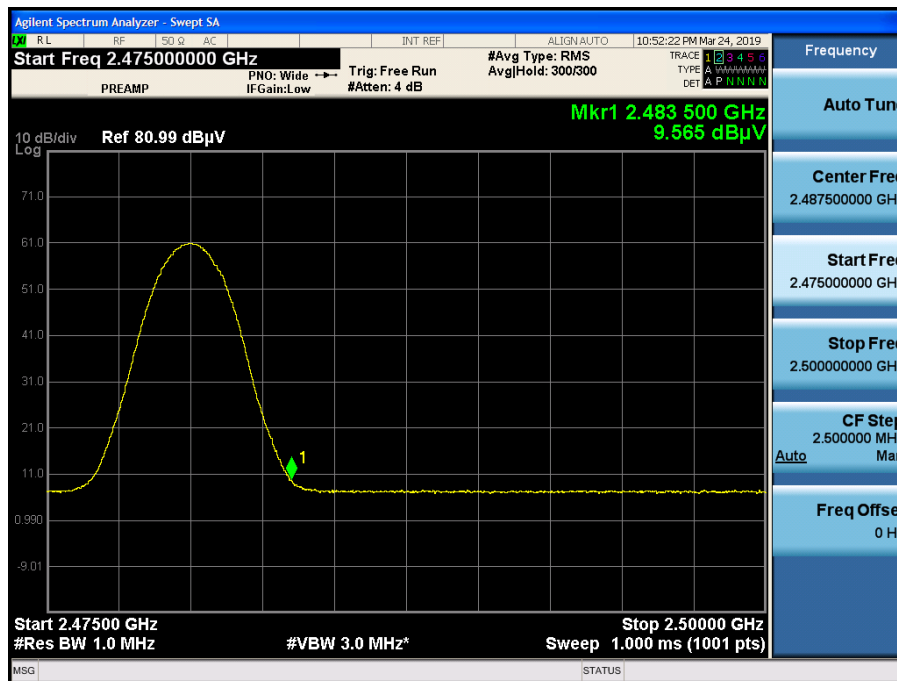
Radiated Restricted Band Edges plot – Average Reading (Ch.78)
