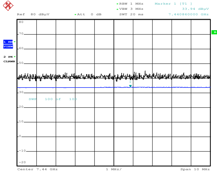
Radiated Spurious Emissions plot – Average Reading (Ch.39 3rd Harmonic_X-H)
