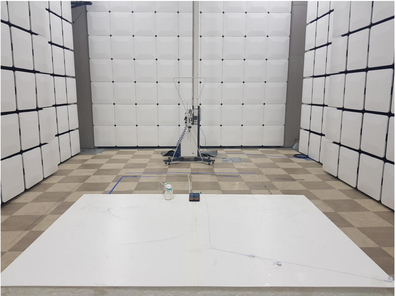
RE_30M~1GHz_Front
